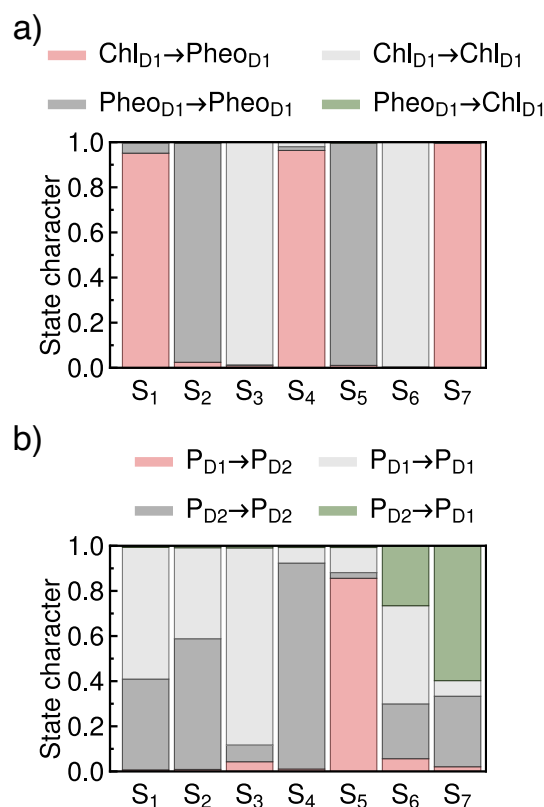
Figure 3: Characterization of the excited states via their charge transfer numbers. a) Excited state characters of \text{Chl}_{\text{D1}}\text{Pheo}_{\text{D1}} pair at the FC geometry. b) Excited state characters of \text{P}_{\text{D1}}\text{P}_{\text{D2}} pair at the FC geometry.
