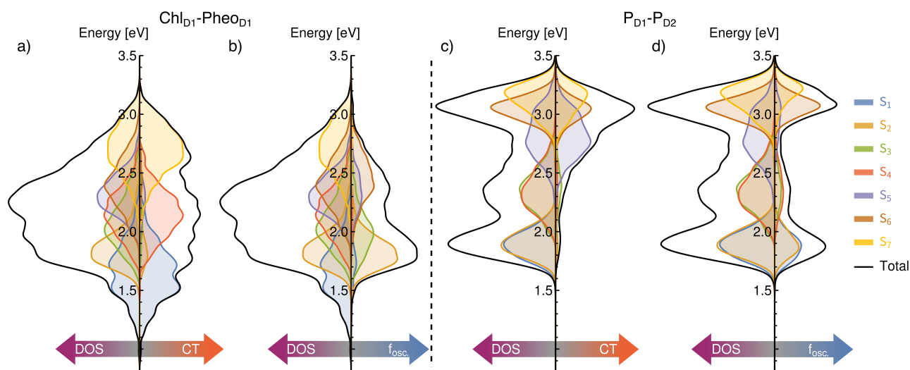
Figure 6: Spectral characteristics of \text{Chl}_{\text{D1}}\text{Phe}_{\text{OD1}} and \text{P}_{\text{D1}}\text{P}_{\text{D2}} pairs. a) DOS and density of the \text{Chl}_{\text{D1}} \rightarrow \text{Phe}_{\text{OD1}} CT character. b) DOS and absorption spectrum in \text{Chl}_{\text{D1}}\text{Phe}_{\text{OD1}} pair. c) DOS and density of \text{P}_{\text{D1}} \rightarrow \text{P}_{\text{D2}} and \text{P}_{\text{D2}} \rightarrow \text{P}_{\text{D1}} CT characters. d) DOS and absorption spectrum in \text{P}_{\text{D1}}\text{P}_{\text{D2}} pair.
