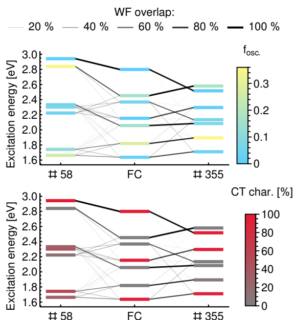
Figure 4: Illustration of mixing and reordering of excited states using wavefunction overlaps with the Franck–Condon geometry as a reference for the \text{Chl}_{D1}\text{Phe}_{D1} pair. Geometry #58 represents an example of the mixing of states, while geometry #355 illustrates reordering. States are coloured by the oscillator strength from the ground state in the upper panel and by the portion of the \text{Chl}_{D1} \rightarrow \text{Phe}_{D1} CT character in the lower panel.
