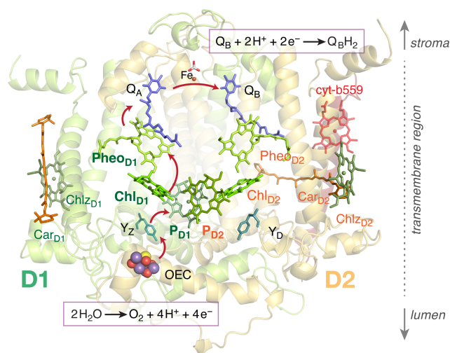
Figure 1: The chlorophyll and pheophytin pigments comprising the reaction center of PSII. Important additional cofactors of PSII are also indicated. The primary charge separation occurs among pigments of the D1 protein, initiated either within the \text{Chl}_{\text{D1}}\text{Pheo}_{\text{D1}} or the \text{P}_{\text{D1}}\text{P}_{\text{D2}} pairs, following direct light absorption or excitation energy transfer from internal and external light harvesting complexes. The arrows depict the flow of electrons from the donor side (water oxidation) to the acceptor side (plastoquinone reduction).
