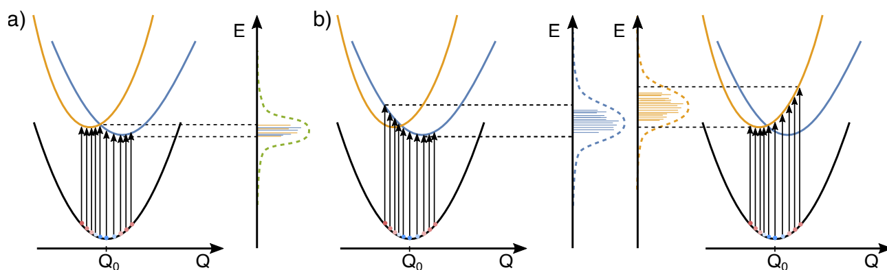
Figure 5: Schematic description of the presented methodology for analyzing a nuclear ensemble in a unified basis of electronic states. a) The electronic states are ordered by their energies and the spectral feature of a first excited state is a mix of two state characters. b) The electronic states are ordered by their character and the spectral features of both excited states are composed of the states that preserve character.
