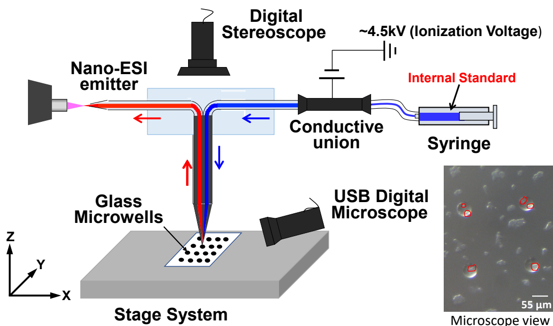
Figure 3: Quantitative Single-probe SCMS experimental setup with individual cells and microwells on glass chip shown in the microscopic image. [Reproduced from Pan, N.; Standke, S. J.; Kothapalli, N. R.; Sun, M.; Bensen, R. C.; Burgett, A. W. G.; Yang, Z. Quantification of Drug Molecules in Live Single Cells Using the Single-Probe Mass Spectrometry Technique. Anal. Chem. 2019, 91, 14, 9018–9024. Copyright © 2019, American Chemical Society]
