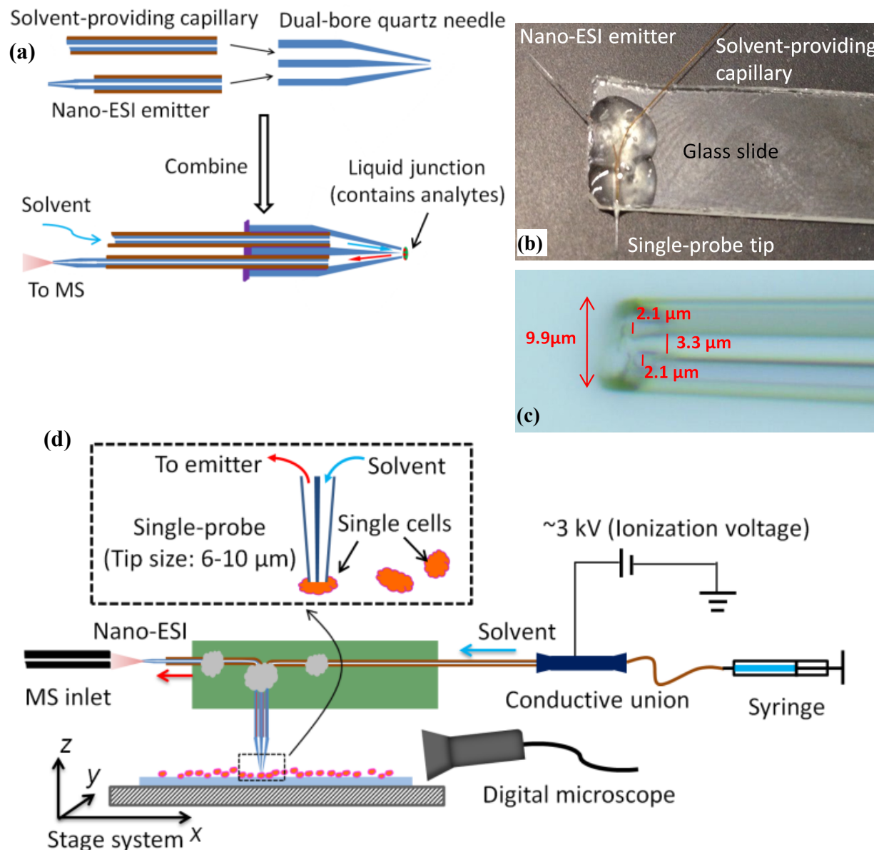
Figure 1. Single-probe SCMS. (a) Fabrication steps of the Single-probe; (b) photograph of a Single-probe; (c) zoomed-in view (40 \times magnification) of the Single-probe tip with measurements from a calibrated digital microscope; (d) schematic of the Single-probe setup for SCMS analysis. [Reproduced with the permission Pan, N.; Rao, W.; Kothapalli, N. R.; Liu, R.; Burgett, A. W.; Yang, Z. The single-probe: a miniaturized multifunctional device for single cell mass spectrometry analysis. Analytical Chemistry 2014, 86.19, 9376-9380. (ref 21) Copyright © 2014, American Chemical Society]
