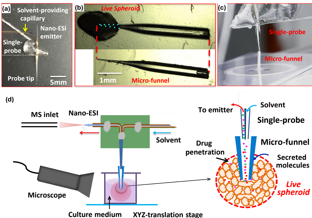
Figure 10: Combined the Micro-funnel and Single-probe technique for MS analysis of extracellular compounds in live spheroids. (a) A photo of a Single-probe device. (b) A photo of a Micro-funnel before and after being implanted into a spheroid. (c) Coupled Micro-funnel and Single-probe device. (d) Real-time MS analysis of extracellular compounds in a live spheroid using the coupled Micro-funnel and Single-probe device. [Reproduced from Sun, M.; Tian, X.; Yang, Z. Microscale Mass Spectrometry Analysis of Extracellular Metabolites in Live Multicellular Tumor Spheroids . Analytical Chemistry 2017, 89, 17, 9069–9076. (ref 28) Copyright © 2017, American Chemical Society]
