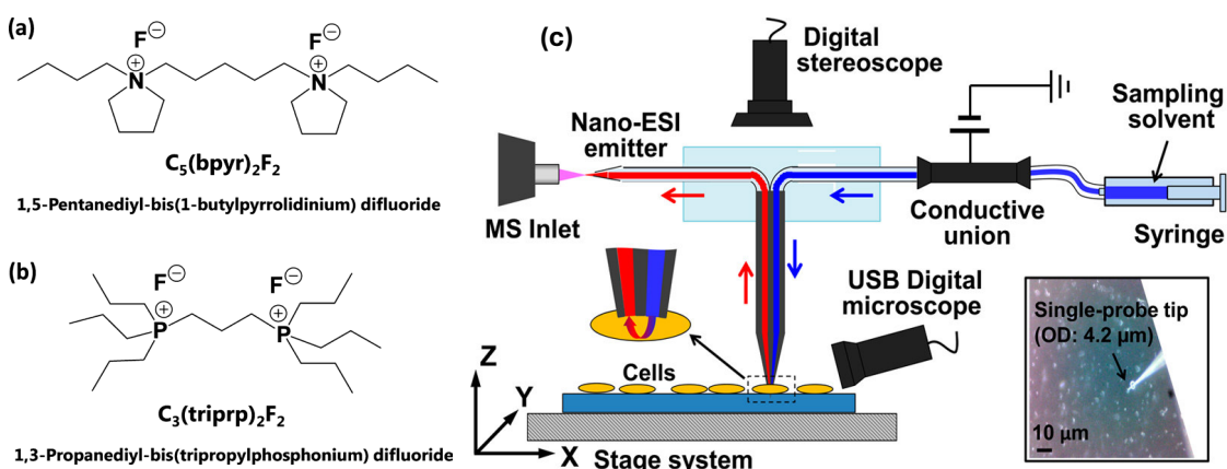
Figure 5: Molecular structures of dicationic compounds (a) C_5(\text{bpyr})_2F_2 and (b) C_3(\text{triprp})_2F_2 . (c) Schematic drawing of the single-probe SCMS setup. The inset indicates the insertion of a single-probe tip into a cell. [Reproduced Pan, N.; Rao, W.; Standke, S. J.; Yang, Z. Using Dicationic Ion-Pairing Compounds To Enhance the Single Cell Mass Spectrometry Analysis Using the Single-Probe: A Microscale Sampling and Ionization Device. Anal. Chem. 2016, 88, 13, 6812–6819. (ref 33) Copyright © 2016, American Chemical Society]
