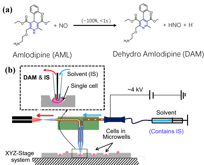
Figure 6: Quantification of NO in single cells. (a) Reaction of AML and NO producing DAM. (b) Using the quantitative Single-probe SCMS cell setup to quantify NO in single cells. A Glass chip containing microwells is used for cell culture and the SCMS experiment. [Reproduced from Lan, Y.; Chen, X.; Yang, Z. Quantification of Nitric Oxide in Single Cells Using the Single-Probe Mass Spectrometry Technique. Anal. Chem. 2023, 95, 51, 18871–18879. (ref 36) Copyright © 2023, American Chemical Society]
