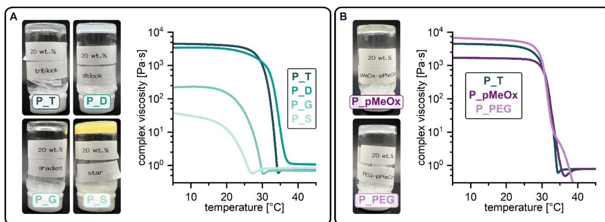
Figure 4: Screening for the gel-sol transition of pPheOzi-based copolymers. Images show self-supporting gels formed by 20 wt.-% aqueous solutions of pPheOzi-copolymer variants (A: P_T, P_D, P_G and P_S; B: P_pMeOx and P_PEG) after incubation at 5 °C. Dissolution of the gels is followed by temperature-dependent rheology measurements conducted at 1.0% strain and an angular frequency of 10 rad/s using an increment rate of 0.5 °C/min. Liquefaction of the gels is indicated by drastic drop in complex viscosity.
