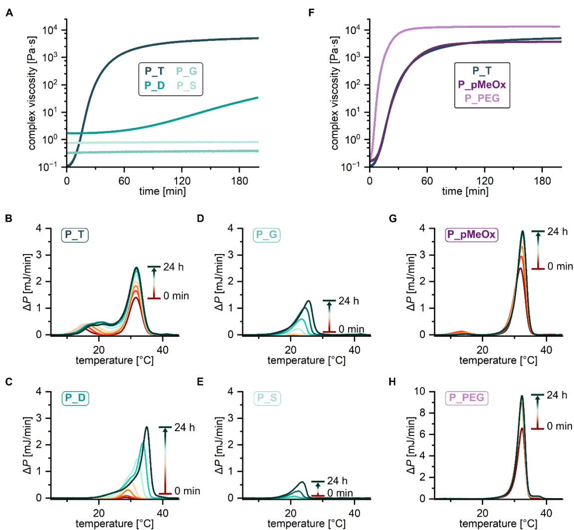
Figure 6: Kinetics of the sphere-to-worm transition-based thermogelation. A-F Time-dependent rheology measurements of liquid 20 wt.% aqueous solutions of P T , P D , P G and P S (A) as well as P pMeOx and P PEG (F) measured at 5 °C, 1.0% strain and an angular frequency of 10 rad/s. Onset of gelation is indicated by increase in complex viscosity. B-E+G+H μDSC thermograms of aqueous solutions of P T (B), P D (C), P G (D), P S (E), P pMeOx (G) and P PEG (H) incubated at 2 °C in the measurement system for different lengths of time (0 min, 10 min, 30 min, 1 hour, 3 hours, 6 hours, 12 hours, 24 hours).
