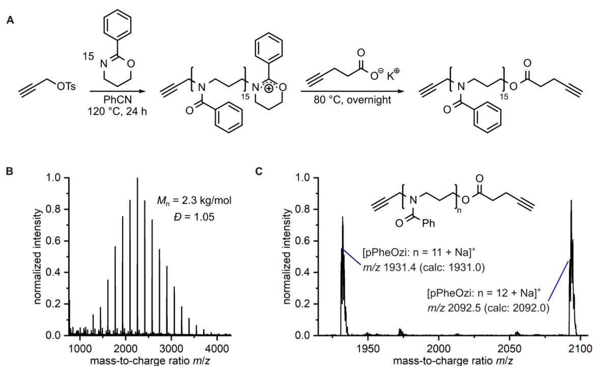
Figure 2: Successful synthesis of pPheOzi-dialkyne. A Synthetic pathway of pPheOzi-dialkyne by CROP of PheOzi using propargyl tosylate as initiator and potassium 4-pentynoate as terminating reagent. B MALDI-ToF mass spectrum of the purified pPheOzi-dialkyne recorded in reflector mode. The spectrum was obtained using DCTB as matrix and NaTFA as ionization agent. C Spectral expansion of the MALDI-ToF mass spectrum shown in B revealing essentially a single species for each DP of pPheOzi-dialkyne that is in accordance with the targeted polymer structure.
