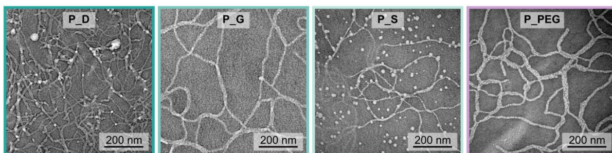
Figure 5: Presence of worm-like aggregates. Negative stain TEM images obtained of aqueous solutions of P_D , P_G , P_S and P_PEG after incubation at 5 °C revealing the presence of worm-like aggregates.
