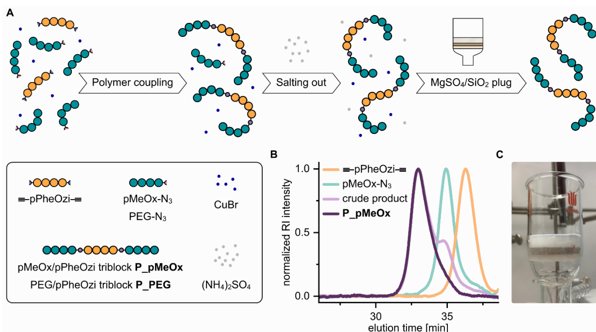
Figure 3: Coupling protocol for pPheOzi-based ABA triblocks. A Schematic representation of the polymer coupling strategy. The coupling reaction involves the pPheOzi dialkyne, an excess of hydrophilic azide-functionalized hydrophilic polymer (pMeOx-N 3 or PEG-N 3 , respectively) and the catalyst CuBr. Successfully coupled triblocks are separated from remaining homopolymer by selective precipitation through addition of (NH 4 ) 2 SO 4 . After dialysis, residual salts are removed by filtration of the polymer through a MgSO 4 /SiO 2 plug. B Size exclusion chromatography elugrams of the P_pMeOx synthesis. Shown are the elugrams of the starting materials pMeOx-N 3 and pPheOzi-dialkyne, the unpurified coupling product containing pMeOx/pPheOzi triblock and pMeOx-N 3 impurity, and the purified product P_pMeOx. C MgSO 4 /SiO 2 plug after filtration of the pMeOx/pPheOzi triblock P_pMeOx showing a fine blue layer on top, indicating separation of copper salts.
