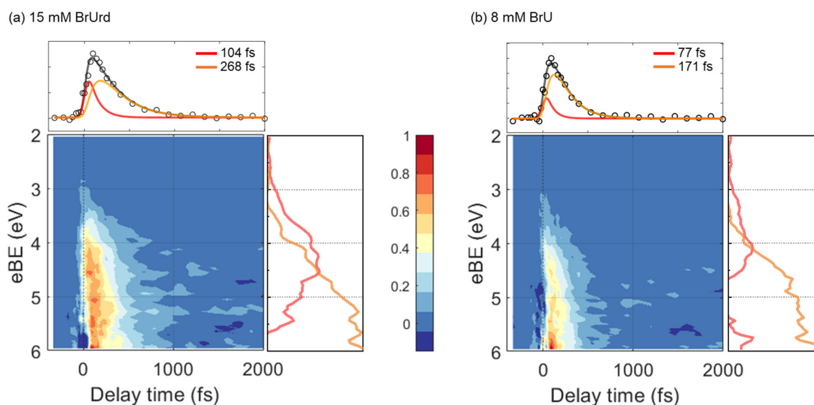
Fig. 4 LAPE-subtracted time-resolved photoelectron spectra and associated global lifetime analysis (GLA) results for (a) 15 mM BrUrd and (b) 8 mM BrU aqueous solution. In the upper panel, temporal lineout of GLA results are displayed, while the right panel shows evolution-associated spectra (EAS) obtained from GLA. Fast time components resulting from GLA are labeled in red, while slow time components are labeled in blue. The integrated total temporal behavior of the GLA results is depicted by the black solid line in the temporal lineout.
