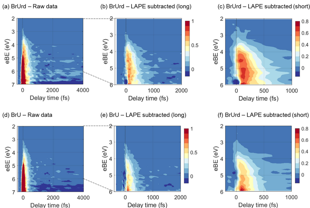
Fig. 3 Contour plots of time-resolved photoelectron spectra for (a-c) 15 mM BrUrUd and (d-f) 8 mM BrU in liquid flat jets. The 2 – 6 eV region of the raw photoelectron spectra (a and c) was processed by subtracting the laser-assisted photoelectric effect (LAPE) at zero-time delay obtained in a 25 mM NaCl solution, resulting in LAPE-subtracted spectra with long (b and e) and short (c and f) temporal windows. The depletion features emerging from 6.5-7 eV corresponds to the UV-pump-induced population depletion of the target molecule ground state. 3 point spectral and temporal smoothing is applied to the short temporal window plots in order to clearly show the spectral shifts. The color bar is normalized based on the LAPE subtracted data. LAPE-subtracted spectra out to 4 ps are shown in Fig. S5.
