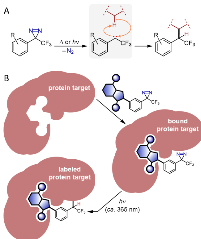
Fig. 1 Overview of diazirine reactivity and utility in chemical biology. A: Photochemical or thermal activation of diazirine reagents reveals reactive carbenes that can engage in X–H insertions to nearby substrate molecules. B: Photoaffinity labelling of target proteins with diazirine-enabled small molecules allows for identification of macromolecular binding partners.
