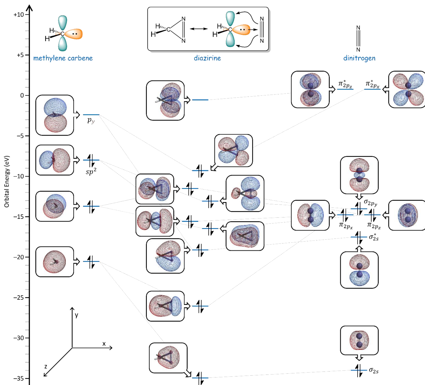
Fig. 11 Calculated frontier molecular orbitals (M06-2X/6-311+G(2df,2p)) for the parent diazirine molecule ( \text{H}_2\text{CN}_2 ), and correlations to the calculated orbitals of methylene carbene and dinitrogen.
