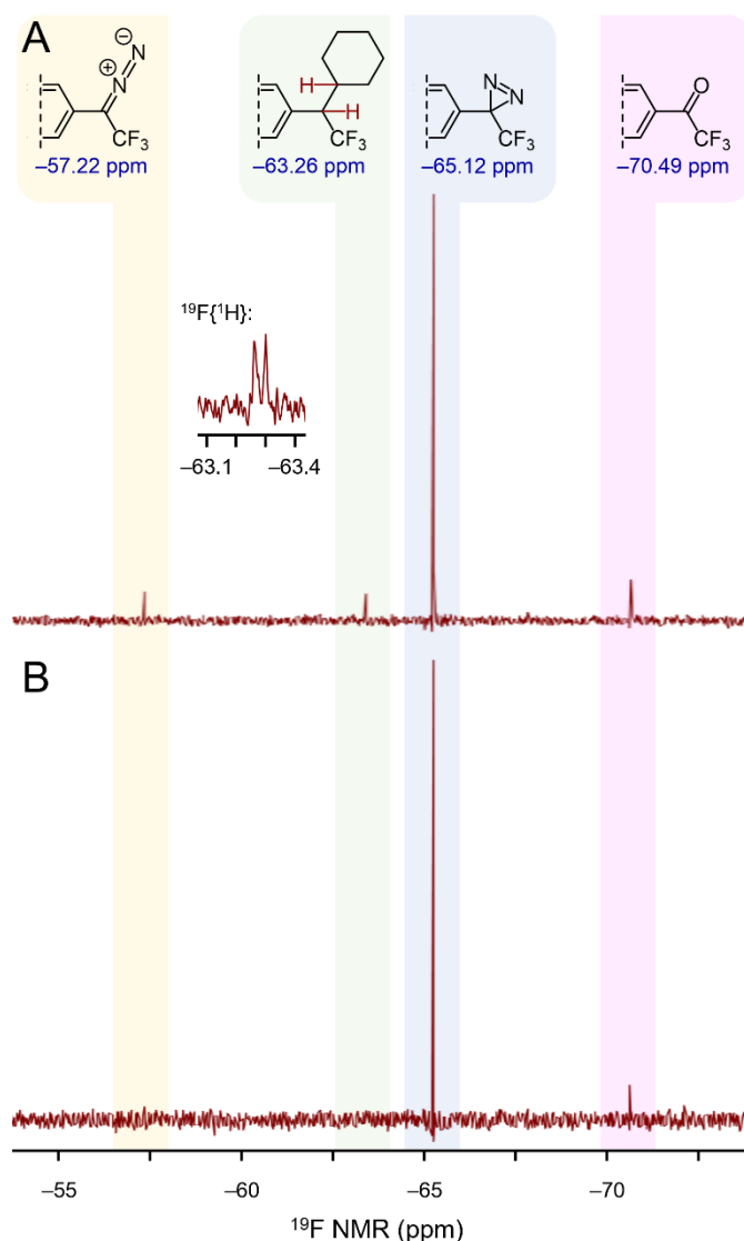
Fig. 10 ^{19}\text{F} NMR spectra illustrating the activation of diazirine 1 using red light. A: NMR spectrum following irradiation of 1 in cyclohexane with 815 nm light. B: Control sample stored in an amber vial. The inset shows a ^1\text{H} -coupled ^{19}\text{F} NMR spectrum, which confirms the presence of cyclohexane adduct 7 .
