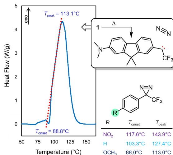
Fig. 6 DSC data for compound 1 , showing the diazirine activation exotherm. T_{\text{peak}} corresponds to the temperature at which the maximum heat flow is observed. T_{\text{onset}} is determined experimentally from extrapolation of the tangent of the upward slope observed in the DSC experiment (red dotted line), to the fitted baseline of the plot. Inset data taken from reference 17 show the decrease in activation temperature with increasing electron density in the aromatic ring.
