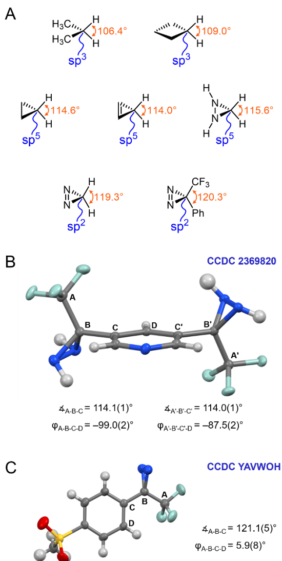
Fig. 5 Structural properties of diazirines and comparator molecules. A: Calculated bond angles (optimized using M06-2X/6-311+G(2df,2p)) for representative sp^3 and sp^5 alkanes and alkenes, together with calculated structures for diazirines and diaziridines. B: X-ray structure for 3,5-bis(3-(trifluoromethyl)diaziridin-3-yl)pyridine (CCDC 2369820). C: X-ray structure for 3-(4-(methylsulfonyl)phenyl)-3-(trifluoromethyl)-3H-diazirine (CCDC YAVWOH). 20 Thermal ellipsoids are shown at 50% probability.
