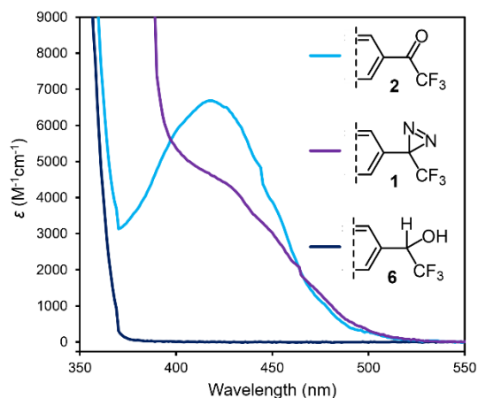
Fig. 8 UV/Vis spectrum for diazirine 1 , together with positive and negative control compounds 2 and 6 . All data were acquired using 0.05 mM samples in MeOH. Refer to the ESI for UV/Vis data for compounds 5 and 7 , and for UV/Vis spectra collected in cyclohexane.
