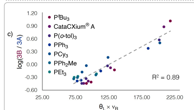
Figure 6 a) Aryne annulation conditions using a series of alkyl-substituted arynes and a variety of phosphine-ligated Buchwald-style palladacycle precatalysts. b) Charton analysis using each phosphine ligand individually. c) LFER model relating the regioselectivity of the aryne annulation to the product of the ligand's cone angle and the Charton value of the aryne substituent.
