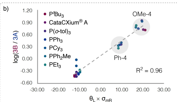
Figure 7 a) Aryne annulation conditions using a series of phosphine-ligated Buchwald-style palladacycle precatalysts and a variety of arynes with similarly sized but electronically differentiated substituents. b) LFER model relating the regioselectivity of the aryne annulation to the product of the ligand's cone angle and the \sigma_m parameter of the aryne substituent.
