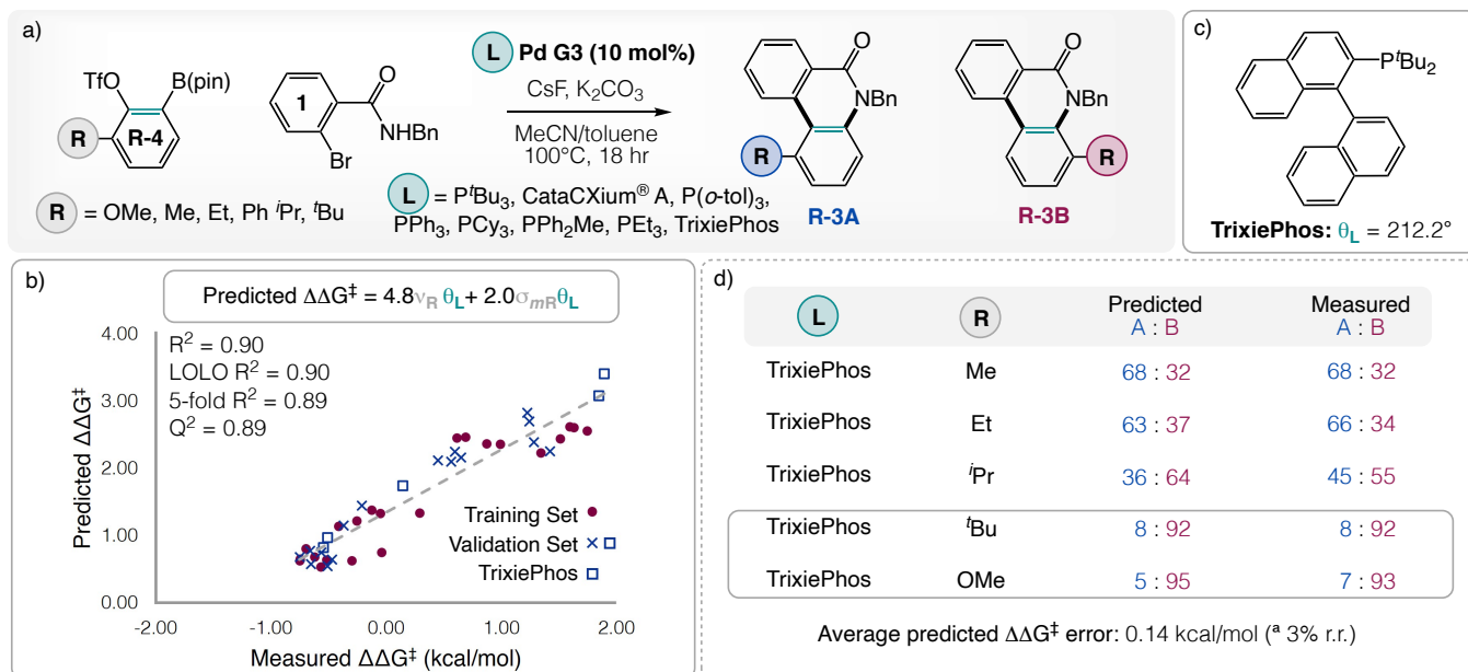
Figure 8 a) Aryne annulation conditions using a series of phosphine-ligated Buchwald-style palladacycle precatalysts and aryynes with substituents of various size and electronics. b) Multivariate linear regression correlating regioselectivity of the aryne annulation to a combination of ligand cone angle and the Hammett and Charton parameters associated with the aryne substituent. c) Experimental regioselectivity using TrixiePhos ligand vs. the regioselectivity predicted by multivariate linear regression.
