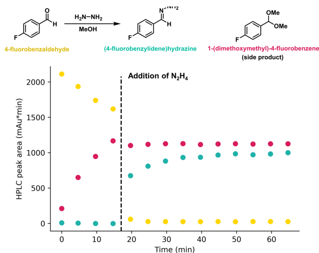
Fig. 7 Online HPLC monitoring of product formation with hydrazine hydrate addition at 17 min.
