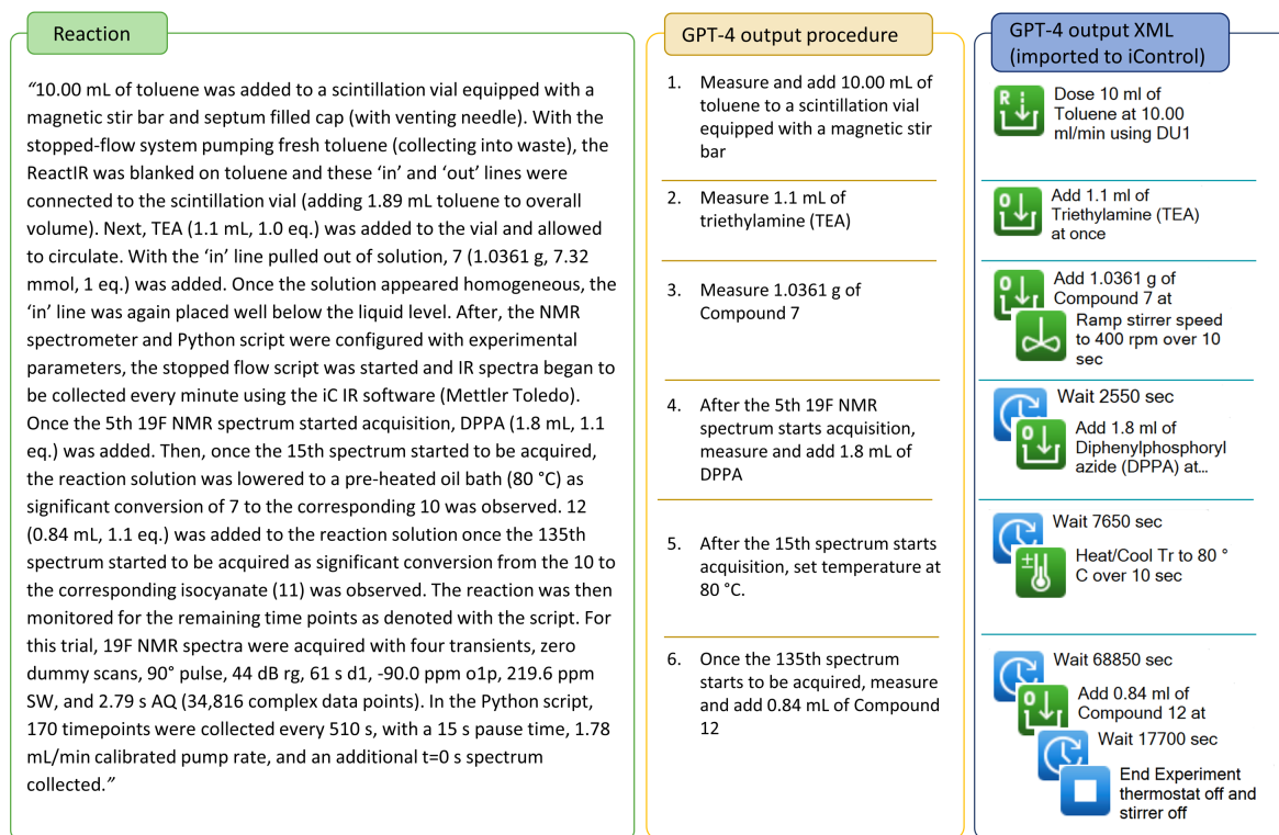
Fig. 6 Literature procedure of Curtius rearrangement, stepwise procedure and iControl operations generated by GPT-4.
