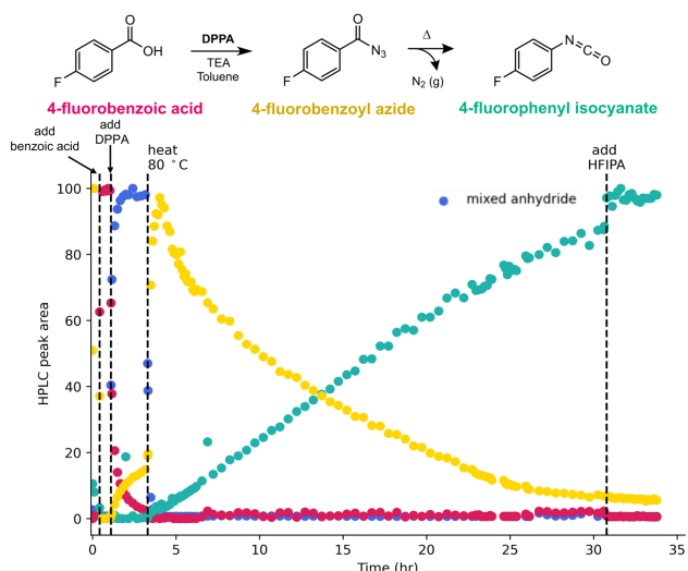
Fig. 9 Online HPLC monitoring of 4-fluorophenyl isocyanate formation with DPPA addition at 42.5 min, and heat at 169.5 min.
