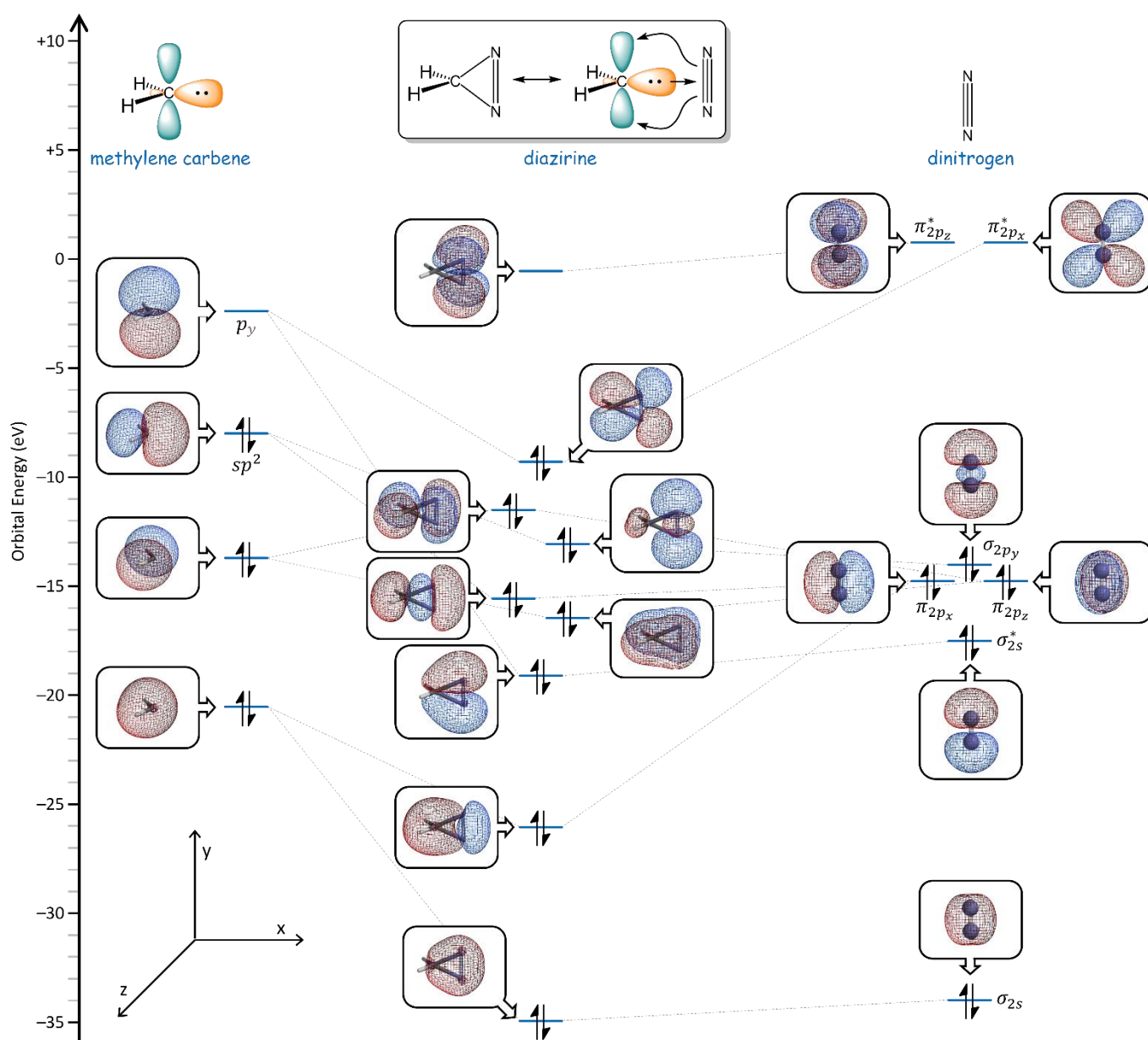
Fig. 11 Calculated frontier molecular orbitals (M06-2X/6-311+G(2df,2p)) for the parent diazirine molecule ( H_2CN_2 ), and correlations to the calculated orbitals of methylene carbene and dinitrogen.
