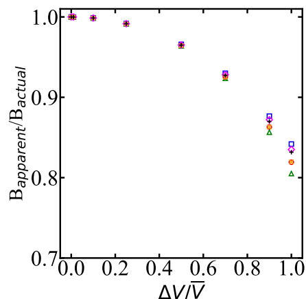
Figure 6. When droplet diameter dispersity is ignored, the inferred B_{\text{apparent}} relative to B_{\text{actual}} depends on uniform spread in volume \Delta V relative to the mean volume \bar{V} . \Delta V is the width of a uniform distribution of droplet volumes according to the uniform distribution. Symbols of the same color correspond to different widths of uniform distribution and different colors correspond to different mean volume of the droplets. B_{\text{actual}} is the predicted B with monodisperse droplets and B_{\text{apparent}} is the computed B with dispersity in droplet volume.
