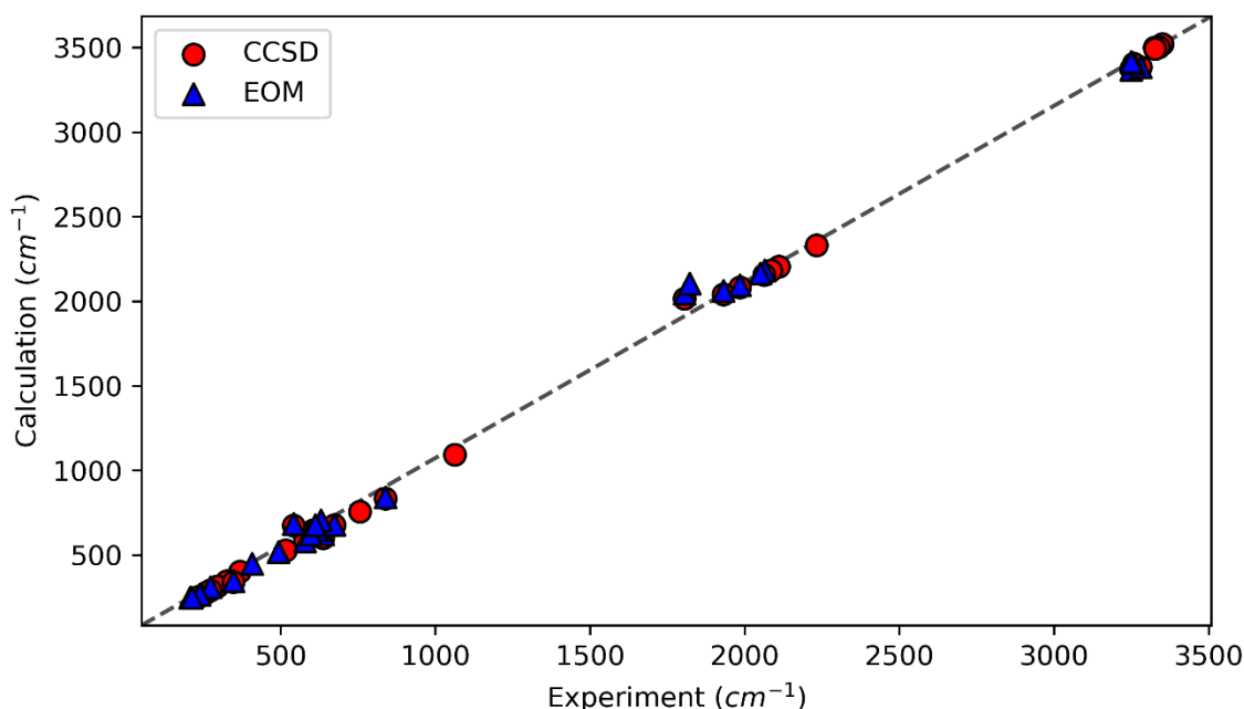
Figure 2. Comparison of the calculated harmonic frequencies with the observed frequencies for neutral \text{HCCX} ( X = \text{F}, \text{Cl}, \text{Br} and \text{I} ) and X and A states of the \text{HCCX} cations (red circles: CCSD/cc-pVTZ.; blue triangles EOMCCSD-IP/cc-pVTZ.; v_{\text{calc}} = 1.0505 v_{\text{exp}} , R^2 = 0.9993 )
