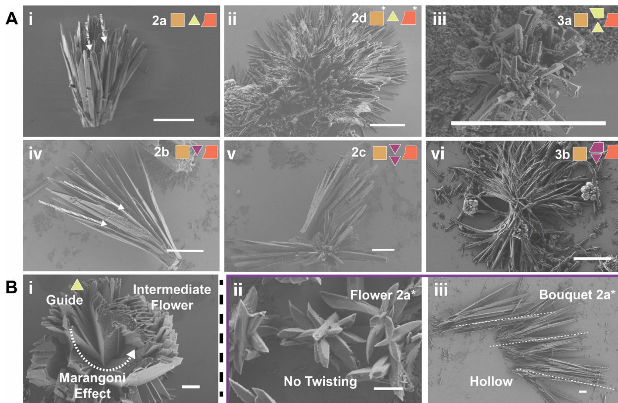
Fig. 4. Evolution of Bouquet Superstructures in the Matrices. (A) (i-vi) SEM images of set of bouquet superstructures formed in the matrix under various conditions. Scale bar = 10 \mu\text{m} . (B) (i) SEM image capturing the capillary action brought by supramolecular photoisomers, which facilitates the Marangoni effect; (ii) SEM image depicting the effect of UV light exposure to the superstructure 2a; (iii) SEM image illustrating the effect of UV light exposure to the rods in 2a. Scale bar = 2 \mu\text{m} .
