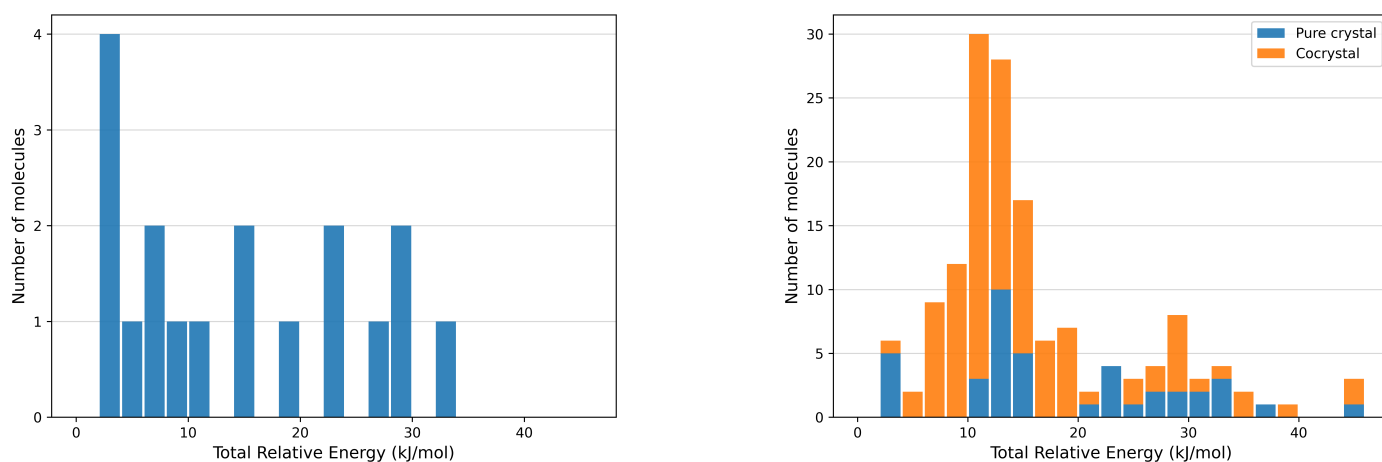
Fig. 10 (a) Histogram detailing the distribution of total relative energies \Delta E_{total} of CS guests with pure and cocrystal structures and (b) Histogram detailing the distribution of the total relative energies \Delta E_{total} of the pure and cocrystal structures studied. Histogram bin width = 2 kJ/mol.
