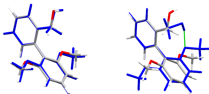
Fig. 7 Overlays of the crystalline molecular geometries (element colours) of the BBA-8,12-OMe guests in the CS (LIRLEH) with their respective local conformers (blue). Intramolecular hydrogen bonding is indicated with a green line.
