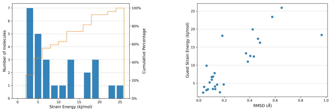
Fig. 9 (a) Histogram detailing the distribution of intramolecular strain energies of the CS guest molecules studied, with a cumulative percentage of the distribution of molecules as a function of strain energy (orange line). (b) Plot of \Delta E_{strain} against RMSD of atomic positions between the optimised crystalline molecular geometry and the conformation of the optimised isolated molecule of the CS guest molecules studied. Histogram bin width = 2 kJ/mol.
