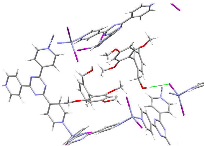
Fig. 8 Structure of two unique BBA-8,10-12-OMe guest molecules in the CS pores (LIRLIL). The highlighted guest-framework interaction relates to the guest with high strain energy, a result of distortion of the local conformer away from intramolecular hydrogen bonding.
