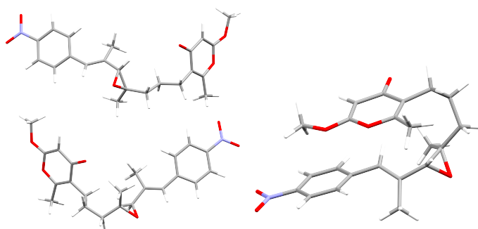
Fig. 5 (a), (b): the two unique crystalline molecular geometries of tenebrathin in the pores of the optimised CS structure (CSD Refcode CO-QBIW) and (c): the gas phase (global energy minimum) structure of tenebrathin.
