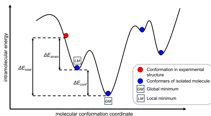
Fig. 1 Schematic of a conformational energy surface: the molecular energy vs a general conformational degree of freedom. The molecular geometry found in the experimental crystal structure is represented as a red point and the conformers of the isolated molecule are represented as blue points. The global minimum conformer, at the lowest point on the potential energy landscape, is indicated by GM. The local minimum conformer of the guest in the experimental structure is indicated by LM.
