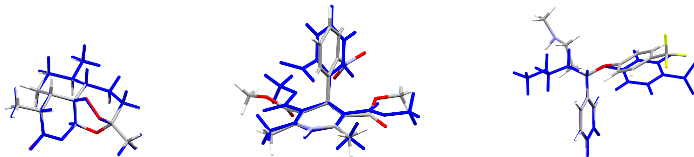
Fig. 4 Overlays of the crystalline geometry of (a) (+)-artemisinin (XAZPEW), (b) nifedipine (RECJAN) and (c) fluoxetine (CENBOP) in the optimised CS structure (element colours) with its gas phase (global energy minimum) conformer (blue).
