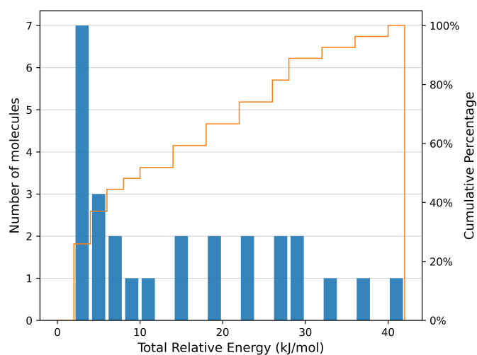
Fig. 3 Histogram detailing the distribution of the total relative energy \Delta E_{total} of the 27 distinct molecular geometries of the 15 unique guests in the 16 CS structures chosen, with a cumulative percentage of the distribution of molecules as a function of strain energy (orange line). Histogram bin width = 2 kJ/mol.
