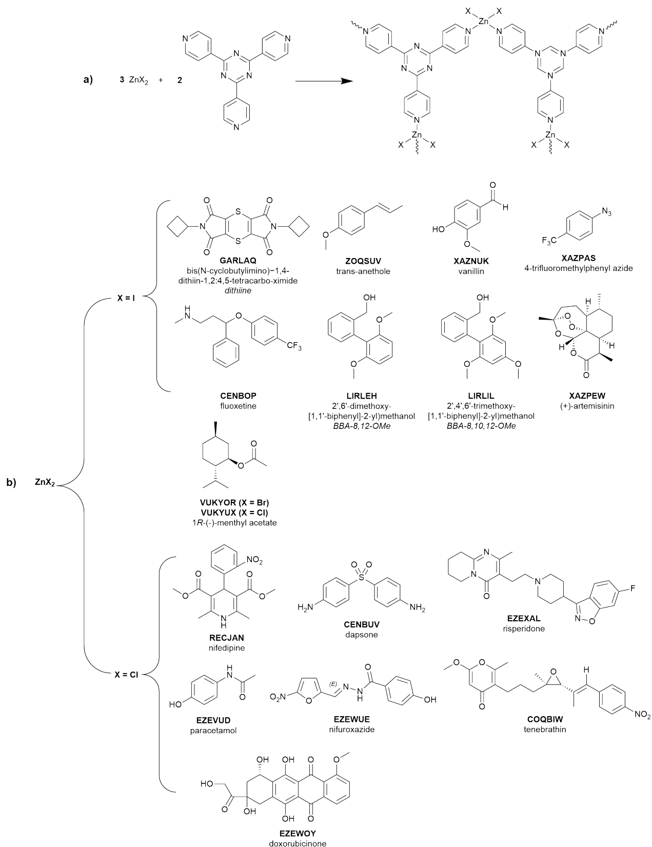
Fig. 2 (a) Schematic for the synthesis of the (\text{ZnX}_2)_3(\text{tpt})_2 crystalline sponges, where \text{X} = \text{Cl}, \text{Br}, \text{or I} . The zinc (II) ions coordinate to the tpt ligands to form the displayed repeat unit. (b) Chemical diagrams of the guest molecules and associated CSD reference codes of the studied crystalline sponge structures. Each structure includes the guest molecule soaked into the (\text{ZnX}_2)_3(\text{tpt})_2 framework.
