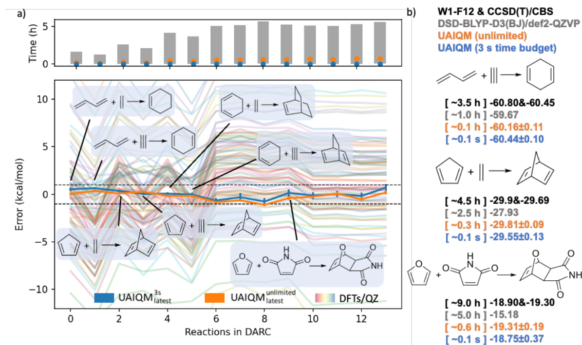
Figure 2. Performance of auto-selected UAIQM and 84 functionals, benchmarked in previously, 35 on the Diels–Alder reactions (DARC) 35,36 . a) Error of reaction energy and calculation time for each reaction. b) Comparison of time and reaction energies on representative reactions with W1-F12 & CCSD(T)/CBS (black, time for CCSD(T)/CBS), DSD-BLYP-D3(BJ)/def2-QZVP (grey), UAIQM at time budget 3s (blue) and at unlimited time budget (orange). Energies are in kcal/mol, the calculation time – CPU-hour.
