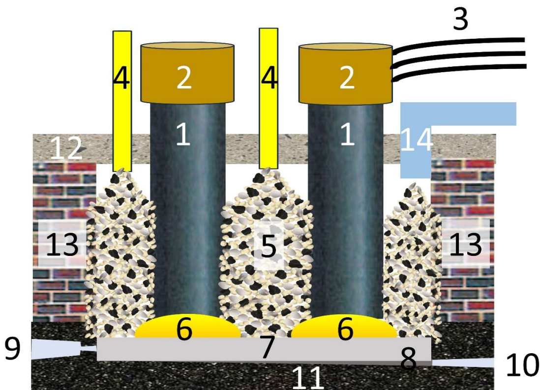
Figure 4 Electrothermal reduction of rock phosphate is done in a submerged arc furnace.
