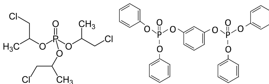
Figure 25 TCPP (left) and RDP (right) molecule structures
