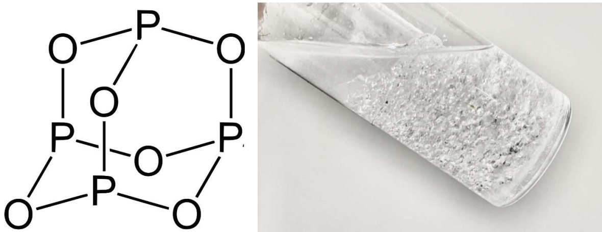
Fig 6 Phosphorus trioxide structure. The compound P_2O_5 (more precisely P_4O_{10} ) has the same structure, but with four extra oxygen atoms at the phosphorus corners sticking out. Right: phosphorus trioxide solid and liquid at 23 °C.
