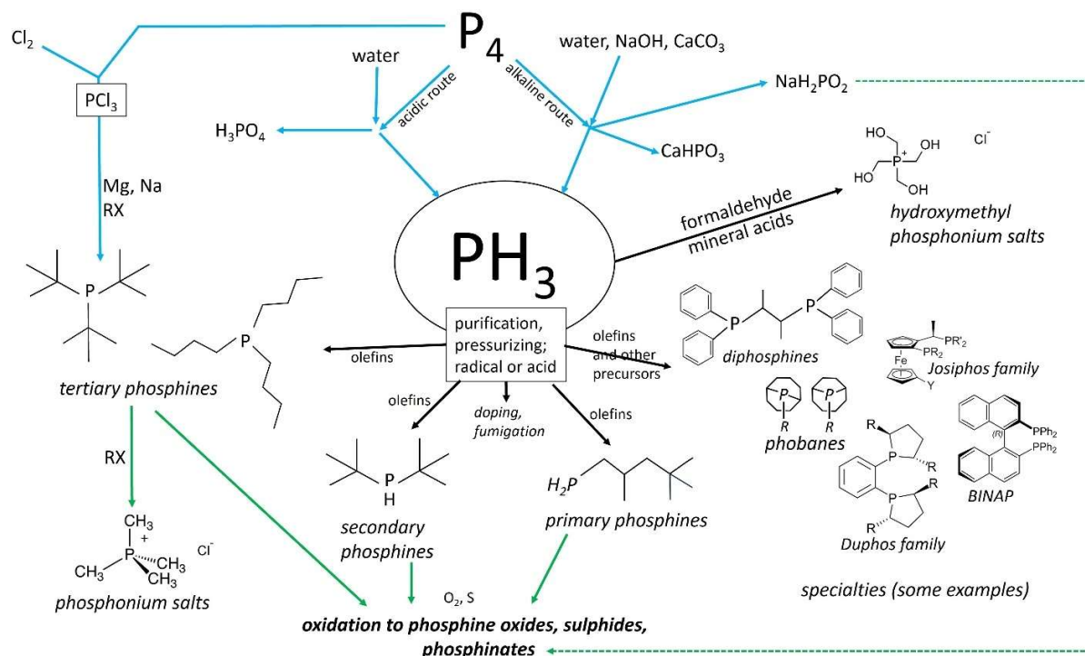
Figure 2 Phosphine routes.
