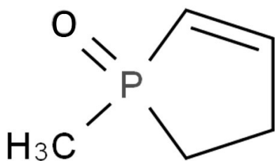
Figure 40 Five-membered cyclic phosphine oxide: 1-methyl-1-oxophospholene called MPO.
