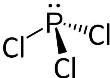
Figure 18 Fig 1 \text{PCl}_3 . The molecule has the shape of an umbrella; on the apex is a lone pair of electrons, i.e. these electrons do not take part in a chemical bond but are available for this.
