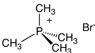
Figure 37 A phosphonium salt, tetramethylphosphonium bromide.
