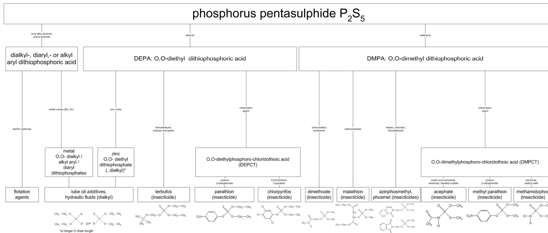
Figure 31 Some phosphorus pentasulphide, P_2S_5 , The lubricant additives box may refer to longer alkyl groups than ethyl also. Not all PS insecticides are shown.
