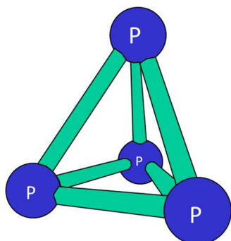
Figure 3 The P_4 molecule.
