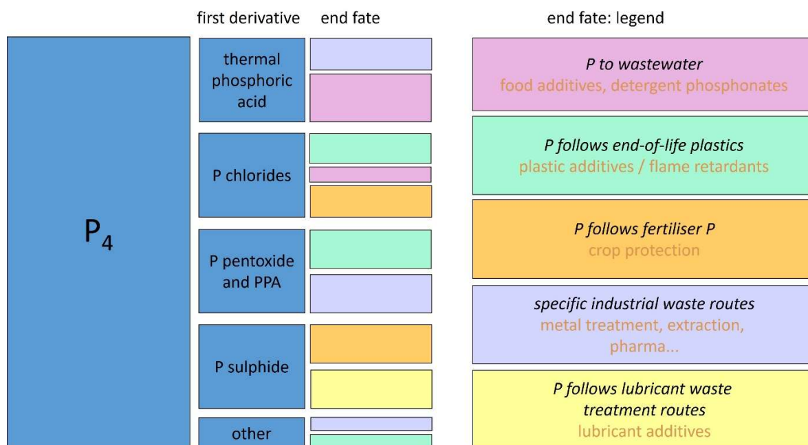
Figure 43 Main environmental fates of true P 4 derivatives
