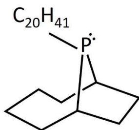
Figure 34 Eicosyl phobane, a bridged phosphine with the formal name 9-eicosyl-9-phosphabicyclo[3.3.1]nonane. The [4.2.1] arrangement is also obtained during synthesis from phosphine (PH 3 ) and cyclooctadiene.
