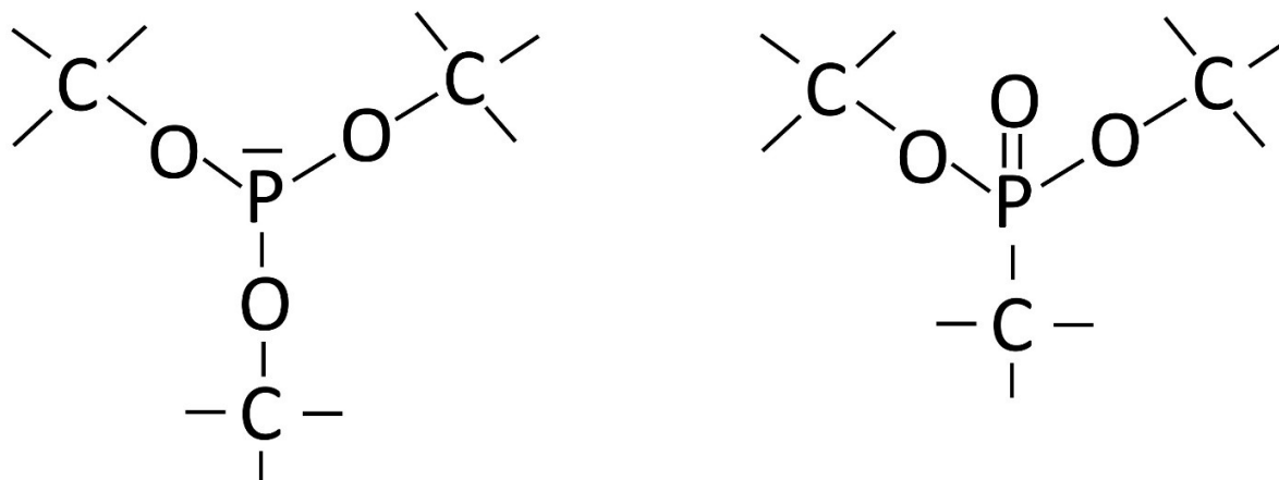
Figure 20 Trimethyl phosphite (left) and dimethyl methyl phosphonate (right). Both molecules can be described by the formula \text{C}_3\text{H}_9\text{O}_3\text{P} but the arrangement is different (i.e. they are isomers).
