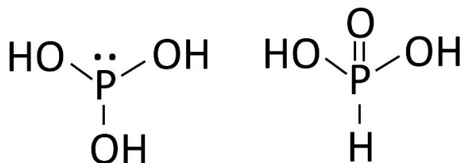
Figure 22 The two tautomers of phosphorous/phosphonic acid. These tautomers are in equilibrium, with the form shown on the right dominating.
