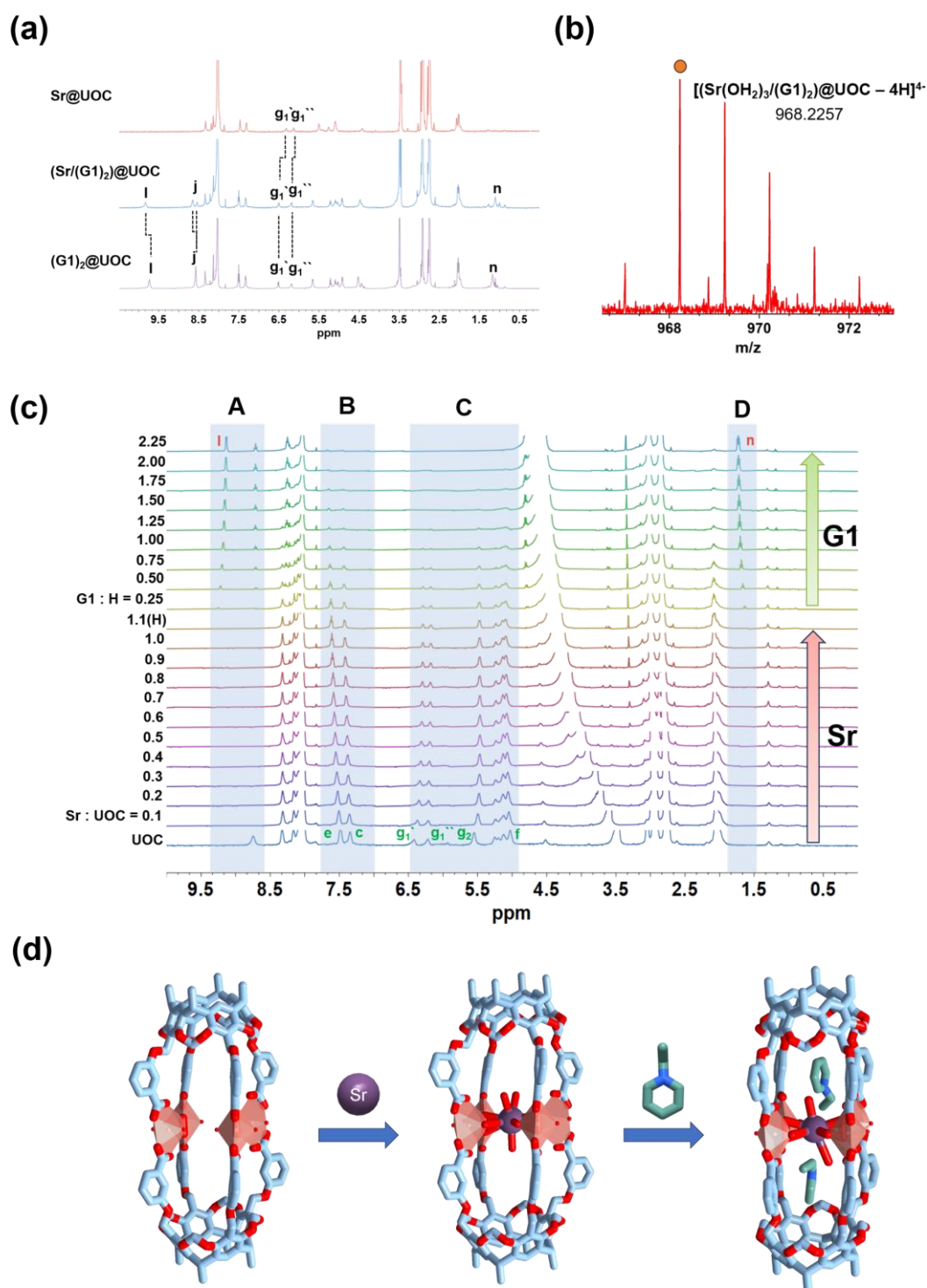
Figure 6. Encapsulation of both Sr 2+ ions and organic species [G1] + within the cavity of UOC. (a) 1 H NMR spectra of Sr@UOC, (G1) 2 @UOC, and (Sr/(G1) 2 )@UOC (DMF-d 7 , 298 K). (b) High-resolution FT-MS spectra of (Sr/(G1) 2 )@UOC. (c) 1 H NMR spectra of UOC (1.2 mM, DMF-d 7 , 298 K) titrated by Sr 2+ ions and [G1] + (dissolved in D 2 O) in turn. From bottom to top, the equivalents of Sr 2+ ions or [G1] + gradually increase. (d) Schematic formation of heterogeneous guest co-encapsulated complex (Sr/(G1) 2 )@UOC and its optimized structure.
