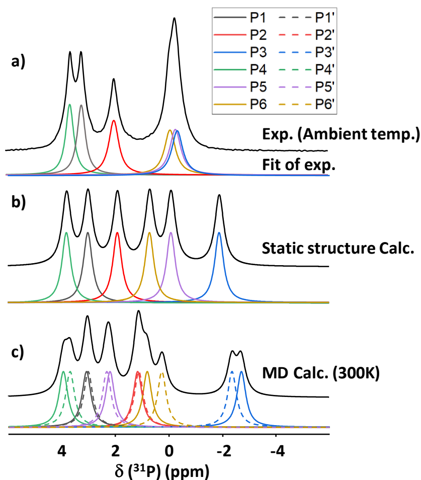
Figure 8: a) Experimental and fitted ^{31}\text{P} MAS NMR spectrum of OCP at “ambient temperature” (refrigerating unit set to 0^\circ\text{C} ), with resonances assigned according to Davies et al.; 15 b) DFT-calculated ^{31}\text{P} chemical shifts for the relaxed static structure extrapolated at 298 K; 15 c) Time-averaged calculated ^{31}\text{P} chemical shifts after MD simulation at 300 K.
