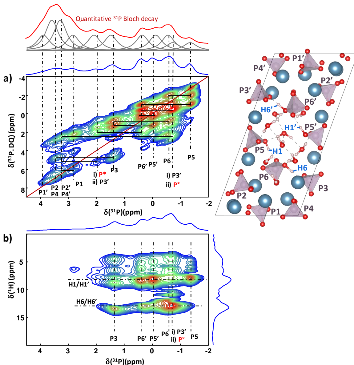
Figure 12: 2D NMR experiments recorded on unenriched OCP at ca. 100 K (temperature of the refrigerating unit): a) \{^1\text{H}\} ^{31}\text{P} - ^{31}\text{P} DNP S3 DQ/SQ correlation spectrum recorded at 9.4 T, with a 7.4 ms recoupling time, and \nu_r = 13 kHz. The fit of the quantitative direct-excitation (Bloch decay) ^{31}\text{P} MAS NMR spectrum (recorded at 100 K) is shown in red above the figure. Small shifts in positions between DQ/SQ and direct-excitation MAS peaks are observed, possibly due to surface and/or DNP effects (as discussed in the manuscript). b) ^1\text{H} - ^{31}\text{P} DNP CP-HETCOR spectrum recorded at 9.4 T; t_{\text{cp}} = 0.2 ms, \nu_r = 13 kHz. The symbols i) /ii) and \text{P}^*/\text{P}^\circ signal correspond to the 2 tentative assignments discussed in the main text.
