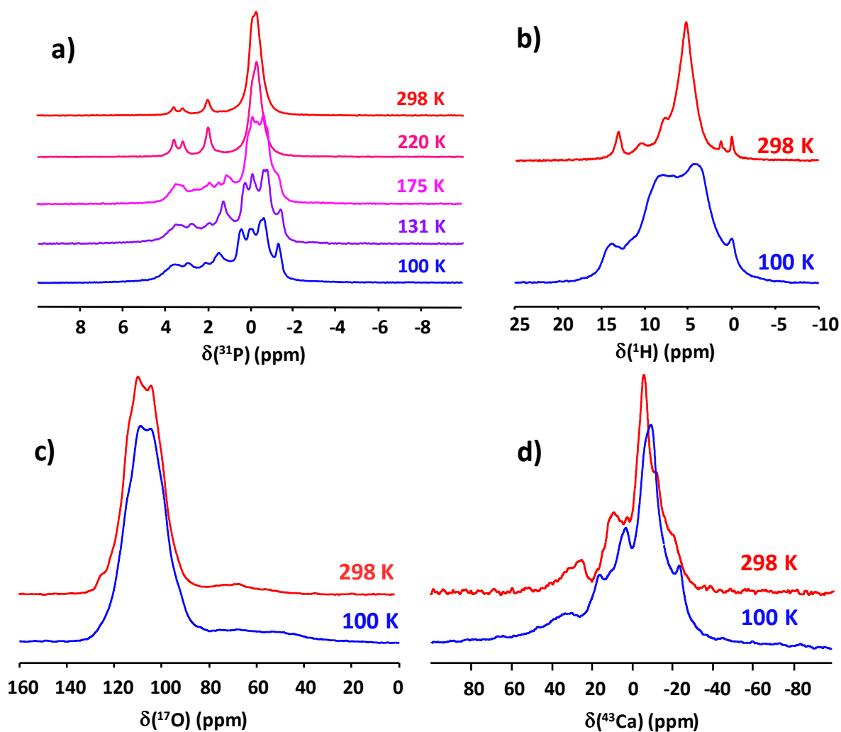
Figure 3: Evolution with temperature of a) ^{31}\text{P} CPMAS NMR spectra recorded on the unenriched OCP sample ( B_0 = 9.4\text{ T} and \nu_r = 10\text{ kHz} , b) ^1\text{H} MAS NMR spectra recorded on the ^{17}\text{O} enriched OCP sample ( B_0 = 18.8\text{ T} and \nu_r = 40\text{ kHz} ), c) ^{17}\text{O} Hahn-Echo NMR spectra (refocused over one rotor period), recorded on the ^{17}\text{O} -enriched OCP sample ( B_0 = 18.8\text{ T} and \nu_r = 25\text{ kHz} ) and d) ^{43}\text{Ca} MAS NMR spectra recorded on the 15% ^{43}\text{Ca} -enriched OCP sample ( B_0 = 18.8\text{ T} and \nu_r = 8\text{ kHz} ). Indicated temperatures are those of the refrigerating units.
