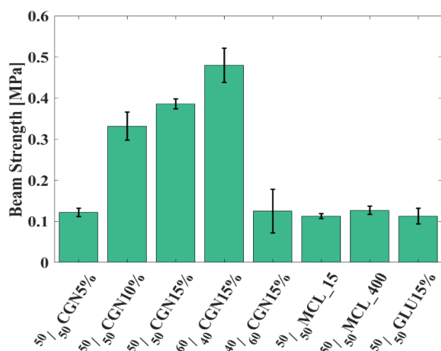
Figure 2 - BST of organics-ACC models with single-material matrix. ^{60}/_{40} CGN15% presents the highest BST.
