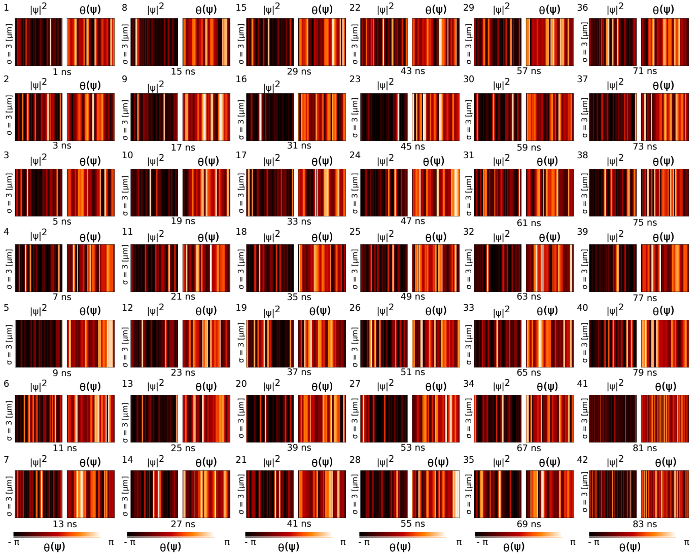
FIG. 2. Time evolution of soliton formation in a 2D anisotropic GP Equation (Hamiltonian in Equation 12) from 1 ns to 83 ns. Subfigures 1 to 42: Show the simultaneous plotting of the soliton's wave function amplitude ( |\psi|^2 ) and phase angle ( \theta(\psi) ) with a 2 ns time step.
