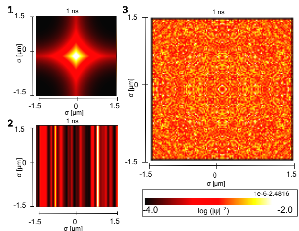
FIG. 1. (1) Evolution of the asymptotic curve in the numerical analysis of the 2D anisotropic Gross-Pitaevskii (GP) equation, independent of temperature, within a square domain of 3 \mu\text{m} in length. (2) Formation dynamics of observed solitons in the numerical analysis of the 2D anisotropic GP equation, accounting for temperature dependency, within a square domain of 3 \mu\text{m} in length. (3) Dynamics of observed condensates in the numerical analysis of the 2D anisotropic GP equation, considering temperature as a function of critical density, within a square domain of 3 \mu\text{m} in length.
