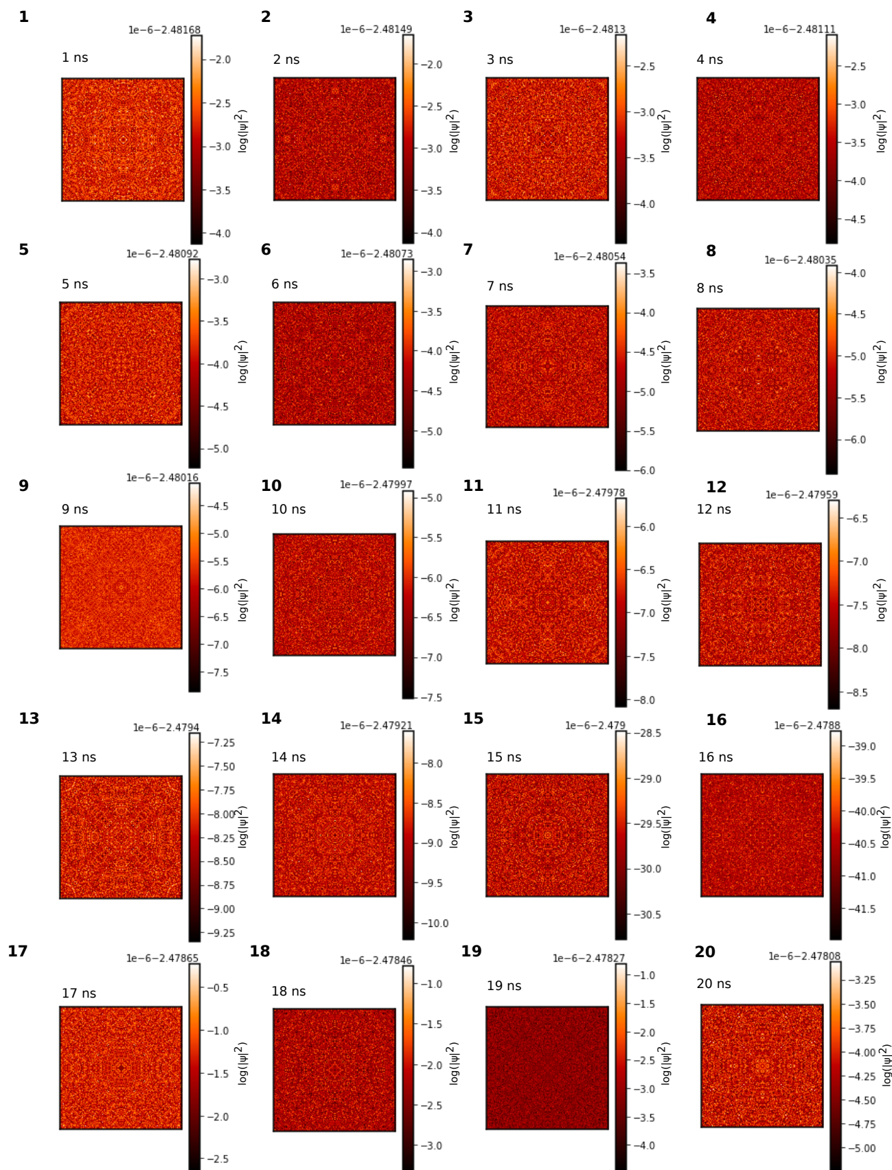
FIG. 3. 1 - 20: Growth dynamics and nucleation of BEC with time according to equation 14 – initial time frame = 1 ns with time steps of 1 ns and final time frame = 20 ns with time step = 1 ns.
