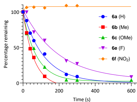
Figure 2: Kinetic follow-up of the photorelease of 6a–f mediated by 1PE (LED, 405 nm). The remaining percentage was determined by HPLC analysis and is the average of three runs. Lines are least-squares fits of the data to a simple exponential decay.
