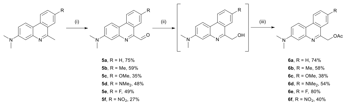
Scheme 2: Preparation of -OAc phenanthridine derivatives. Reagents and conditions: (i) SeO 2 , dioxane, reflux, 3 h; (ii), (iii) NaBH 4 , Ac 2 O, 0 °C, 16 h.
