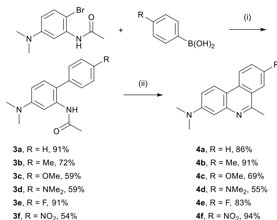
Scheme 1: Synthesis of 3,6,8 trisubstituted phenanthridine derivatives. Reagents and conditions: (i) Pd(PPh 3 ) 4 , Na 2 CO 3 , THF/H 2 O, 100 °C, 24 h; (ii) POCl 3 , reflux, 33 h.
