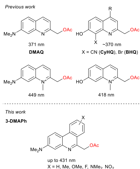
Figure 1: General structure of first and second-generation quinoline-based PPGs (top) and novel phenanthridine-based PPGs (bottom).
