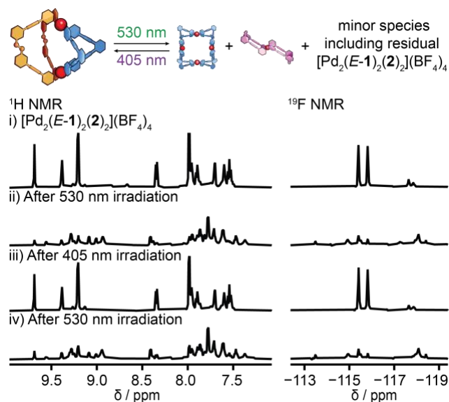
Figure 3. Partial 1 H (600 MHz) and 19 F (565 MHz) NMR spectra in DMSO- d 6 showing photoswitching of heteroleptic cage [Pd 2 ( E-1 ) 2 ( 2 ) 2 ](BF 4 ) 4 . i) before irradiation; ii) after 530 nm 10 min; iii) 405 nm 5 min; iv) 530 nm light 10 min irradiation. The PSS composition (PSS 530 = 88% Z -1%, the same as for the
