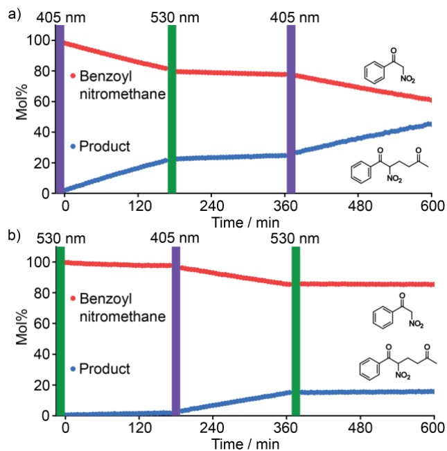
Figure 5. Photoswitchable catalysis by the heteroleptic cage Pd 2 (E-1) 2 (2) 2 (BARF) 4 in CD 2 Cl 2 :CD 3 CN 11:1 monitored by 1 H NMR spectroscopy. Reaction conditions: benzoyl nitromethane (17 mM), methyl vinyl ketone (33 mM), and 18-crown-6 (12 mM), [Pd] 2.0 mM. Irradiation by 405 nm (5 min) and 530 nm (10 min) outside of the NMR instrument, with colored bars representing the time between NMR measurements, see SI-S16 for details.
