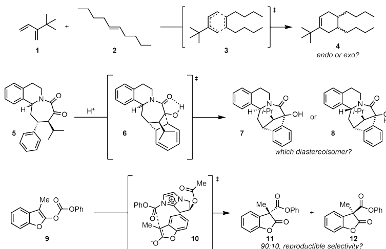
Figure 1: On top, Diels Alder reaction between 4,4-dimethyl-3-methylenepent-1-ene ( 1 ) and (E)-dec-5-ene ( 2 ). On middle, diastereoselective intramolecular acidic cyclization. On bottom, enantioselective organo-catalysed Black rearrangement.
