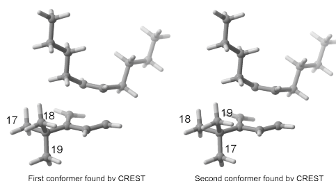
Figure 2: Two conformers found by CREST and considered as duplicates in FASTCAR.
