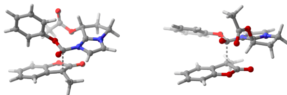
Figure 6: On the left, lowest TS found for major enantiomer. On the right, lowest TS found for the minor enantiomer.
