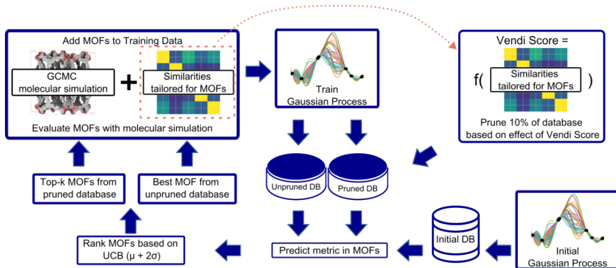
Figure 2. Workflow for our VBO framework. An initial GP, trained with data for two randomly chosen MOFs, is used to predict the performance metric in the starting database. k+1 MOFs are selected for molecular simulation evaluation based on the upper confidence bound (UCB) acquisition function. One MOF is chosen as the MOF scoring the highest UCB just as in standard Bayes optimization. The remaining k MOFs are selected based on UCB but only after 10% of the database is pruned. The MOFs pruned from the database are the MOFs that would increase the least the Vendi Score of the cumulative set of MOFs evaluated by molecular simulation. The top k+1 MOFs selected are then evaluated using molecular simulations. To perform a new iteration, the molecular simulation data for the newly evaluated k+1 MOFs are added to the data for training the GP, and the MOF selection process is repeated.
