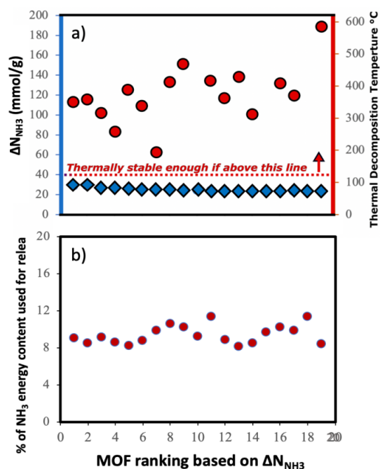
Figure 11. a) Thermal stability in top-20 MOFs from VBO campaign. Blue diamonds indicate \Delta N_{NH_3} (left-axis) and red circles indicate predicted thermal decomposition temperature (right-axis). Top-20 MOFs appear likely to withstand operation conditions. b) Estimated energy penalty to release stored NH_3 as percentage of the hydrogen-based energy content of NH_3 (22.5 MJ/kg NH 3 ) in the top-20 MOFs. Penalty hovers around 8 to 12 percent on NH_3 energy content.
