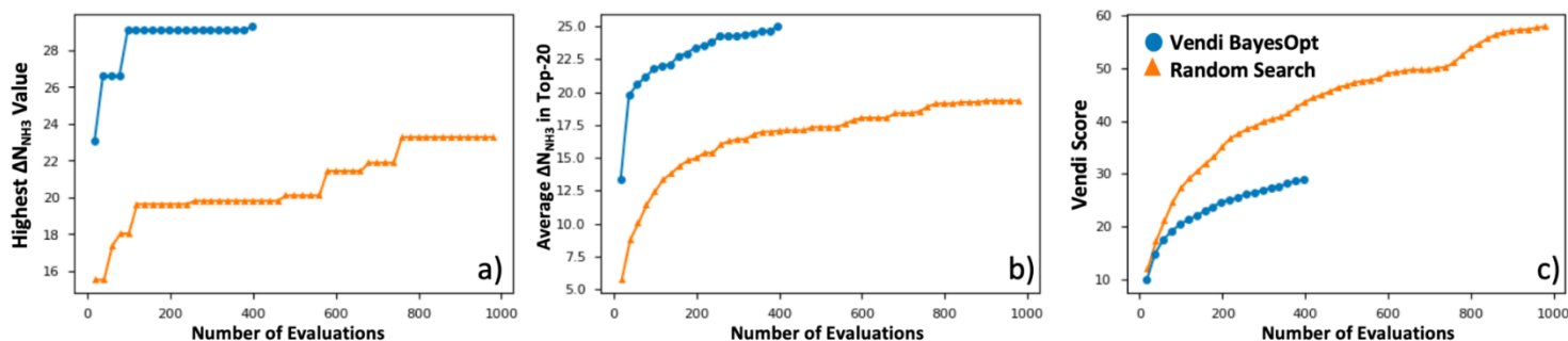
Figure 7. Evolution of VBO campaign (blue) in the \sim 10,000 MOF database, when searching for MOFs for \text{NH}_3 storage, compared to the evolution of the random search (orange). a) Evolution of the highest \Delta N_{\text{NH}_3} found among evaluated MOF at a given point in the campaign. b) Evolution of the average \Delta N_{\text{NH}_3} among the top-20 evaluated MOFs at a given point in the campaign. c) Evolution of the Vendi Score of evaluated MOFs at a given point in the campaign. Note that the VBO campaign was ended early due to negligible changes in the highest \Delta N_{\text{NH}_3} since the 80 th evaluation. Once again VBO greatly outperformed random search.
