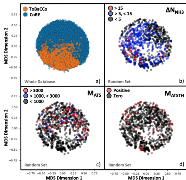
Figure 4. MOF mapping onto two-dimensional plots by using multidimensional scaling (MDS) representations. a) all MOFs in the hybrid database colored by their origin (either the ToBaCCo database or the CoRE database). b-d) 1,000 random MOF subset, colored by range of \Delta N_{NH_3} (b), M_{ATS} (c), and M_{ATSTH} (d) performance metrics. The extent of segregation observed is a harbinger of the efficacy of our MOF kernel similarity as input to train the GP.
