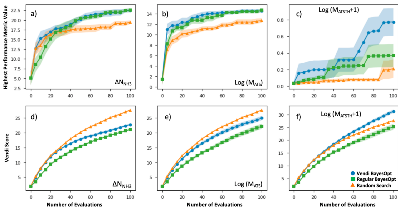
Figure 6. Efficacy of VBO (blue) applied on a 1,000 subset of random MOFs compared to Bayesian optimization (green) and random search (orange). Top row presents the evolution of the highest value of the performance metric as the number of MOF evaluations increases for a) \Delta N_{\text{NH}_3} for ammonia storage, b) M_{\text{ATS}} for ammonia removal from plasma reactor, and c) M_{\text{ATSTH}} for ammonia capture from air. Bottom row presents the evolution of the Vendi Score for the set of evaluated MOFs as the number of MOF evaluations increases for d) \Delta N_{\text{NH}_3} for ammonia storage, e) M_{\text{ATS}} for ammonia removal from plasma reactor, and f) M_{\text{ATSTH}} for ammonia capture from air. Results in a)-f) are averaged across 10 repeat runs, the average value is indicated by the solid line, whereas the standard deviation is indicated by the shaded area. Both VBO and Bayesian optimization outperformed random search, but VBO provided higher diversity of MOF “solutions.”
