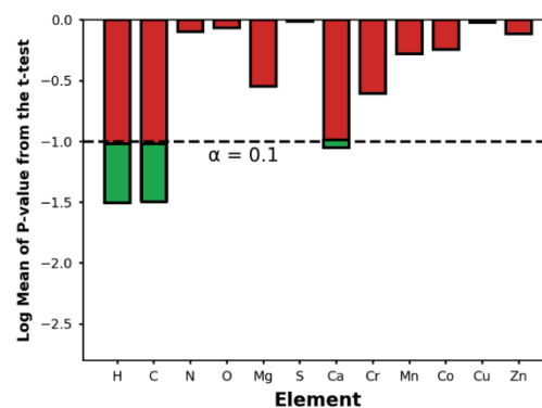
Figure 9. Statistical significance for comparison of elemental compositions between the top-14 MOFs and the entire database based on the p-values derived from the t-test. The dashed line represents our chosen critical value for the one-sided t-test. Bars that fall below this threshold indicate elements that are statistically significantly more abundant in the top-performing MOFs. Ca is a metal that appears significantly more frequently in the top-14 MOFs than in the full database.
