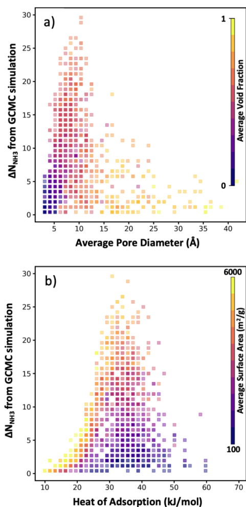
Figure 8. Plots of structure-performance relationships for \text{NH}_3 storage. Each square bin corresponds to a combination of the \Delta N_{\text{NH}_3} performance metric and MOF property, where the transparency of each square bin is indicative of the number of MOFs in the bin, and the color of each bin reflects the average value of the property in the side color scale across all MOFs in the bin. a) \Delta N_{\text{NH}_3} versus MOF average pore diameter (APD), with each bin colored by MOF void fraction. b) \Delta N_{\text{NH}_3} versus heat of adsorption Q_{\text{st}} , with each bin colored by gravimetric surface area. Optimal APD and Q_{\text{st}} appears to be 10 Å and 33 kJ/mol, respectively.
