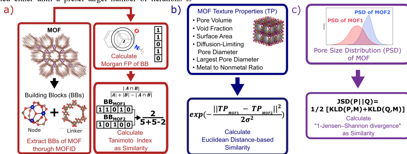
Figure 3. Schematic representation of methods to calculate kernel similarity between MOFs. a) Chemical similarity ( K_{node} and K_{linker} kernels) obtained by decomposing two MOFs into their building blocks, and calculating the Tanimoto index between the Morgan fingerprints of their building blocks. b) Global textural properties similarity ( K_{global} kernel) obtained by calculating the radial basis function Kernel of the Euclidean distance between the property vectors of two MOFs. c) Detailed pore structure similarity ( K_{PSD} kernel) obtained by calculating the difference between one and the Jensen-Shannon divergence between the pore size distributions (PSDs) of two MOFs. The different kernels cover different aspects of MOFs, and by tuning the weights of each Kernel, the representation is adaptable to prediction of properties with different level of dependence on MOF chemistry and structure.
