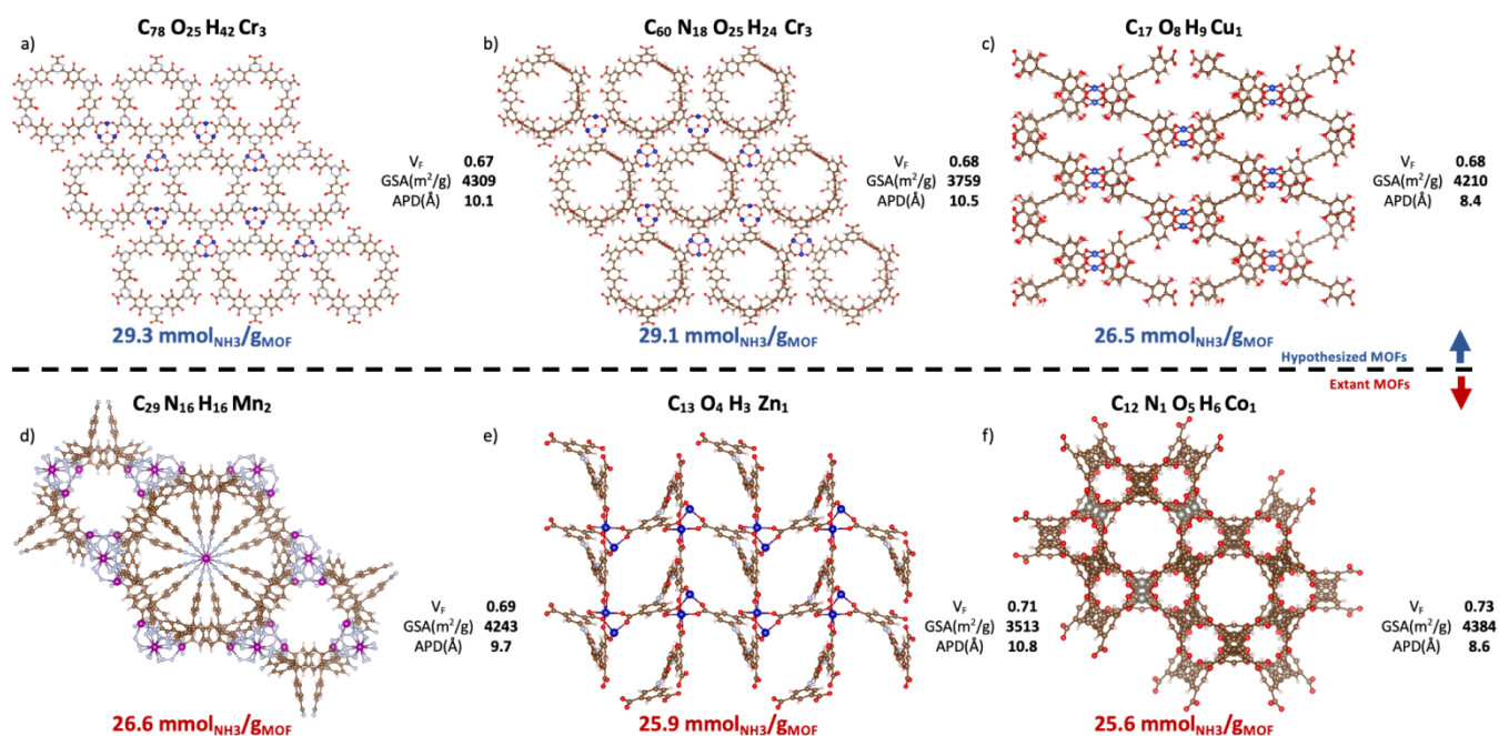
Figure 10. Top-6 MOFs ranked by \Delta N_{NH_3} value. Hypothesized and extant MOFs are in the top and bottom rows, respectively. V_f , GSA, and APD represent, respectively, the void fraction, gravimetric surface areas, and average pore diameter from pore size distribution. The CSD refcode and corresponding publication can be found in Table S5. The three hypothesized MOFs are potentially synthesizable per the free energy criterion by Anderson and Gómez-Gualdrón (Table S6). 53 Ca MOFs appear in the top-14 but not in top-6 presumably due to suboptimal textural properties.
