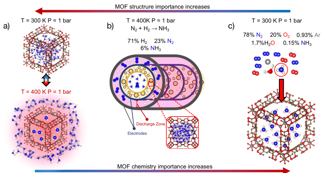
Figure 1. Applications for which \text{NH}_3 adsorption-based MOF performance metrics were optimized to test the efficacy of our Vendi Bayesian optimization (VBO) framework. a) Adsorptive \text{NH}_3 storage at ambient conditions with release at 400 K. b) Membrane-based \text{NH}_3 removal from plasma reactors during \text{NH}_3 synthesis at 400 K and 1 bar. c) Dilute \text{NH}_3 capture from air in adsorbent traps at ambient conditions. Gas-phase composition relevant to each application indicated at the top. The three chosen metrics present different levels of dependence on MOF chemistry and structure.
