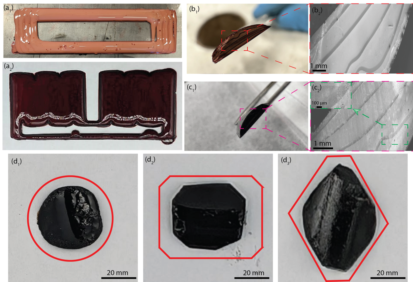
Fig. 3 MDIW printed objects with the (a 1 ) ladder structure (5 layers along the z-axis and partially cured upon removal from the build plate), (a 2 ) double mat structure (5 layers along the z-axis and fully cured after stage I curing); (b 1 ) Cross-sectional photograph of the ladder structure removed from the build plate with the (b 2 ) cross-sectional SEM image showing controlled layer quality; (c 1 ) cross-sectional photograph of carbonized ladder structures and the (c 2 ) cross-sectional SEM image of carbonized ladder structures with an insert image highlighting the porosity. Various machined geometries with red lines indicate the desired geometries of (d 1 ) circular, (d 2 ) chamfered rectangular, and (d 3 ) diamond vs. dimensions after the carbonization
