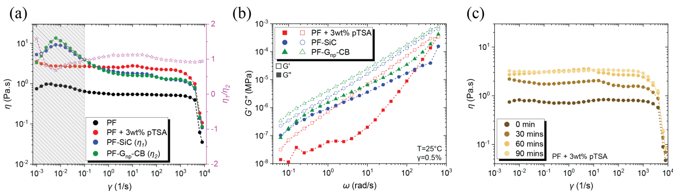
Fig. 2 Rheological studies showing (a) the change in viscosity with the addition of acid catalyst (pTSA) and dispersions of SiC and G_{np} -CB nanoparticles. The pink stars indicate the viscosity ratio around 1 between PF-SiC and PF- G_{np} -CB, (b) flow sweep highlighting the storage and loss moduli of the feedstocks, and (c) change in viscosity with the addition of pTSA as a function of time at the room temperature (RT).
