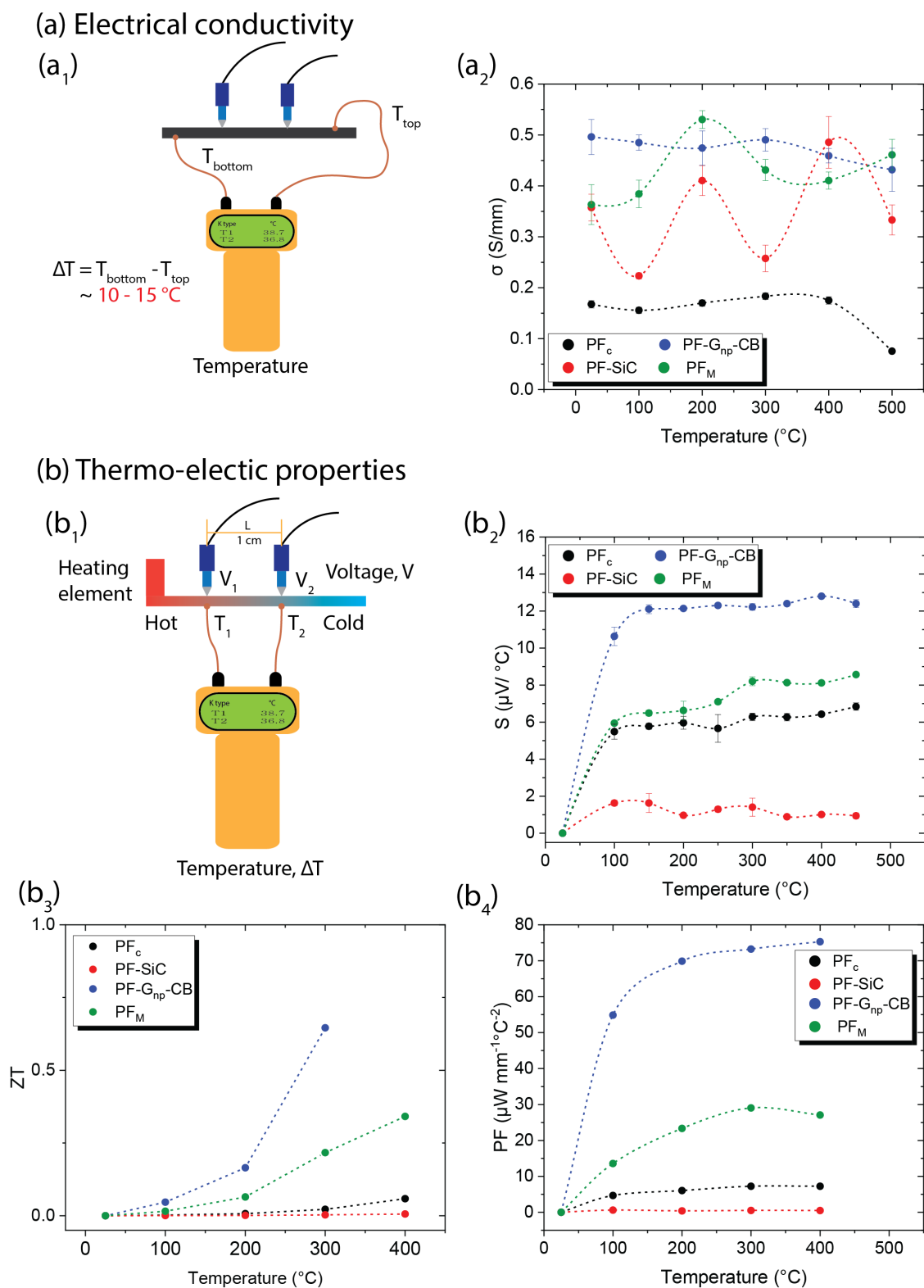
Fig. 5 (a) Electrical conductivity measurements as a function of temperature with (a 1 ) an illustration of the laboratory-made measurement setup and (a 2 ) graphical representation of the measured and calculated values of electrical conduction in S/mm from room temperature to 500°C. (b) Seebeck effect/thermo-electric measurements with (b 1 ) illustration of laboratory made measurement setup, (b 2 ) graphical representation of seebeck effect (S) measurement with the heating element temperature reaching up to 450°C, (b 3 ) calculated values of figure of merit, and (b 4 ) calculated values of power factor. (PF)
