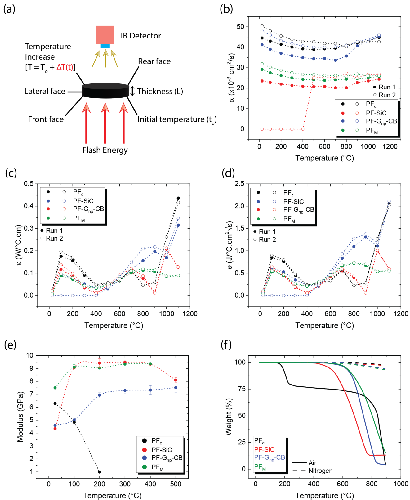
Fig. 4 (a) Illustration highlighting the measurement technique of laser flash thermal diffusivity, (b) measured values of diffusivity of carbonized samples for two consecutive runs from room temperature to 1100°C, (c) calculated values of thermal conductivity, (d) calculated values of effusivity, (e) DMA analysis of carbonized samples from room temperature to 500°C or until failure in air, and (f) TGA analysis of carbonized sample showing the failure due to oxidation in air and inert (nitrogen) environment.
