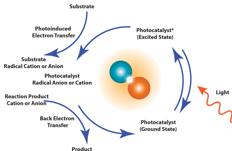
Figure 1: A generalized photoredox catalysis cycle (blue arrows) with a cartoon representing a photoinduced electron transfer event.
