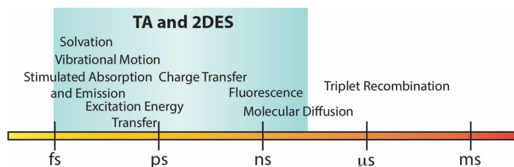
Figure 2: Overview of the timescales of molecular processes in solution associated with photoredox catalysis relative to the time resolution of TA and 2DES. The time resolution of TA and 2DES can extend beyond the nanosecond regime but different delay methods are generally required. The timescale ranges shown here are approximate and longer or shorter timescale outliers exist for all processes shown here.
