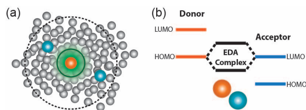
Figure 4: (a) Cartoon schematic representing diffusion limits and excited state lifetimes for photoredox catalysis. The grey, blue, and orange spheres are solvent molecules, reactants, and the photocatalyst, respectively. The green circle represents the diffusion limit of a photoexcited organic radical. Since the lifetime of an organic radical is expected to be short, the photocatalyst
