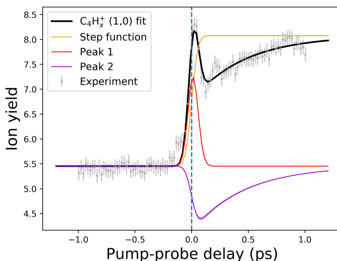
Fig. 10 An example of the pump-probe fit for the (1,0) channel of the C 4 H x + fragment. Points with error bars present experimental points retrieved from the PImMS camera, while the solid lines demonstrate the fitted curve (black line) and fit components (colored lines). The step function (yellow line) represents the static change in given ionic species production in the pump before probe and probe before pump regimes. Peak 1 (red line) corresponds to the (0,0)→(1,0) channel, while Peak 2 (violet line) corresponds to the (1,0) → (1,1,0)/(1,0,0) channel (see Figures 8 and 9). The vertical dashed line shows the temporal overlap of pump and probe pulses. All the fits are available in the ESI.
