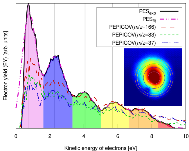
Fig. 3 Experimental pump-probe delay averaged photoelectron spectrum of FLU (solid line) and PEPICOV-disentangled spectra for the parent FLU^+ ( m/z = 166 ), FLU^{2+} ( m/z = 83 ), and the fragment ion at m/z = 37 . The different colored areas underneath the spectrum and the vertical lines highlight different ATI peak orders. The inset shows the distorted raw electron VMI image. The vertical lines correspond to the circles in the inset image. The full PEPICOV map is available in the ESI
