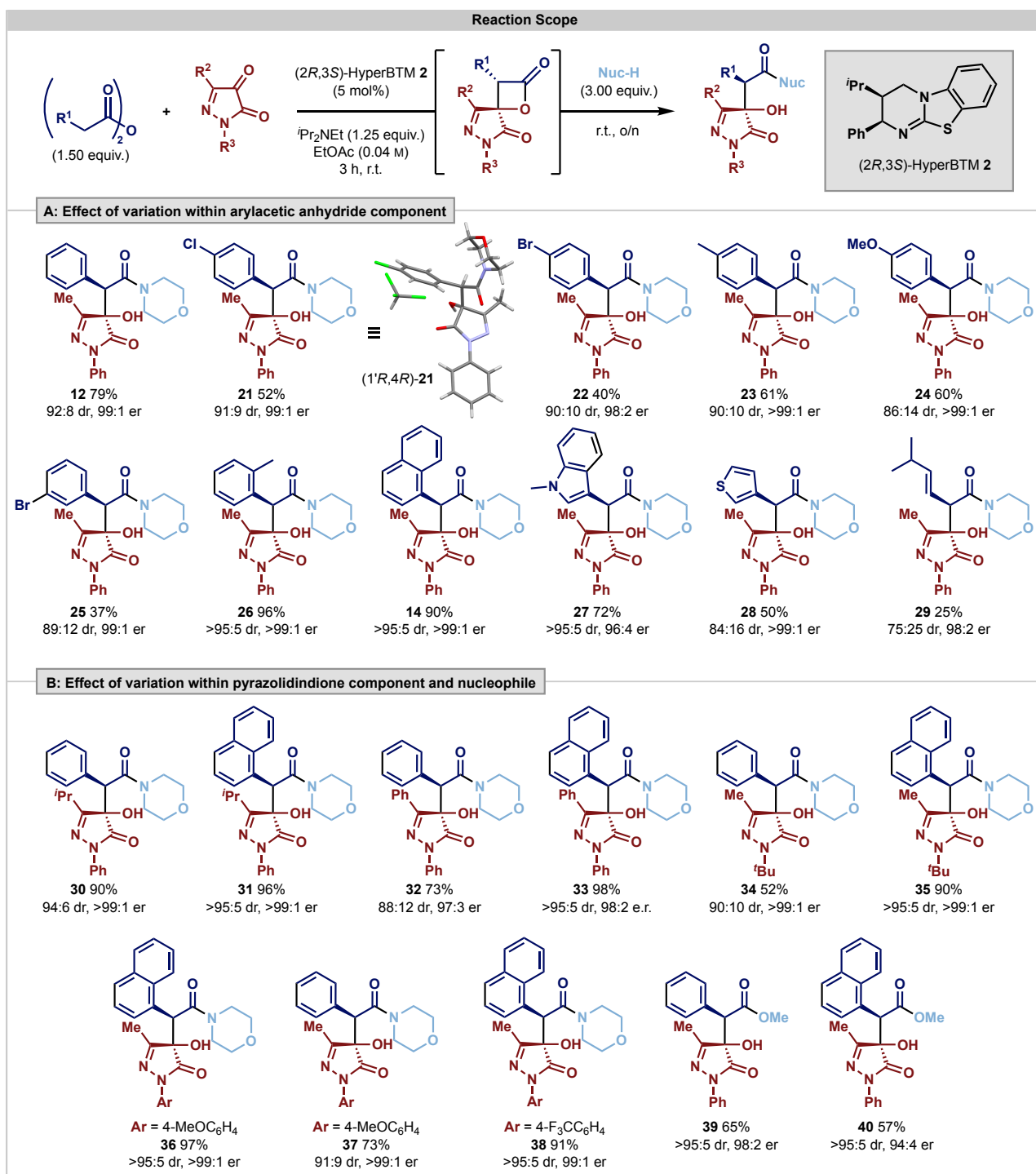
Scheme 2: [a] All reactions performed on 0.25 mmol scale with 1.0 equiv. of dione and 1.5 equiv. of anhydride. [b] Product dr assessed by 1 H NMR analysis of the crude reaction mixture. [c] Yields are isolated yields after chromatographic purification; all product ers are determined by HPLC analysis on a chiral stationary phase.
