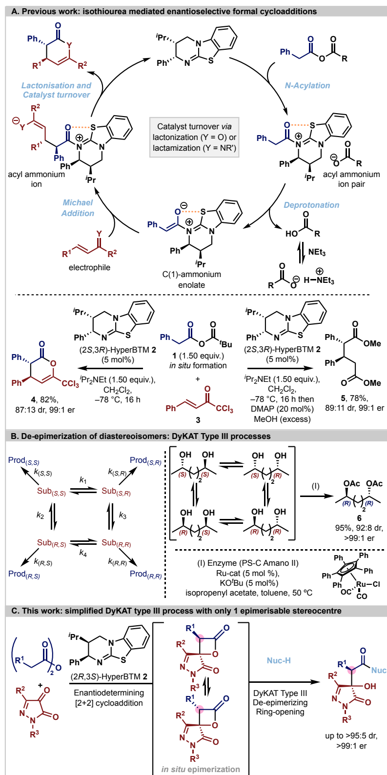
Figure 1: A. Previous work. B. DyKAT type III de-epimerization processes. C. This work: Coupling an enantioselective catalytic [2+2]-cycloaddition with a DyKAT type III ring-opening process.
