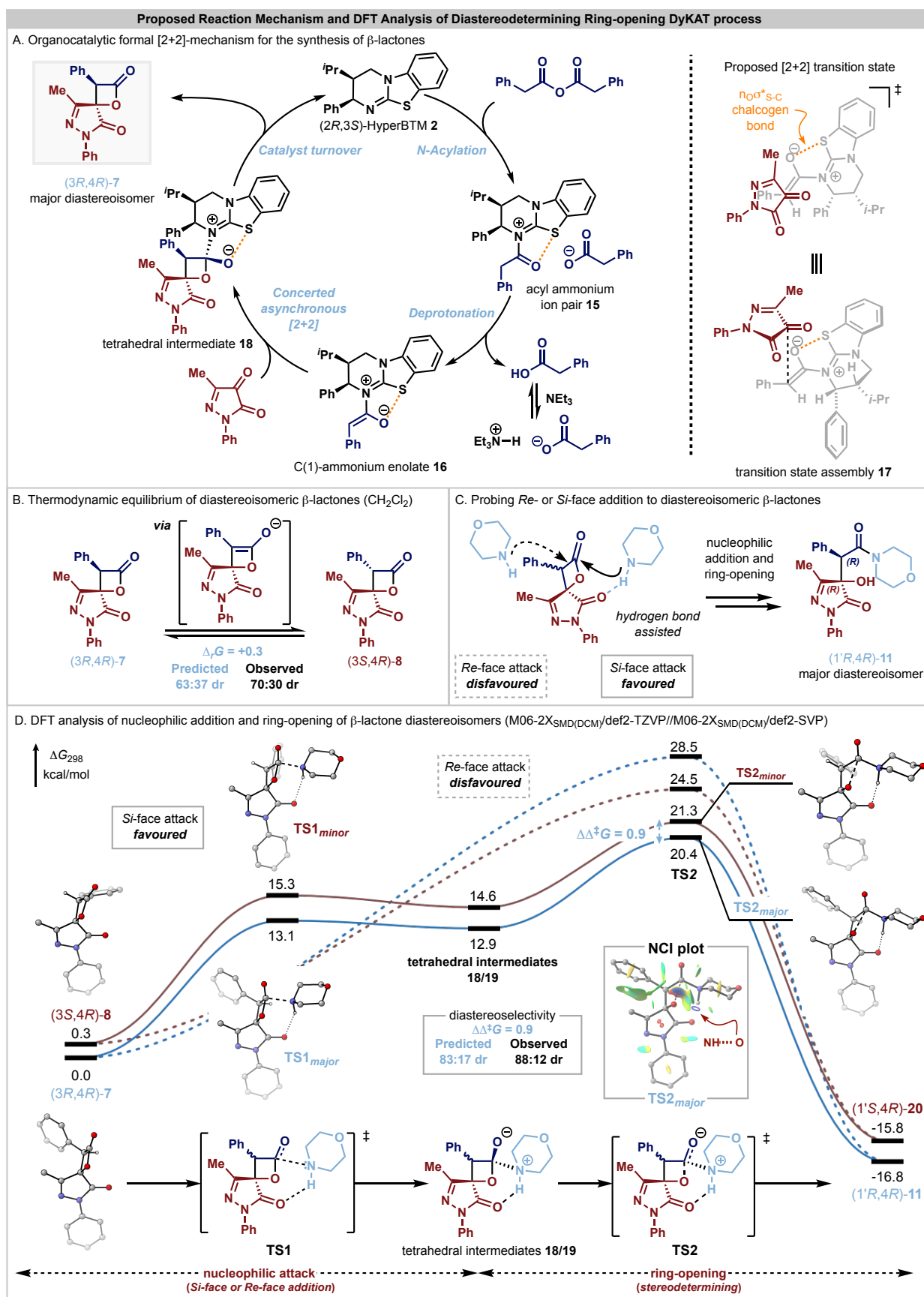
Figure 2 DFT analysis of pathways from the interconvertible (3R,4R)-7 and (3S,4R)-8 \beta -lactone diastereoisomers. M06-2X SMD /def2-TZVP//M06-2X SMD /def2-SVP Gibbs free energies ( \Delta G_{298} ) are shown in kcal/mol and selected hydrogen atoms have been removed for clarity.
