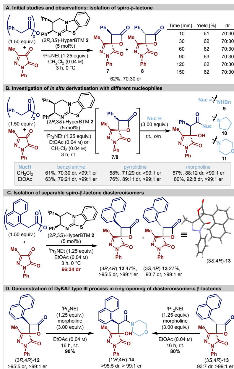
Scheme 1: [a] Reactions performed on 0.25 mmol scale with 1.0 equiv. of 3-methyl-1-phenylpyrazol-3,4-dione and 1.5 equiv. of homoanhydride. [b] Product dr assessed by ^1\text{H} NMR analysis of the crude reaction mixture. [c] Yields are isolated yields after chromatographic purification; all product ers are determined by HPLC analysis on a chiral stationary phase.
