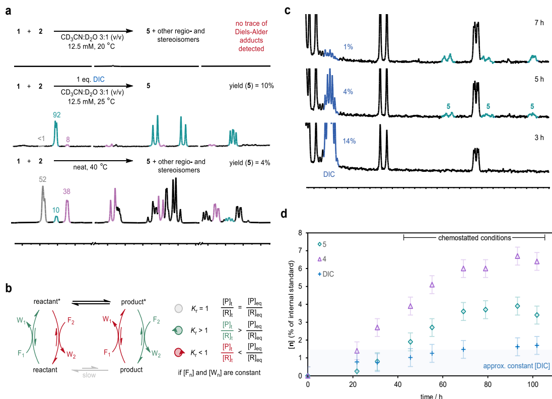
Fig 4 | Reaction selectivity and mechanistic insights. a Partial ^1H NMR stackplot (600 MHz, CD_3CN:D_2O 3:1 (v/v), 293 K) showing the regioselectivity, stereoselectivity and yield of the unfuelled reaction (top) and the ratcheted synthesis under the same conditions (middle), in comparison with a thermal synthesis (bottom). Numbers denote the relative proportions (%) of the exo-ortho ( 5 , teal), endo-ortho (purple) and meta - (grey) isomers. b Ratcheting synthesis through an information ratchet
