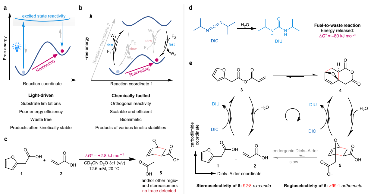
Fig 1 | Endergonic synthesis using a ratchet mechanism. a Typical endergonic chemical transformation, for example a deracemisation or isomerisation reaction, driven by light. Differences in
