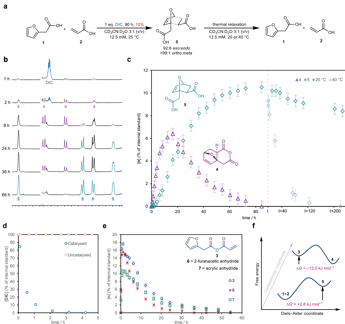
Fig 2 | Ratcheted synthesis of 5. a Ratcheted synthesis of 5 and, in the absence of the chemical fuel, its relaxation to the equilibrium distribution under the same conditions. b Partial 1 H NMR (600 MHz, CD 3 CN:D 2 O 3:1 (v/v), 298 K) stackplot showing the consumption of DIC (blue) and the formation of 4 (purple) and 5 (teal) over time. DIC addition at t = 0. c Kinetics of the formation of 4 (triangles) and 5 (diamonds) and the subsequent retro-Diels–Alder of 5 to 1 and 2 at 20 °C or 40 °C beginning at time t. Thermal relaxation t 1/2 20 °C ~16 days, t 1/2 40 °C = 25 h. d Kinetics of carbodiimide hydration catalysed by the endergonic reaction 1 + 2 ⇌ 5 (blue) and the uncatalysed background (orange). e Kinetics of mixed ( 3 , circles) and symmetrical ( 6 , crosses and 7 , squares) anhydride formation and hydrolysis. Symmetrical anhydrides are consumed through hydrolysis, whereas 3 either hydrolyses or reacts to form 4 . Formation and hydrolysis of 3 constitutes an energy-consuming futile cycle. f Free energy profile of ground state species of the anhydride chemical state calculated using (B3LYP/6-31+G(d,p)/GD3BJ) level of theory with corrections for solvation (PCM in acetonitrile (ε = 35.688)). Free energy profile of the diacid chemical state based on experiment. Energies in kJ mol -1 . Error bars refer to the measurement of ratios of NMR integrals (±0.5% relative to starting materials).
