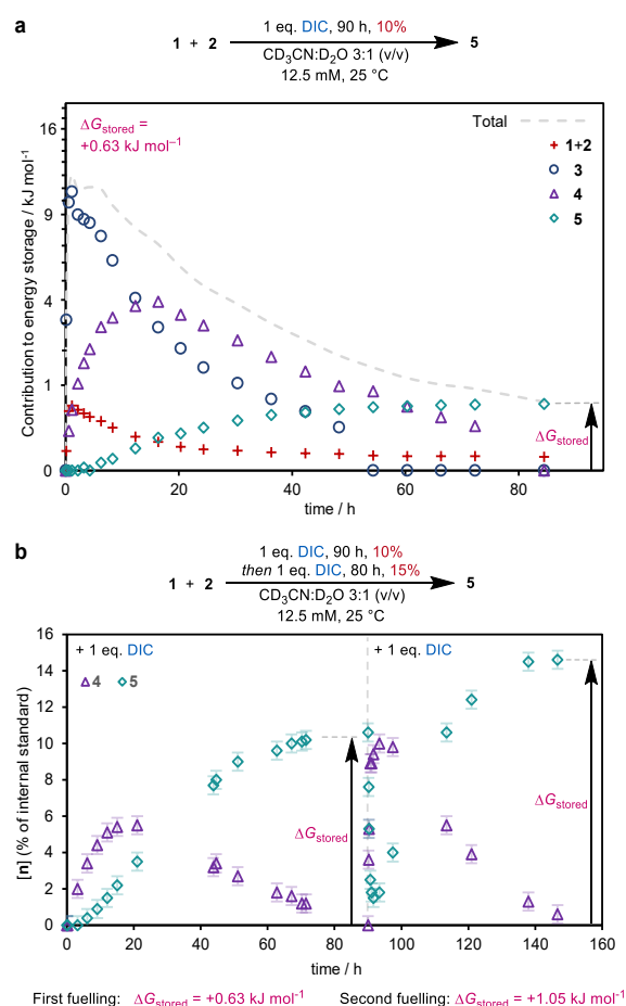
Fig 3 | Progressive work and energy storage. a The contribution of each species to the energy stored in the out-of-equilibrium reaction network. 54 The vertical axis is non-linear, increasing in increments of
