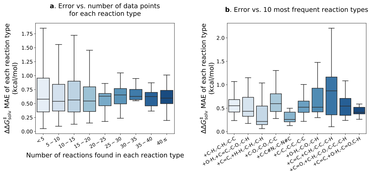
Figure 7: The results of the fine-tuned model with no additional feature on the pre-training test set reaction split. (a) Distribution of the \Delta\Delta G_{\text{solv}}^{\ddagger} MAE categorized by the number of training reaction data found in each reaction type. (b) Distribution of the \Delta\Delta G_{\text{solv}}^{\ddagger} MAE for the 10 most frequent reaction types. The reaction type is specified by the bond changes. For example, +C-H,-C-H,-C-C indicates that one carbon-hydrogen bond is formed, one carbon-hydrogen bond is broken, and one carbon-carbon bond is broken. Outliers are not shown in the plots.
