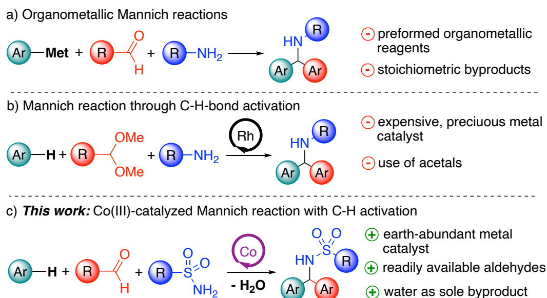
Scheme 1. Mannich-Type Reactions
