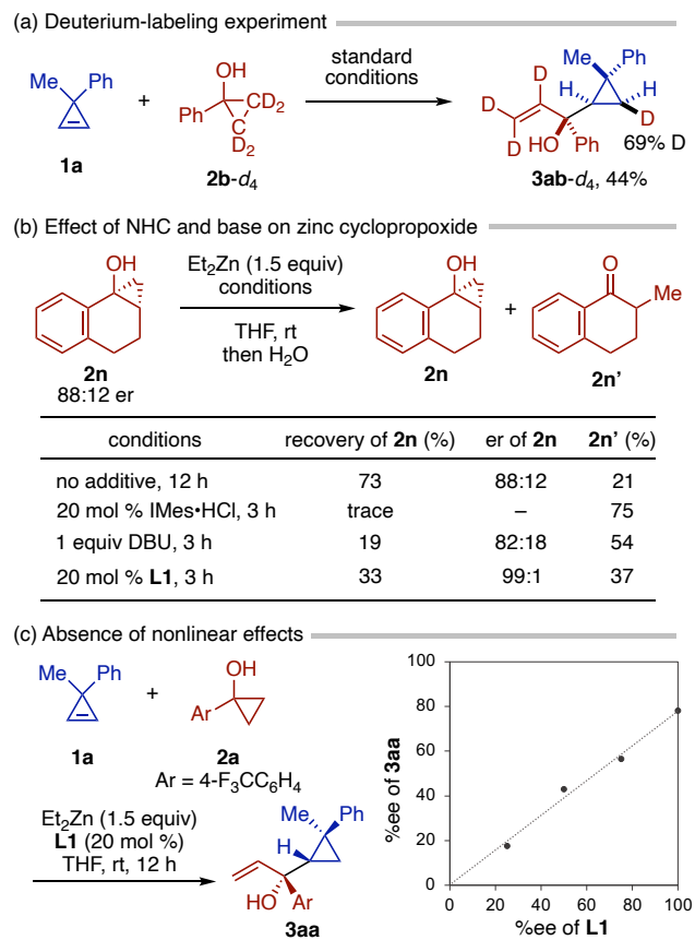
Figure 1. Mechanistic experiments. (a) Reaction of deuterium-labeled cyclopropanol. (b) Effect of NHC and base on the decomposition of zinc cyclopropoxide. (c) Examination of nonlinear effects in the reaction using L1 .
