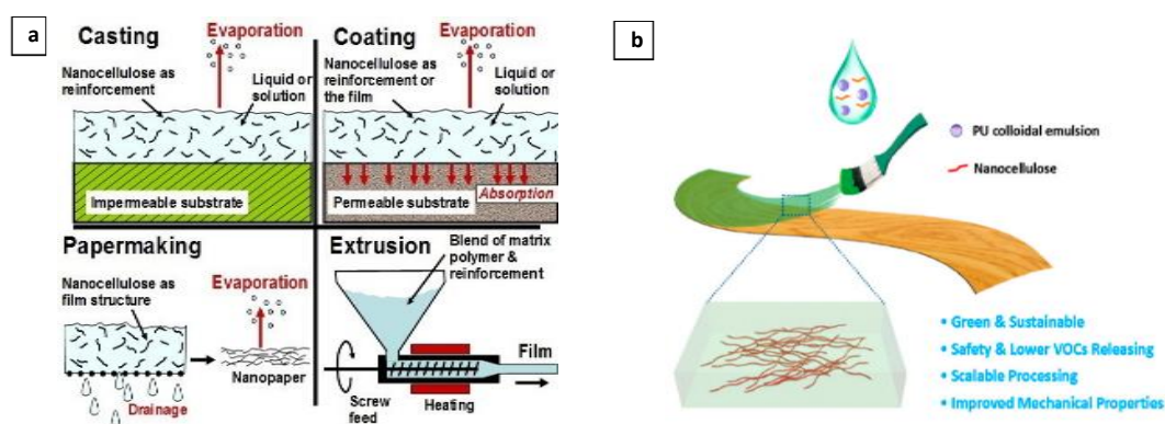
Figure 1. a) Schematic illustrating the four popular ways to make nanocellulose-containing films that are thin, presenting variations in liquid withdrawal[50]. b) nanocellulose-reinforced water-related polyurethane wood coating schematics[51]
