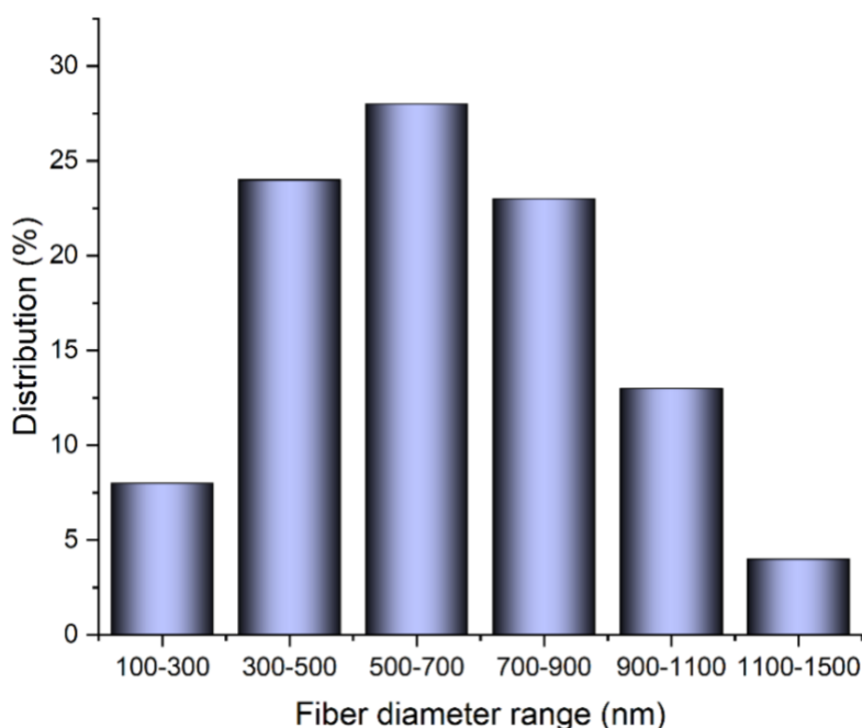
Figure 4. Fiber diameter distribution obtained from SEM micrographs of the copolymer, using Image J software.
