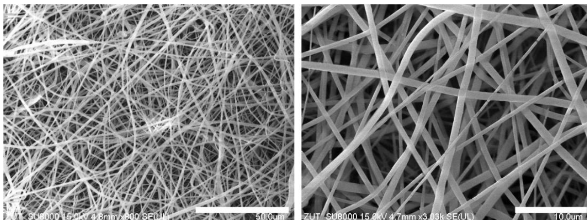
Figure 3. SEM micrographs of the obtained fibers from PDF-DLF copolymer using \text{CHCl}_3 as the solvent with 30% wt/vol% concentration.
