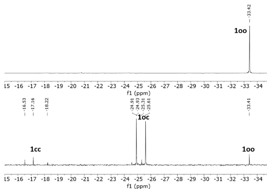
Fig. 2 ^{31}\text{P}\{^1\text{H}\} NMR spectra (121 MHz, toluene- d 8 ) of 1oo (top) and the PSS@365 nm (bottom), where partial DTE photocyclization produces a mixture of oo , oc and cc isomers.
