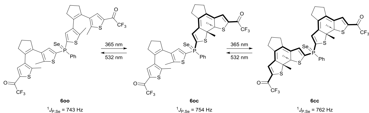
Scheme 3 – Photoisomerization-induced variation of ^1J_{P,Se} in the 00 , 0c and cc isomers of phosphine selenide 6 .
