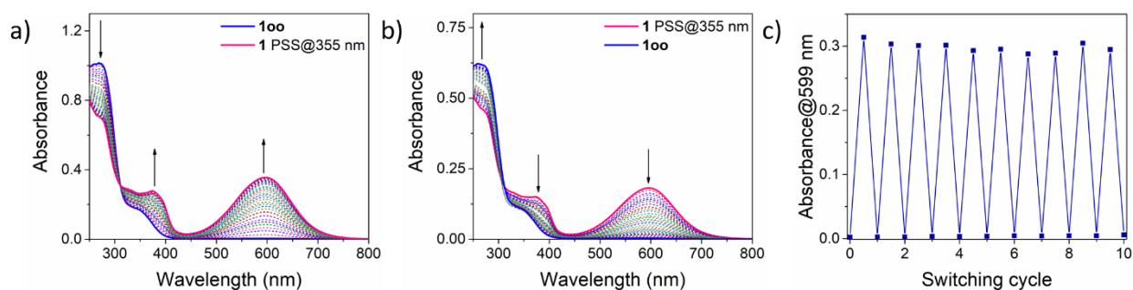
Fig. 1 Photochemical properties of 1 in cyclohexane solution. a) Variation of the UV-vis absorption spectrum of 1oo ( c = 3.12 \cdot 10^{-5} M) upon irradiation at \lambda_{\text{exc}} = 355 nm until a photostationary state is obtained (PSS@355 nm). b) Variation of the UV-vis absorption spectrum of PSS@355 nm for 1 ( c = 1.83 \cdot 10^{-5} M) upon irradiation at \lambda_{\text{exc}} = 532 nm until the initial spectrum of 1oo is recovered. c) Variation of the ring-closed absorbance of 1 ( c = 2.39 \cdot 10^{-5} M) in the visible region ( \lambda_{\text{exc}} = 599 nm) upon 10 consecutive photoswitching cycles with UV and visible light ( \lambda_{\text{exc}} = 365 and 520 nm).
