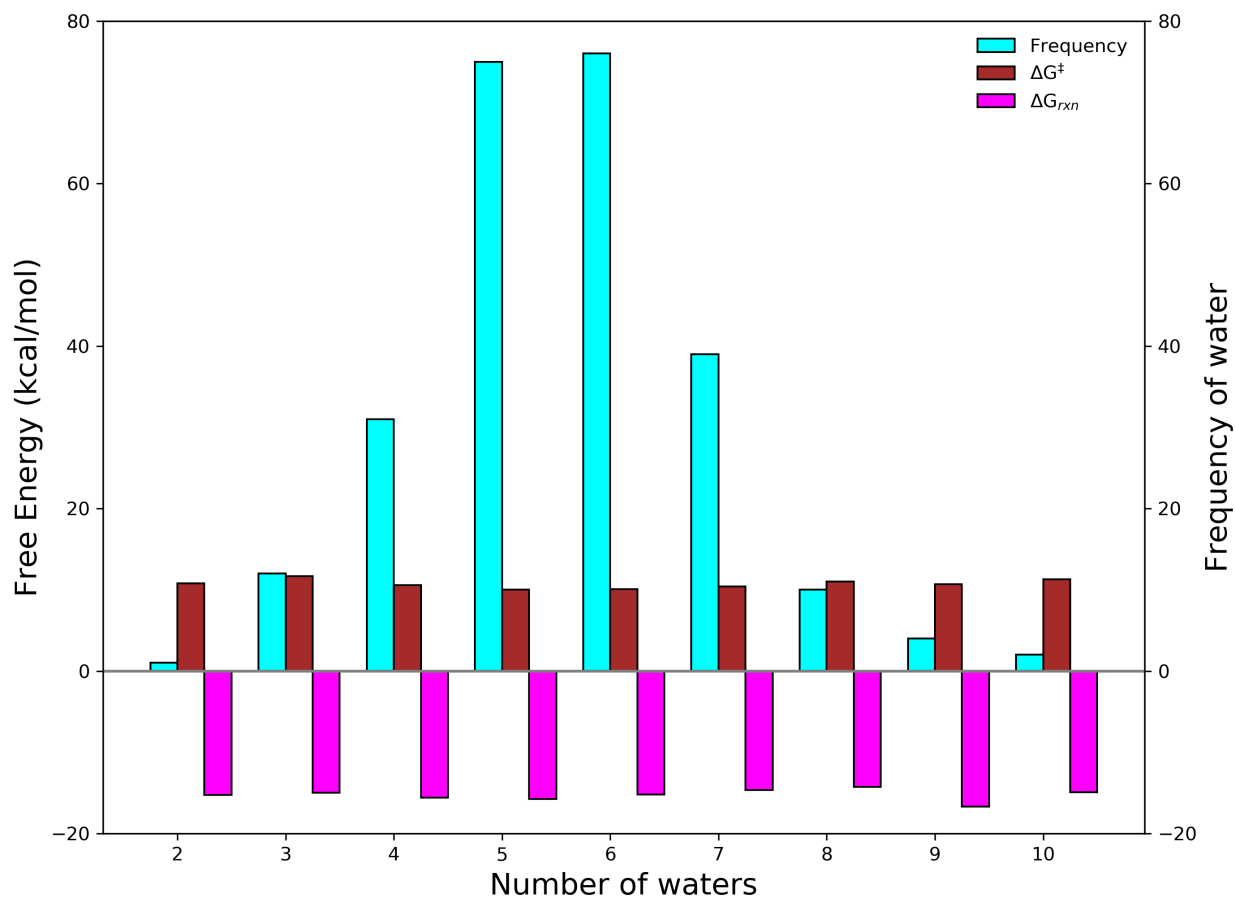
Figure 7: Mean activation free energy (brown), reaction free energy (magenta), and number of QM-cluster models with a given number of explicit water molecules (cyan) identified as having interatomic contacts with the chorismate for the 250 QM-cluster models built from selected MD frames.
