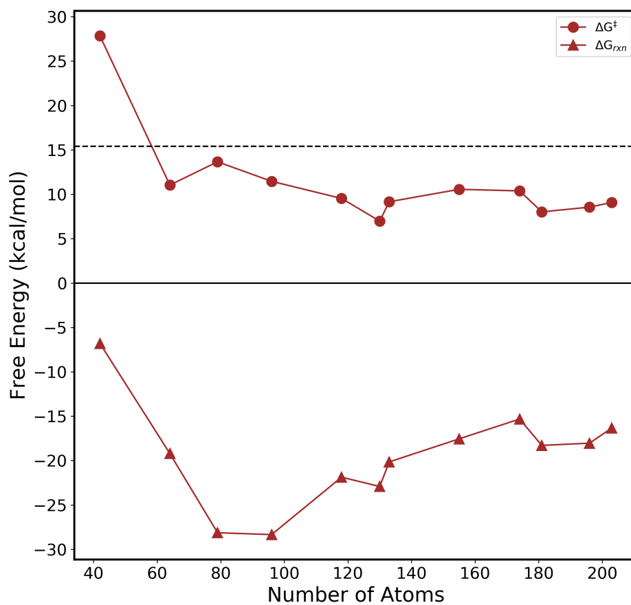
Figure 2: Kinetics and thermodynamics of the iteratively grown QM-cluster models using the probe ranking scheme. Computed \Delta G^\ddagger values are represented by circles and \Delta G_{rxn} values by triangles. The black dashed line shows the experimental \Delta G^\ddagger value from reference. 86
