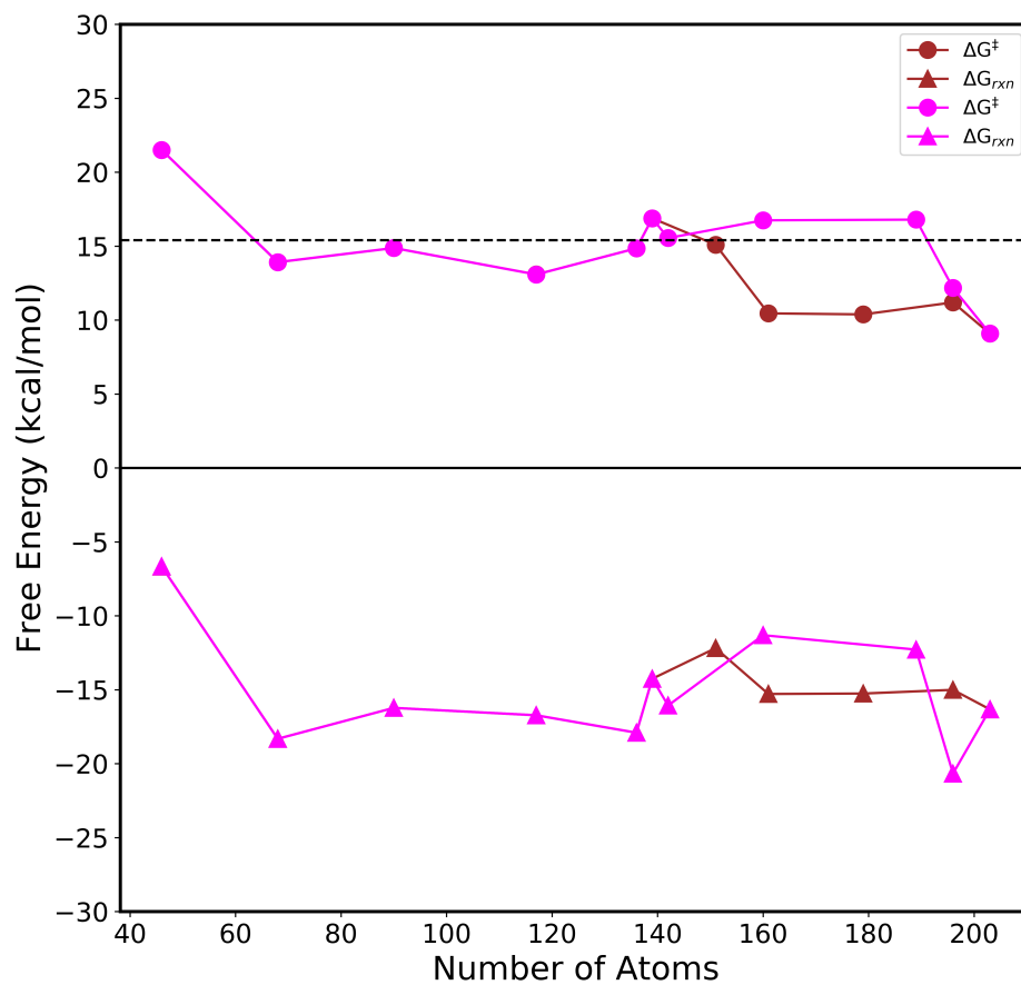
Figure 4: Kinetics and thermodynamics of the iteratively grown QM-cluster models using the F-SAPT ranking scheme. Computed \Delta G^\ddagger values are represented by circles and \Delta G_{rxn} values by triangles. The signed ranking order is given in magenta, while the unsigned ranking order is given in brown. The black dashed line shows the experimental \Delta G^\ddagger value from reference. 86
