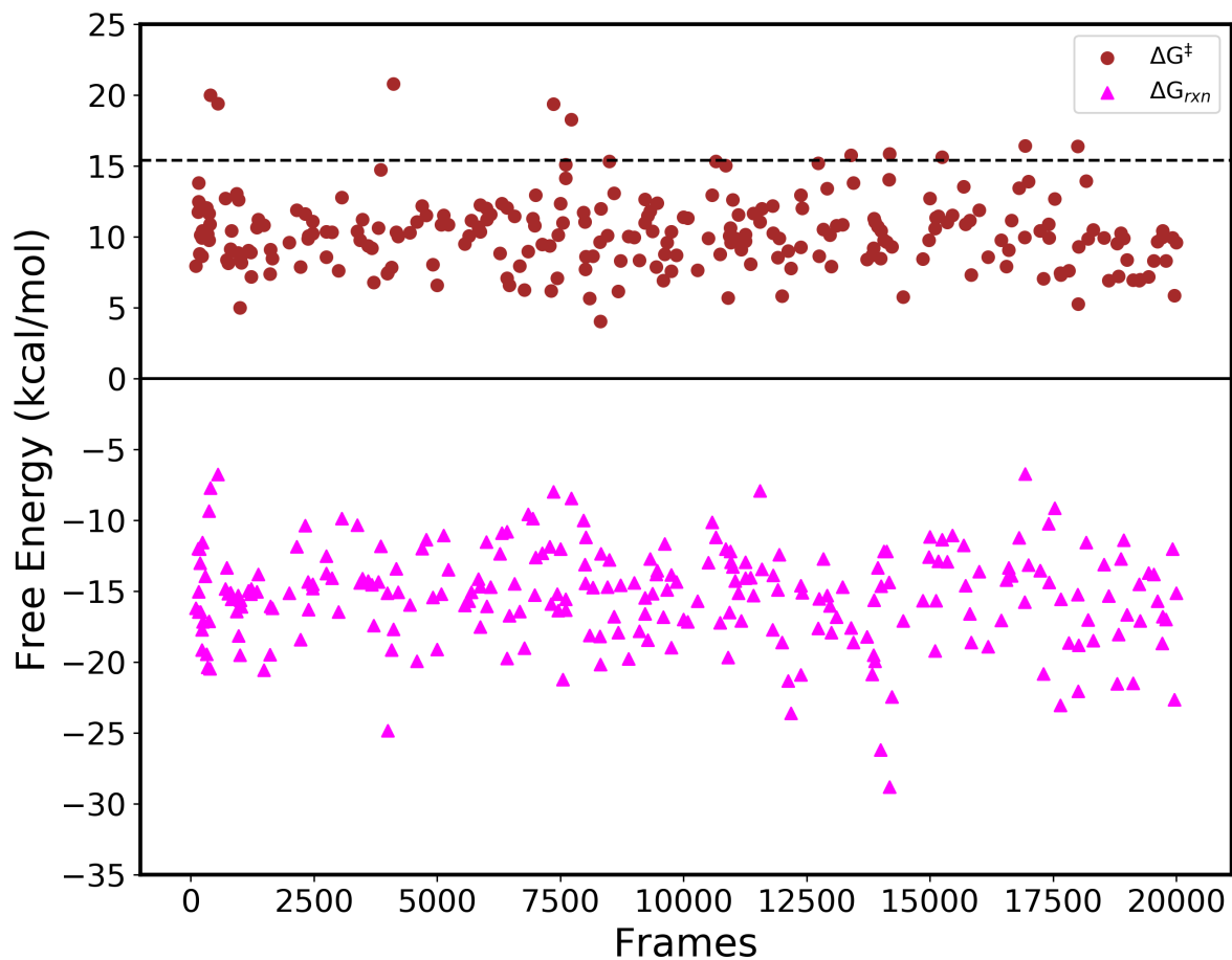
Figure 5: Computed values of \Delta G^\ddagger (circle) and \Delta G_{rxn} (triangle) for the 250 maximal QM-cluster models plotted against the select frame number (each representing a time scale of 1 ps). The black dashed line at the top is the experimental value from reference. 86
