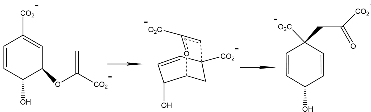
Scheme 1: Schematic representation of the Claisen rearrangement of chorismate to prephenate
