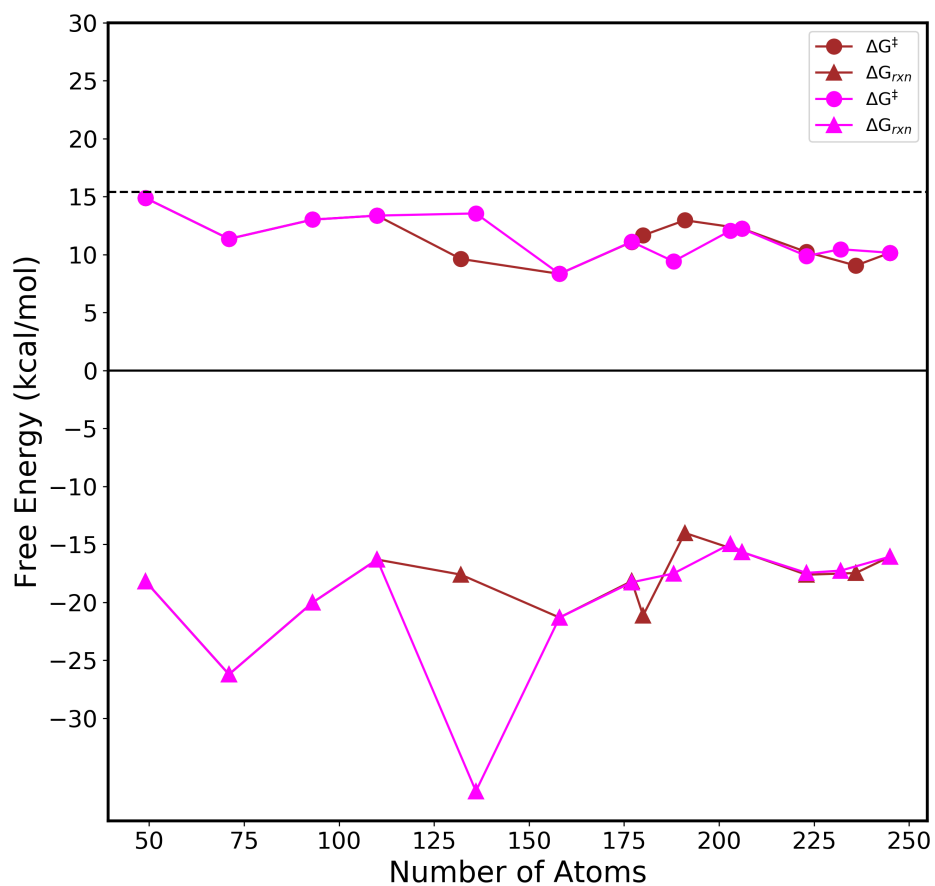
Figure 3: Kinetics and thermodynamics of the iteratively grown QM-cluster models using the arpeggio ranking scheme. Computed \Delta G^\ddagger values are represented by circles and \Delta G_{rxn} values by triangles. The original ranking is given in magenta, while values from the tie-breaking scheme are given in brown. The black dashed line shows the experimental \Delta G^\ddagger value from reference. 86
