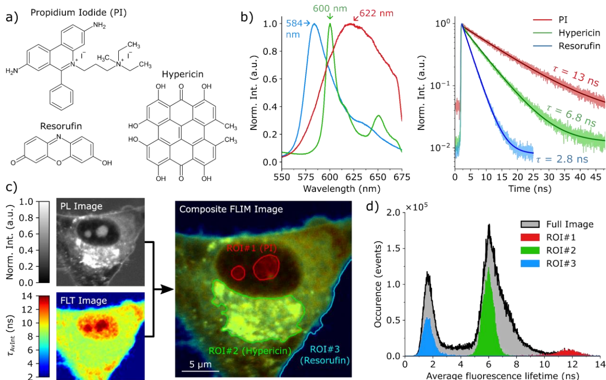
Figure 1: Characterization of hypericin-induced PDT in single glioma cells. a) The chemical structures of hypericin, resorufin and PI. b) The fluorescence spectra and fluorescence decay curves for hypericin (green), resorufin (blue) and PI (red) in medium solution, acquired by excitation with a 405 nm laser. The respective fluorescence lifetimes \tau are 2.8 ns for resorufin, 6.8 ns for hypericin and 13 ns for PI. c) depicts a composite FLIM image of a single glioma cell in an early PDT stage. The composite FLIM image's color is given by the FLT recorded at each pixel, while the brightness is determined by the PL intensity. Three regions of interest (ROI) are indicated in c), where the fluorescence signal is dominated by one specific dye, [ROI#1 (nucleoli): PI, ROI#2 (ER): hypericin, ROI#3 (medium): resorufin]. The occurrence histograms in d) display the number of photons that are associated with a certain average FLT for the full image (black) and the ROIs in c).
