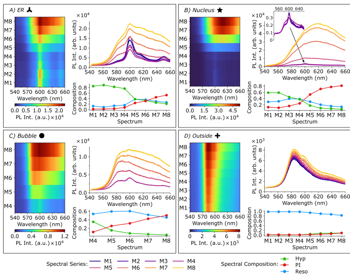
Figure 4: Spatially resolved fluorescence spectra recorded on the locations of the corresponding markers indicated in Fig. 3. All spectra were recorded at the same wavelength and laser power used for the FLIM image acquisition ( \lambda_{\text{exc}} = 405 \text{ nm} , I = 7.8 \mu\text{W}/\mu\text{m}^2 ) with an integration time of one second.
