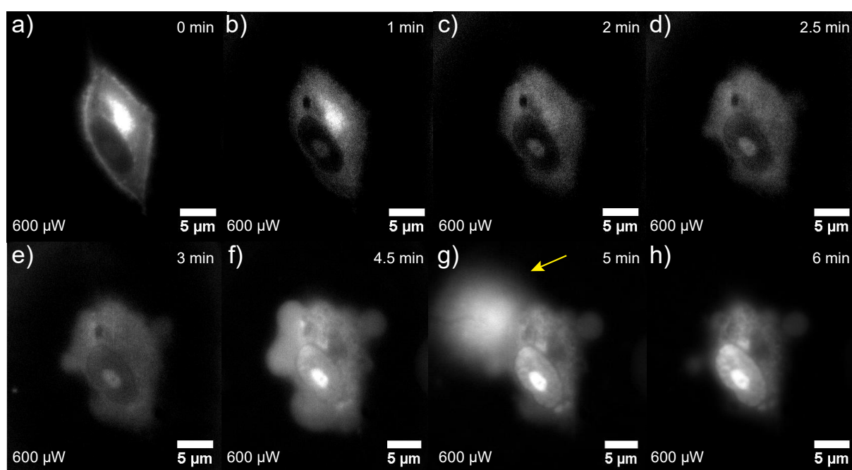
Figure 5: Series of widefield fluorescence images showing the effect of hypericin-induced PDT on a single glioma cell incubated with hypericin and PI. Different stages of cell damage are deducible, including rounding of the cell body (b-d), membrane bleb formation (d-f), explosive membrane rupture (g, yellow arrow), and finally cell death (h). The membrane rupture is accompanied by the release of cytoplasm content into the extracellular environment. The overall recorded fluorescence intensity is continuously increasing, which results from more PI entering the damaged cellular body and binding to RNA/DNA
