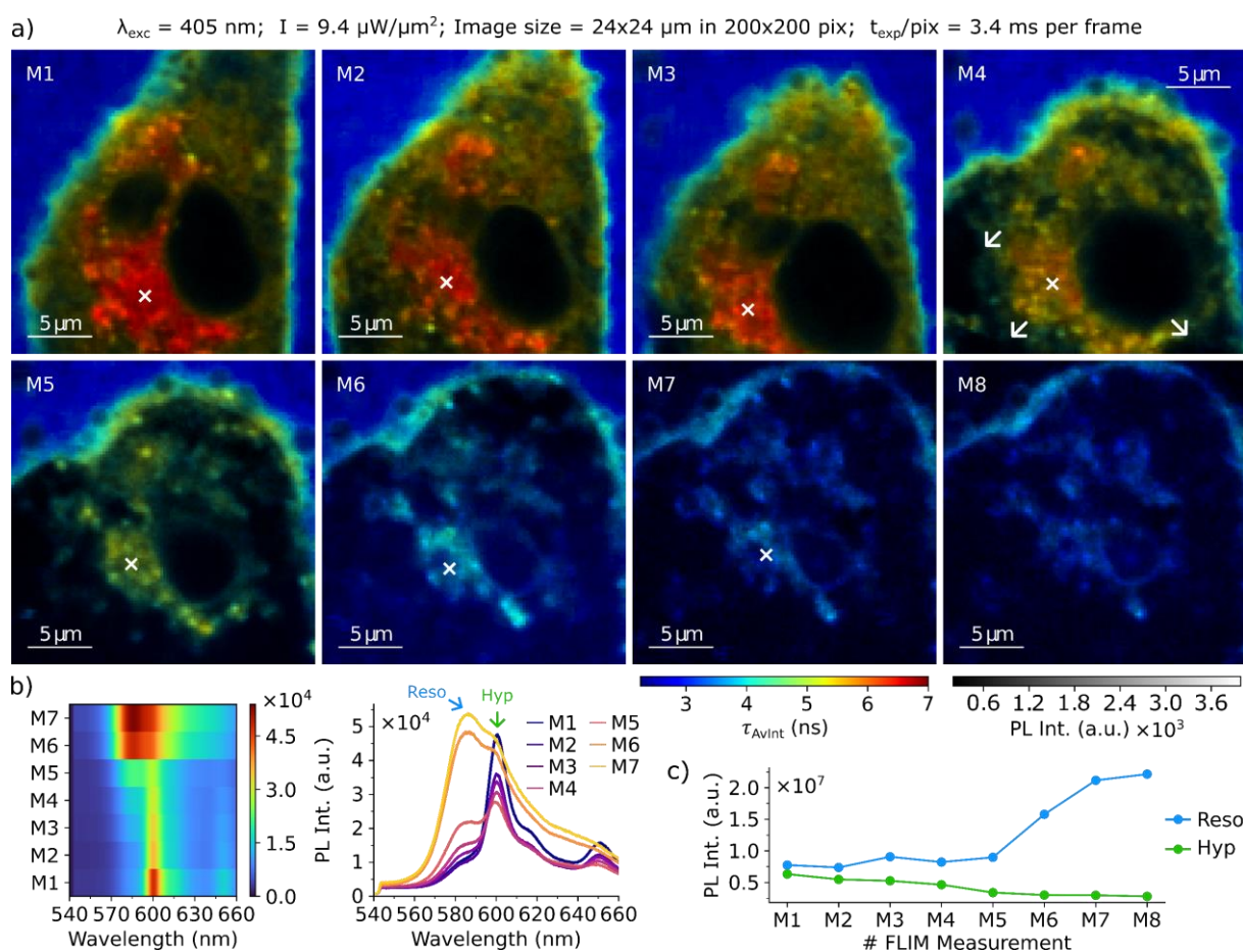
Figure 2: a) Composite FLIM image series of a single glioma cell after hypericin incubation and resorufin conversion. Cell contraction and rounding can be observed in M1 to M3, together with a decrease of hypericin PL intensity. Formation of protuberances of the cellular membrane close to the ER is visible in M4. Further swelling until rupture of the cell membrane occurs between M5 and M8. b) Series of fluorescence spectra acquired in the cell's ER at the locations marked by the white cross in M1-M7. c) Evolution of the overall fluorescence intensities of hypericin and resorufin recorded in each image of the series. The acquisition parameters of the imaging series are displayed on top of the Figure.
