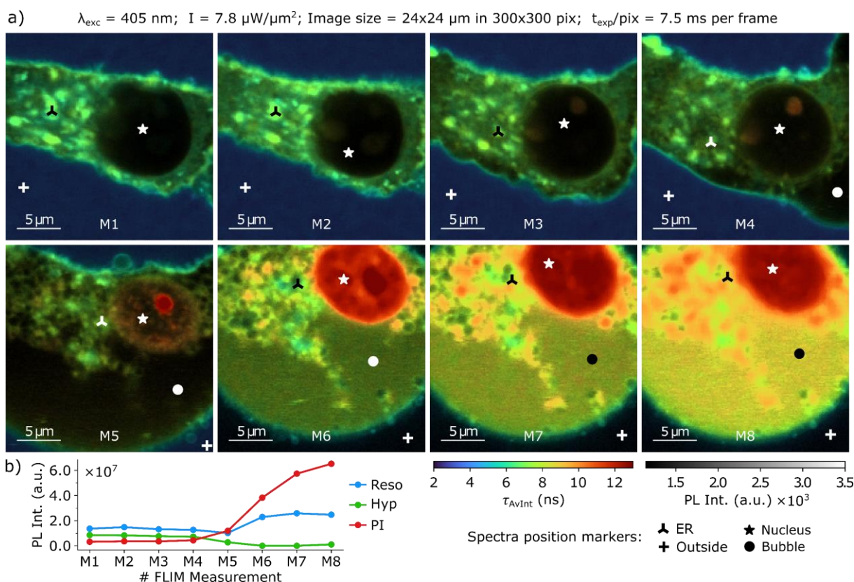
Figure 3: a) Composite FLIM image series of a single glioma cell after hypericin incubation, PI supplementation, and resorufin conversion. b) Evolution of the overall fluorescence intensities of hypericin, resorufin and PI recorded in each image of the series. The fluorescence spectra acquired at the position markers are displayed in Fig. 4. The acquisition parameters of the imaging series are displayed above.
