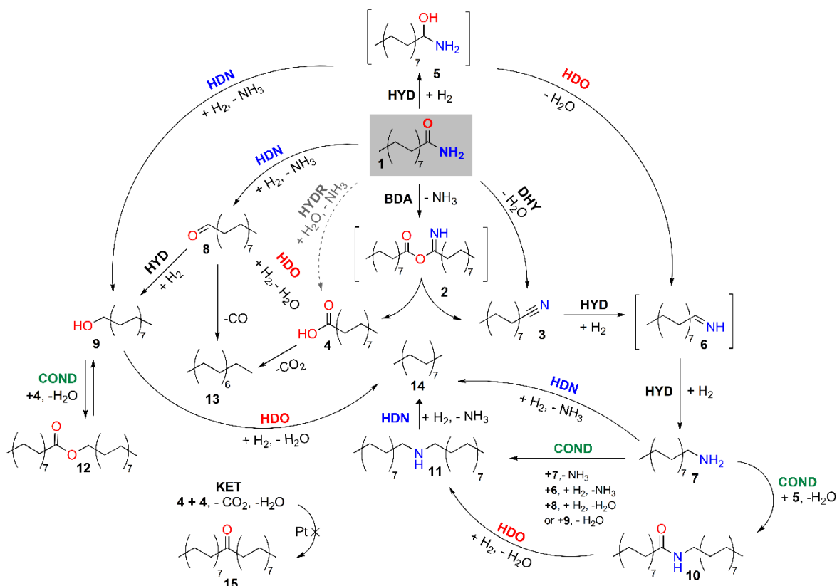
Scheme 1. Proposed reaction network for the hydrotreatment of C16 amide. Indicated compounds: 1 C16 amide, 2 C32 isoimide, 3 C16 nitrile, 4 C16 acid, 5 C16 hemiaminal, 6 C16 imine, 7 C16 amine, 8 C16 aldehyde, 9 C16 alcohol, 10 C32 amide, 11 C32 amine, 12 C32 ester, 13 C15 paraffin, 14 C16 paraffin, and 15 C31 ketone. The bimolecular deammoniation (BDA), direct dehydration (DHY), hydrogenation (HYD) and hydrolysis (HYDR) of the C16 amide, and the condensation (COND), HDO and HDN reactions of the intermediates have been indicated. The bimolecular ketonization of the C16 acid (KET) only occurred over the bare supports. The reaction network has been adapted and extended from a previous study conducted by Verkama et al. 16
