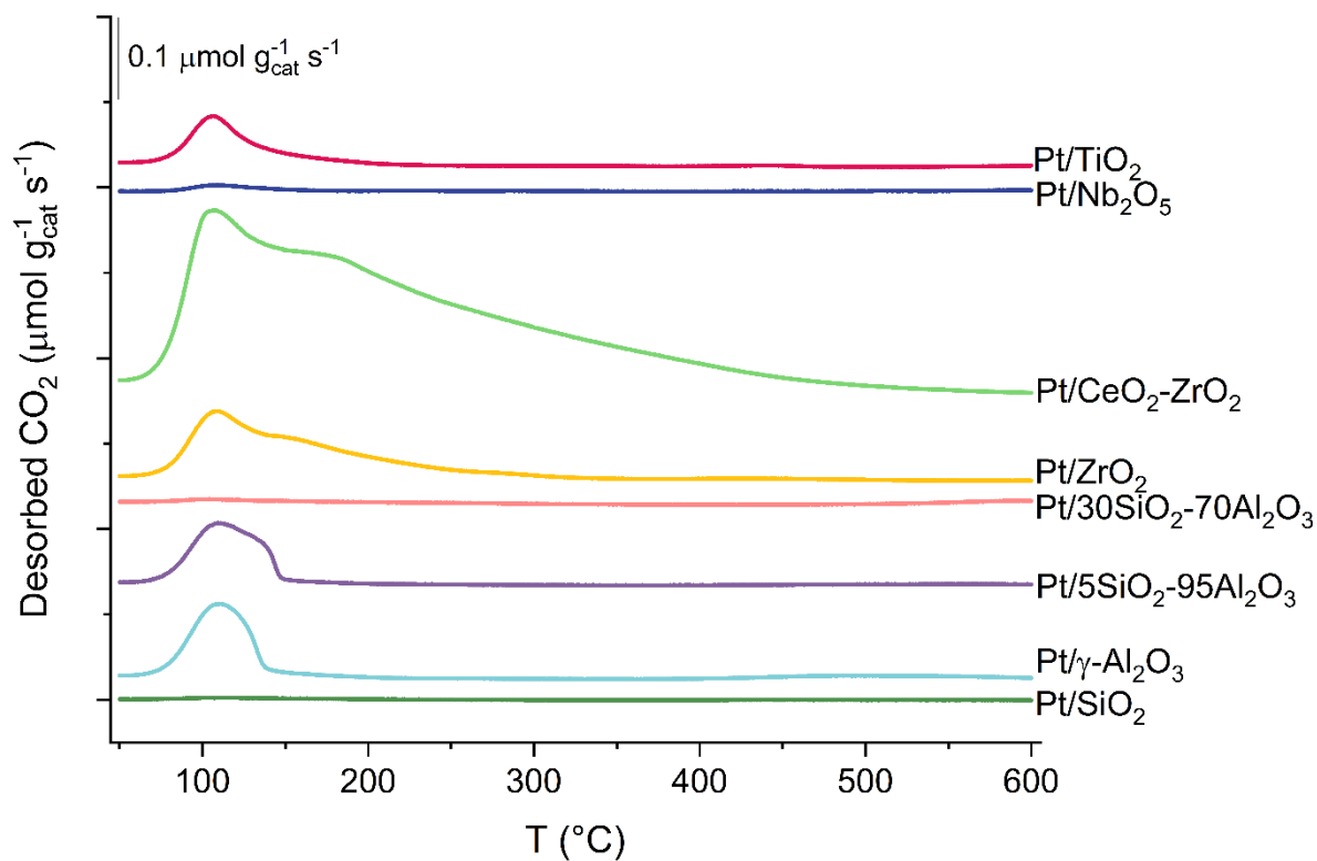
Figure S8. CO 2 -TPD profiles of the supported Pt catalysts. The catalysts were reduced at 350 °C for 60 min before the CO 2 saturation at 50 °C.
