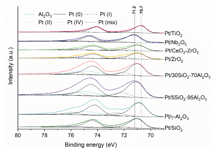
Figure 1. High-resolution X-ray photoelectron spectra of the Pt 4f/Al 2p region of the supported Pt catalysts. The catalysts were reduced ex situ at 350 °C before the measurements.
