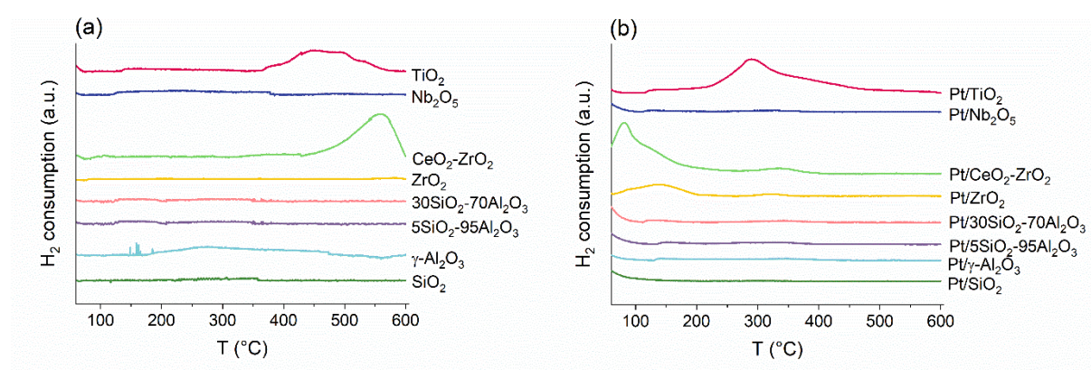
Figure 2. H 2 -TPR profiles of (a) the bare supports and (b) the calcined supported Pt catalysts.
