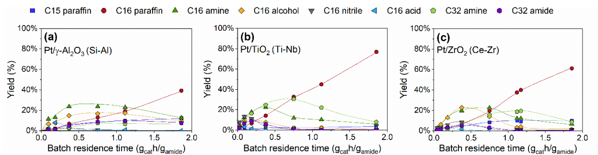
Figure 5. Product distribution as a function of batch residence time for (a) Pt/ \gamma -Al 2 O 3 , (b) Pt/TiO 2 , and (c) Pt/ZrO 2 in the hydrotreatment of C16 amide at 300 °C and 80 bar H 2 . The 60-min reference experiments of Figure 4 correspond to a batch residence time of 0.37 g cat h/g amide . The lines have been added to guide the eye.
