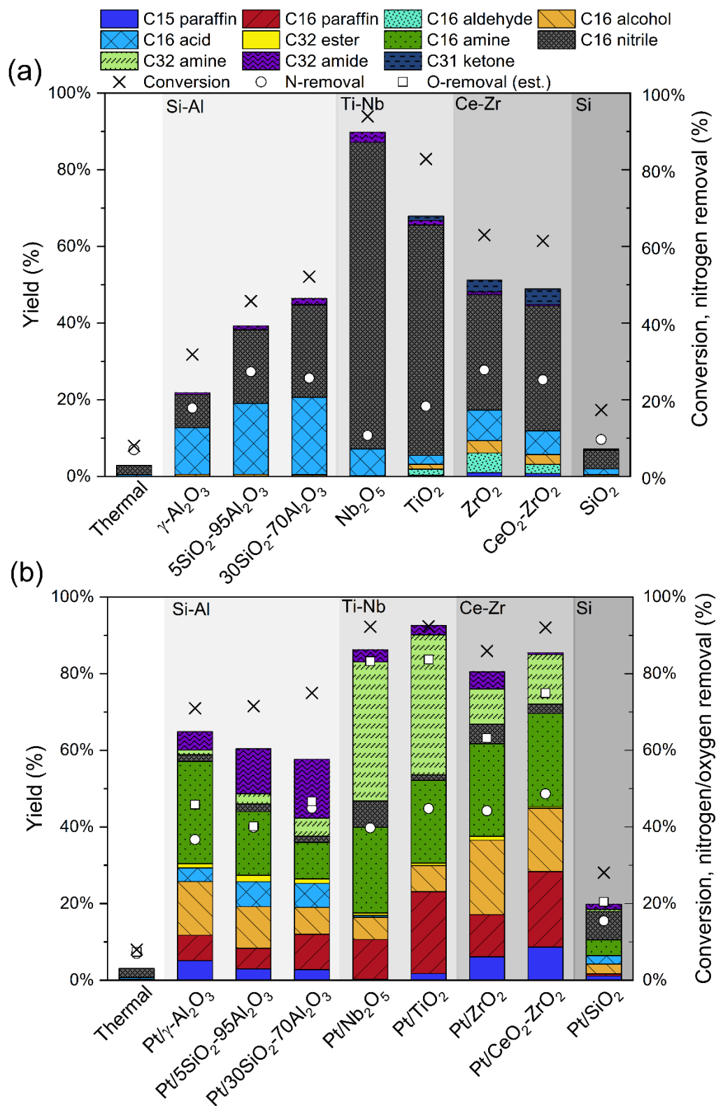
Figure 4. Product distribution, conversion (X), and nitrogen removal (O) of the C16 amide hydrotreating experiments on (a) the bare supports and (b) the supported Pt catalysts. The oxygen removal (□) of the supported Pt catalysts was derived from the product distribution, while the nitrogen removal was obtained from the total nitrogen content analysis. The materials have been grouped according to their Lewis acid site strength. Reaction conditions: 300 °C, 80 bar H 2 , 60 min ( \tau=0.37 \text{ g}_{\text{cat}}\text{h}/\text{g}_{\text{amide}} ).
