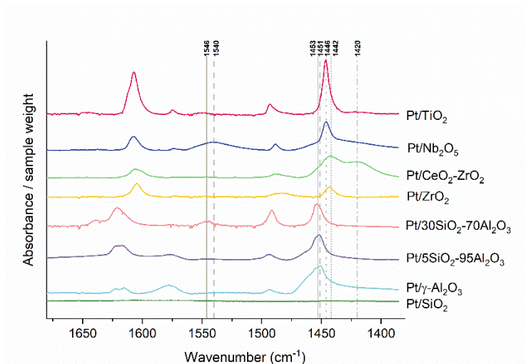
Figure 3. Transmission FTIR spectra for the pyridine-saturated supported Pt catalysts, with the background and spectra of the clean samples subtracted. The spectra were collected at 170 °C. The vibration bands characteristic for pyridine adsorbed on Brønsted acid sites (1540 and 1546 \text{cm}^{-1} ) and Lewis acid sites (1442–1453 \text{cm}^{-1} ) have been indicated with vertical lines.
