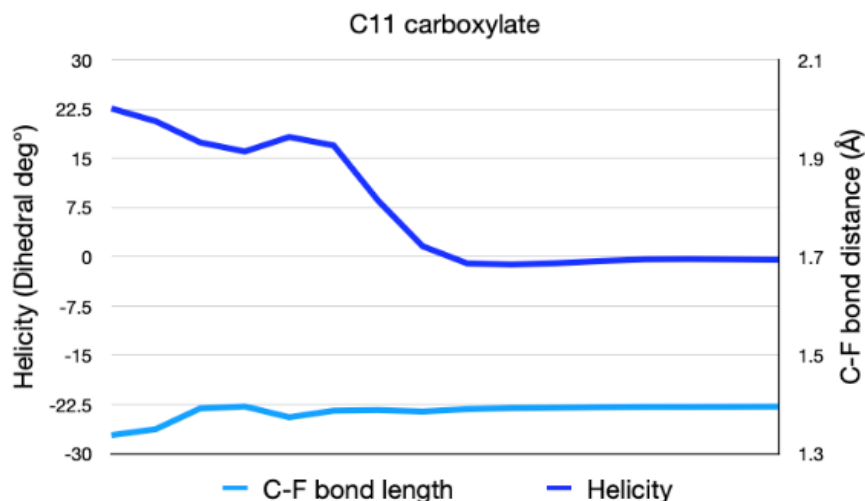
Figure 7: The results of simulated electron capture on C10 – C12 perfluorinated carboxylates on the helicity and terminal C-F bond length. Each of these longer-chain molecules are able to stabilize in the elongated and straightened conformation without defluorination due to the larger number of carbons supporting the additional charge and the entropy gained by the flexibility.
