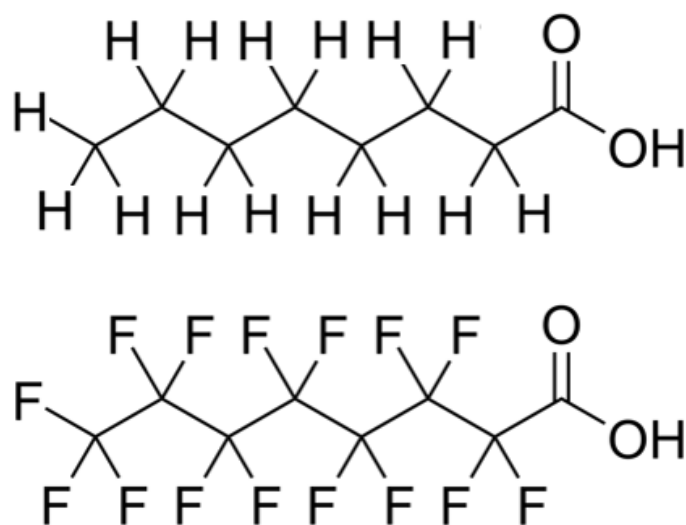
Figure 1: Structural formulae of octanoic acid (top) and perfluorooctanoic acid (bottom). The layout seems to convey that the two molecules share the same linear trans conformation; however, these are connectivity schematics only and contain zero geometric information.
