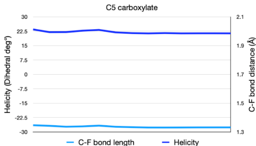
Figure 5: The results of simulated electron capture on C5 perfluorinated carboxylate on the helicity and terminal C-F bond length, result is typical for C4-C6. Each of the short-chain molecules stabilize the -2 state without inducing a change in helicity or fluoride dissociation.
