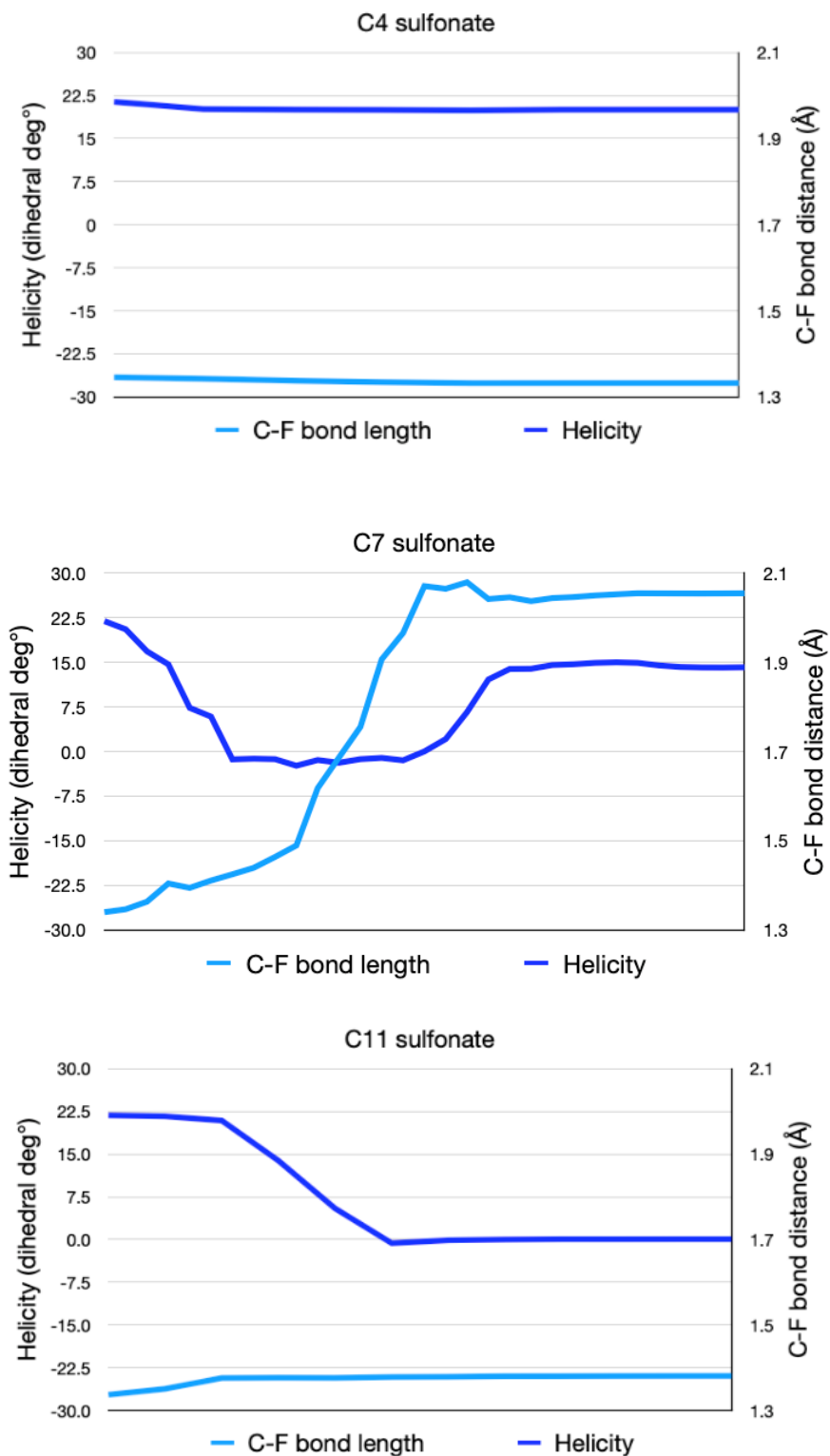
Figure 8: Typical charts of helicity and C-F bond length in short (C4 only), middle (C5-C8), and long (C9-C12) perfluorinated sulfonates. The sulfonate follows the identical trend as the carboxylate although the location of the segmentation has changed as a result of the change in functional group.
