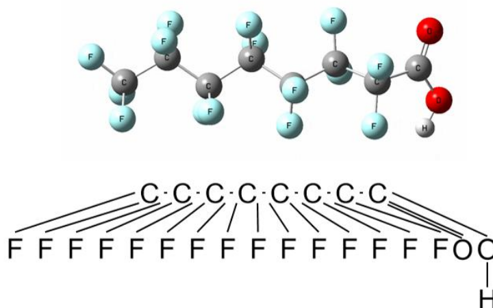
Figure 2: A picture of an optimized model of PFOA (top) and a second structural formula of PFOA (bottom). The picture depicts molecular connectivity and geometry and thus comparatively greater information content than the Fig. 1 structural formula, despite visual similarity. By contrast, the information content of the PFOA structural formula shown here is identical to that held by the more typical layout in Fig. 1.
