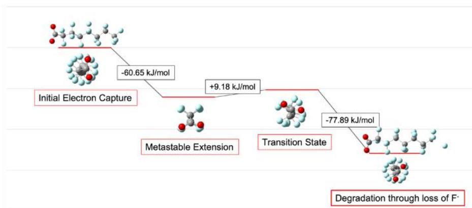
Figure 4: The relaxation pathway of PFOA after the capture of an additional electron. Initially, lengthening C-C bonds cause a loss of helicity and the molecule relaxes into a straight and extended conformation wherein C-F bonds remain intact. Only regaining the compact, helical compact form delivers enough of an advantage to afford the cost of C-F dissociation.
