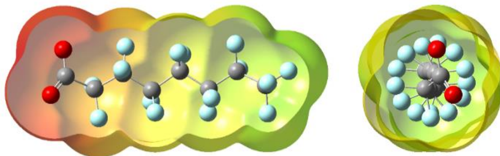
Figure 3: Side and end views of a perfluorooctanoate model with charge on the electron density surface shown in red (negative) at the carboxylate head group progressing toward green (neutral) at the tail. Carbon is shown in grey, fluorine in blue, oxygen in red. The helicity imposed by fluorine-fluorine repulsion is evident.
