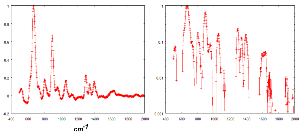
Fig. 1: SERS data of L-Cysteine (data courtesy Sherman et al., 2020). On the right, the data with log scale y-axis (semi log scale). The semi log scale helps us to identify several band ranges. The endpoints of frequency ranges are easily determined by their lowest intensities. Negative data are not represented in the semi log scale.
