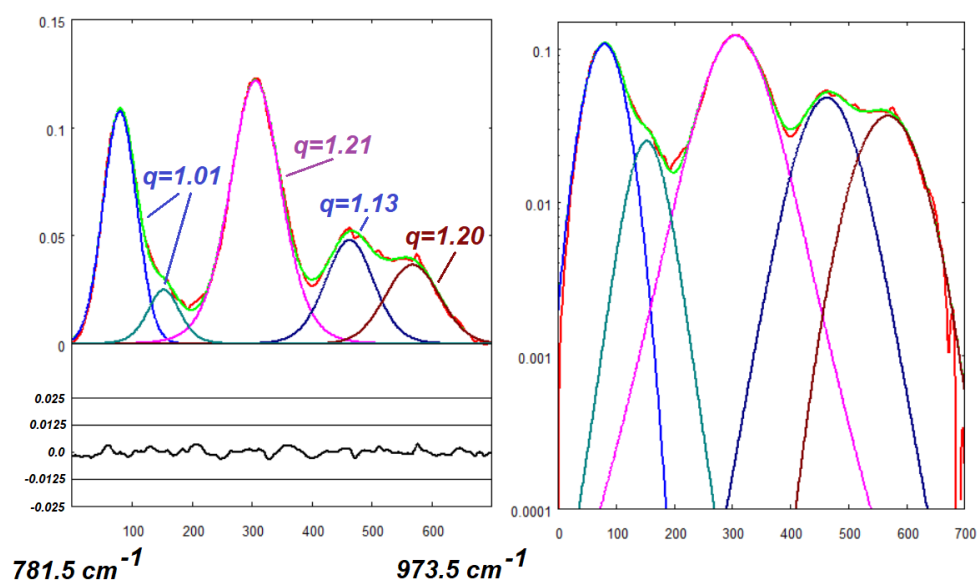
Fig. 9: Fitting (green) onto data (red) of Cysteamine (data Sherman et al., 2020). Frequency ranges from 781.5 to 973.5 \text{cm}^{-1} (see Fig.7). For the deconvolution, five q-Gaussians are used (values of the q-parameters are given in the figure). The q-Gaussian centre positions are 803.5, 823.5, 865.5, 908 and 936.5 \text{cm}^{-1} , from left to right.
