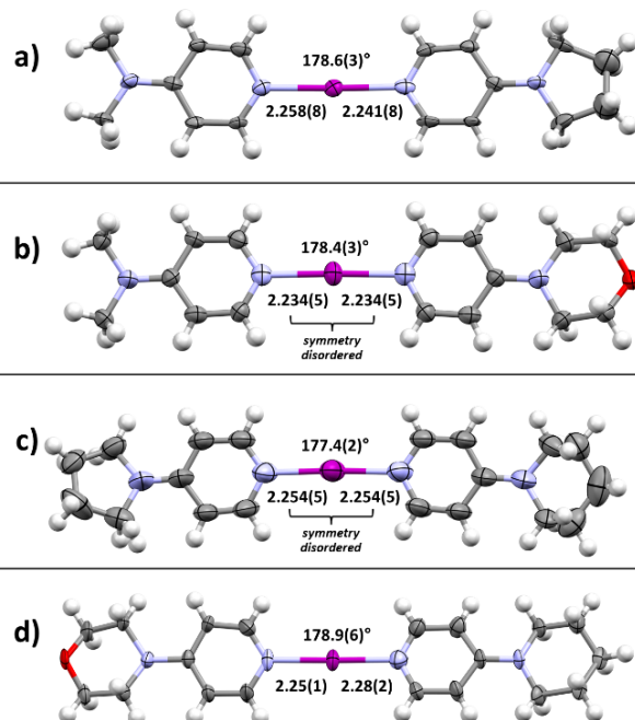
Figure 4. X-ray crystal structures of asymmetric iodine(I) complexes 4 : (a) [I(DMAP)(PPY)] + ( 4ab ), (b) [I(DMAP)(MPY)] + ( 4ac ), (c) [I(PPY)(PiPY)] + ( 4bd ), (d) [I(MPY)(PiPY)] + ( 4cd ) (thermal ellipsoids shown at 50% probability level; anions, minor disordered positions, and solvates omitted for clarity; distances are given in Å).
