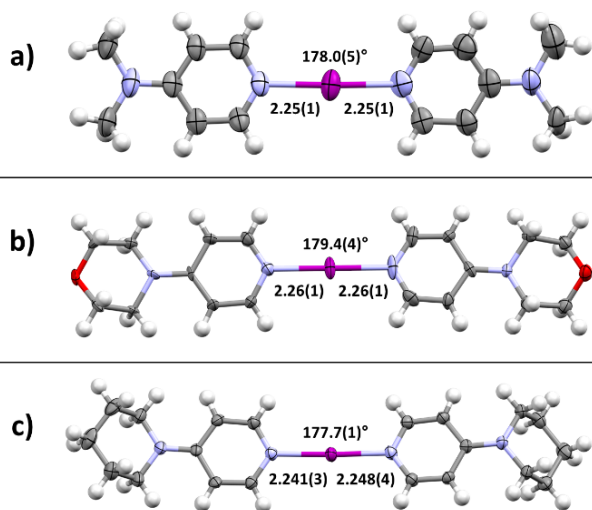
Figure 3. X-ray crystal structures of symmetric iodine(I) complexes 4 : (a) [I(DMAP) 2 ] + ( 4a_1 ), (b) [I(MPY) 2 ] + ( 4c_1 ), (c) [I(PiPY) 2 ] + ( 4d ) (thermal ellipsoids shown at 50% probability level; anions, minor disordered positions, and solvates omitted for clarity; distances are given in Å).
