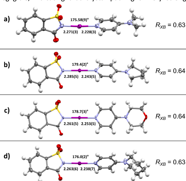
Figure 2. X-ray crystal structures of XB complexes between NISac and (a) DMAP ( 3a ), (b) PPY ( 3b ), (c) MPY ( 3c ), (d) PiPY ( 3d ), and corresponding average reduction ratios R_{XB} (thermal ellipsoids shown at 50% probability level; distances are given in Å).
