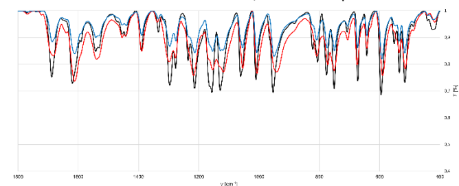
Figure 5. Comparison of IR spectra around 1800-400 \text{cm}^{-1} obtained in the mechanochemical synthesis of XB complex 3a . Black: XB complex 3a from solution. Red: Neat grinding equal amounts of DMAP and NISac for 15 min. Blue: LAG (EtOAc) equal amounts of DMAP and NISac for 5 min.
