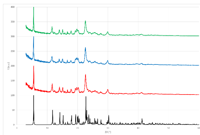
Figure 6. Comparison of PXRD patterns obtained in the mechanochemical preparation of symmetric iodine(I) complex 4a . 33 Black: Simulated PXRD pattern of symmetric iodine(I) complex 4a . Red: route A ( 3a and DMAP for 5 min under LAG (EtOAc) conditions). Blue: route B (two step synthesis under LAG (EtOAc) conditions). Green: route C (grinding one equivalent of NISac and two equivalents of DMAP for 5 min under LAG (EtOAc) conditions).
