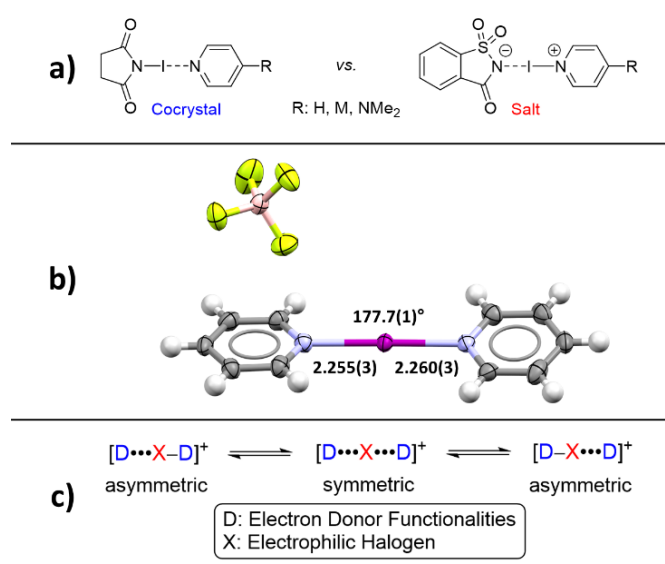
Figure 1. (a) Schematic representation of the co-crystal and "close-to-ionic" coordination mode in NISac based XB complexes. (b) Molecular structure of Barluenga's reagent (CCDC 202334; thermal ellipsoids shown at 50% probability level; distances are given in Å). 94–101 (c) Possible asymmetric and symmetric coordination modes of a three-center-four-electron halogen bond.
