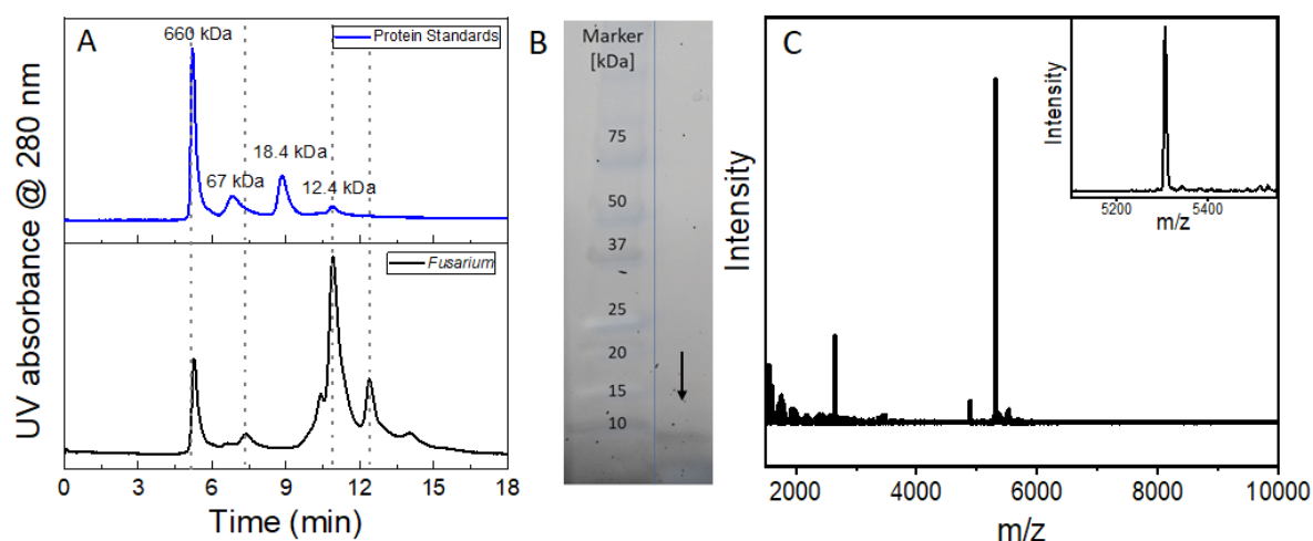
Fig. 4. Characterization of aqueous solutions of ice-affinity purified INs from F. acuminatum . (A) Separation of a protein standard and the ice-affinity purified F. acuminatum extract on a gel filtration column using a TSK G2000SWXL. The proteins were eluted with a 50 mM sodium phosphate, 0.3 M NaCl buffer, pH 7, at a flow rate of 1 mL/min. (B) SDS-PAGE gel electrophoresis of the ice-affinity purified F. acuminatum extract shows a weak band just below 10 kDa that is highlighted by an arrow (C) MALDI spectra of the ice-affinity purified sample show a dominant signal at ~5300, which is highlighted in the inset.
