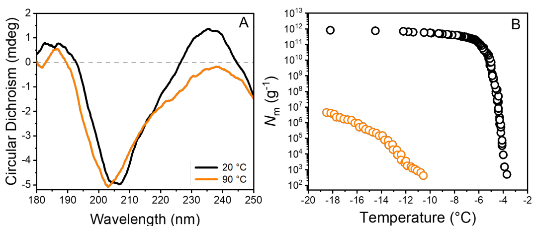
Fig. 2. Characterization of aqueous solutions containing ice-affinity purified INs from F. acuminatum . (A) The CD spectrum shows a maximum molar ellipticity at ~235 nm and a minimum at ~205 nm, and both signals are altered following heating to ~90 °C. (B) Effects of high temperature (98 °C) on the ice nucleation activity of F. acuminatum extract. Shown is the cumulative number of INs ( N_m ) per gram of mycelium plotted against the temperature. Data were obtained from Kunert et al. (10).
