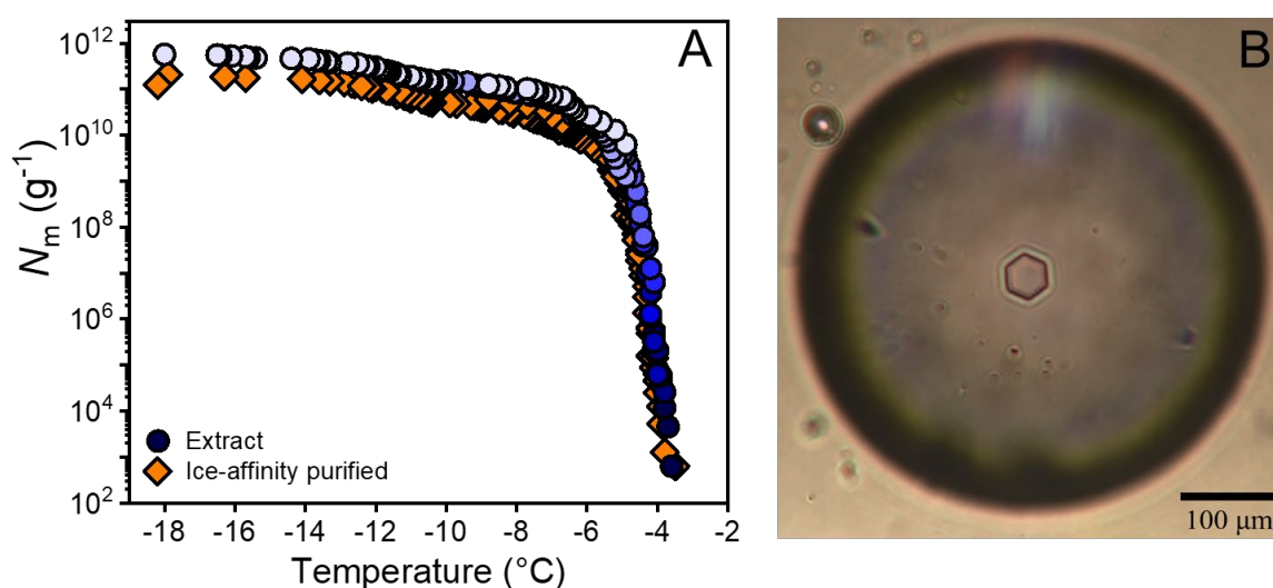
Fig. 1. Freezing experiments of aqueous extracts containing fungal ice nucleators from F. acuminatum . (A) Shown is the cumulative number of ice nucleators per unit mass of F. acuminatum ( N_m ) for extracts containing ice nucleators from spores and mycelial surfaces
