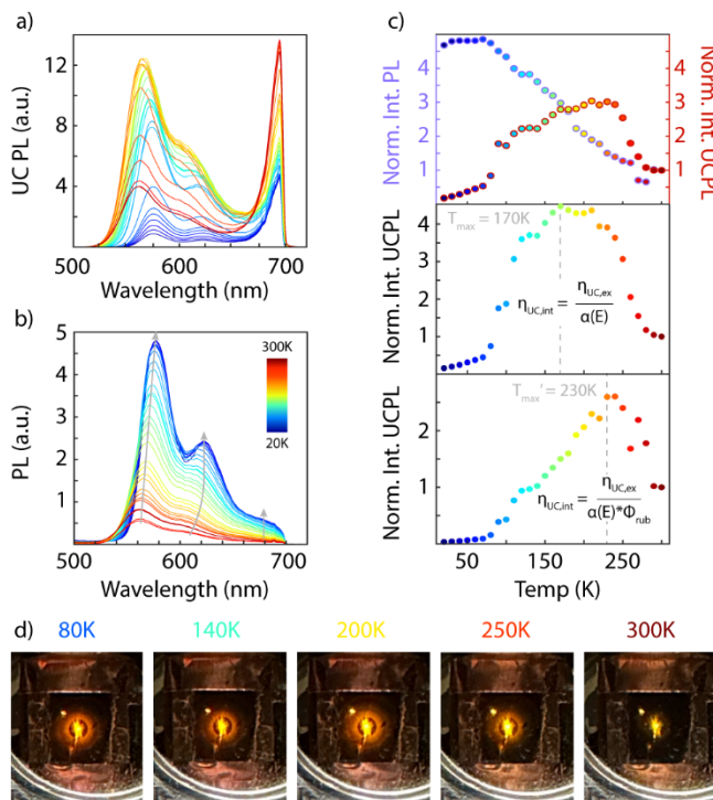
Figure 2: a) UCPL for the 100 nm MAFArub bilayer collected under 780 nm excitation while cooling from 300 K to 20 K where three spectra were collected at each temperature then averaged. b) Direct emission of the MAFArub bilayer under 405 nm excitation collected while cooling from 300 K to 20 K. A 700 nm short-pass filter was used to isolate dye emission. Three spectra were collected at each temperature then averaged. Grey arrows are included as guides to the eye. c) (top) Integrated direct (lavender) and upconverted (red) emission for the bilayer film. (middle) Integrated UCPL ( \eta_{UC,ex} ) normalized to the absorption overlap of the bilayer film with the excitation laser ( \alpha(E) ). Dashed grey line represents T_{max} = 170 K. (bottom) The absorption, normalized integrated UCPL spectra normalized by the quantum yield of rub under direct excitation, with the equation included. Here, T_{max} is 230 K, indicated via the dashed grey line. d) Photographs of the MAFArub bilayer under 780 nm excitation at select temperatures.
