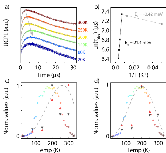
Figure 5: a) UCPL dynamics for the 100 nm MAFarub film for the specified temperatures. Each decay is normalized by the maximum and offset for clarity. The first four temperatures (300K to 140K) are fit to single exponential terms for the fall and rise components, while the 80 and 20 K lifetimes use a biexponential rise term to better account for an observed rapid rise in the first 200 ns. b) The triplet rise times are compared in an Arrhenius plot, where the four highest temperatures are linearly related with an activation energy of 21.4 meV associated with the energy barrier for an Arrhenius type hopping mechanism. The three lowest temperatures interestingly also feature a separate activation energy of -0.4 meV, indicating a transition to an energetically favorable Miller-Abrahams type regime. c) Normalized UCPL model following an inverse temperature dependence for the diffusion length, similar to triplet behavior observed previously in anthracene (dashed grey curve). 65 The dark grey triangles utilize experimental triplet decay lifetimes while the red triangles are triplet rise lifetimes. d) The same normalized UCPL compared with a similar diffusion model, however, instead compared using an empirical diffusion model (dashed grey curve) ( I_{UC} \propto k_{TTA} = 8\pi D_T R_{TT} T_E ) where the triplet diffusivity is a convolution of a linearly temperature dependent triplet lifetime, square root temperature dependent diffusion length, and the experimentally measured triplet concentration. The higher temperature data points indicated via stars in both c) and d) were extracted from ref 40 .
