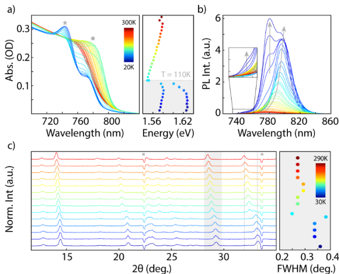
Figure 1: a) Temperature dependent absorption spectra (left) for the 100 nm MAFArub bilayer highlighting the changes to the perovskite onset as the film is cooled from 300 K to 20 K (red to blue). Talc plots (right) for the two phases, denoted by grey octagons and stars, with the phase transition at 110 K included. b) Direct PL spectra for MAFArub bilayer cooling from 300 K to 20 K collected under 405 nm excitation. Three spectra were collected at each temperature then averaged. Spectral inset highlights the growth of the high energy feature at 750 nm. Grey arrows are included as guides to the eye. c) MAFArub XRD patterns (left) collected from 290 K to 30 K. Astrik denotes the instrumental artifacts. Grey dashed lines are included to highlight peak change. Calculated full-width at half max (FWHM) for the (220) plane across the temperature range.
