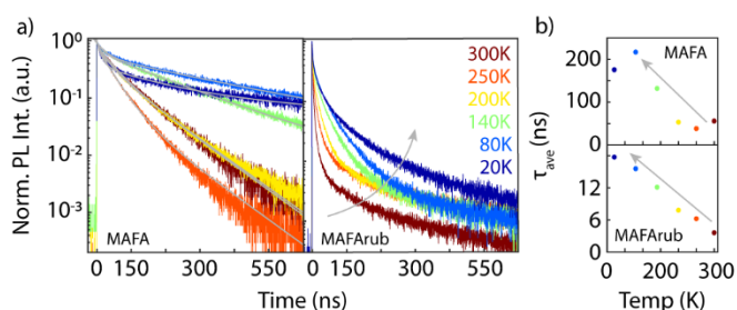
Figure 3: a) Temperature-dependent perovskite PL decays for the neat MAFA film (left) and MAFArub bilayer (right) collected under 635 nm pulsed excitation (125 kHz). Triexponential fits are included as grey lines for the MAFA decays. The grey arrow is included as a guide to the eye for the MAFArub decays. b) Amplitude weighted lifetimes ( \tau_{ave} ) for the MAFA (top) and MAFArub (bottom) films. Grey arrows are included as guides to the eye.
