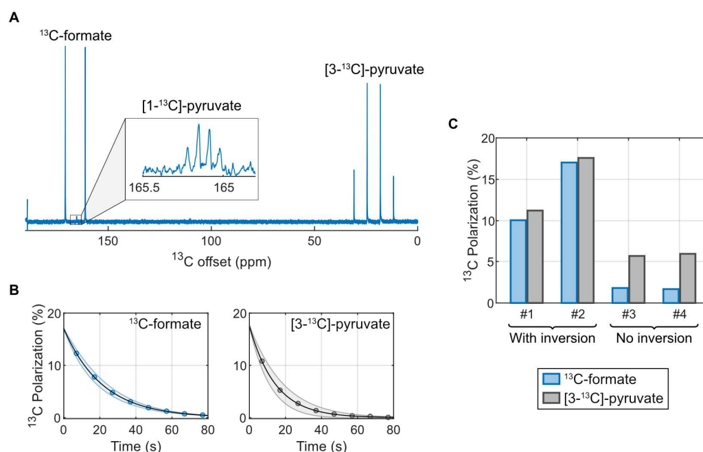
Figure 5: (a) Hyperpolarized ^{13}\text{C} signal after inversion in the liquid state for ^{13}\text{C} -formate and 3-^{13}\text{C} -pyruvate at 1.88 T. The inset shows the weak signal originating from 1-^{13}\text{C} -pyruvate (b) Decays of ^{13}\text{C} polarization monitored with 5^\circ pulses for ^{13}\text{C} -formate and 3-^{13}\text{C} -pyruvate as a function of time after injection in the case where the spin experienced a field inversion during the sample transfer. The colored areas around the fitted curves represent the predicted polarization with 95% confidence. (c) Comparison of the ^{13}\text{C} polarization at the time of injection in the liquid state for the four ^{13}\text{C} -detected experimental runs. See the text for experimental details on the different runs.
