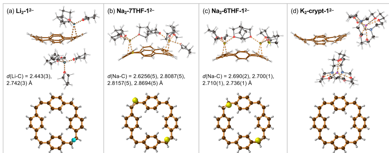
Fig. 2 Single crystal X-ray structures of (a) \text{Li}_2\text{-1}^{2-} , (b) \text{Na}_2\text{-7THF-1}^{2-} , (c) \text{Na}_2\text{-6THF-1}^{2-} and (d) \text{K}_2\text{-crypt-1}^{2-} (thermal ellipsoids: 40% probability). In each case, the lower image is a projection perpendicular to the mean plane of the PCT di-anion, with coordinated metal cations. The shortest metal-carbon distances are indicated by dashed lines and listed. Solvent molecules and minor disorder components are omitted for clarity. Color code: Li: sky-blue; Na: yellow; K: purple; N: blue; O: red; C: black or brown; H: pale gray.
