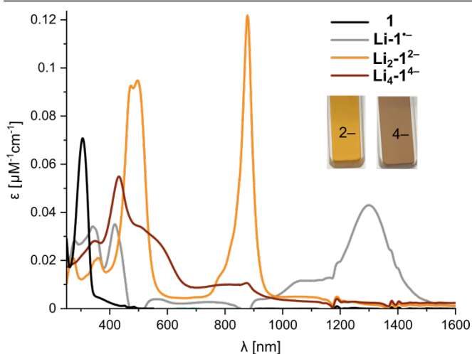
Fig. 6 UV-vis-NIR spectra from in situ reduction of 1 with Li metal in THF at 25\text{ }^{\circ}\text{C} , corresponding to the neutral macrocycle, radical anion, di-anion and tetra-anion (for details, see Fig. S18).
