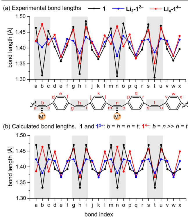
Fig. 3 Comparison of (a) crystallographic C-C bond lengths in 1 , \text{Li}_2\text{-1}^{2-} and \text{Li}_4\text{-1}^{4-} , and (b) calculated bond lengths for gas-phase 1 , \text{1}^{2-} and \text{1}^{4-} from DFT (CAM-B3LYP/def2-TZVP). Bonds in the vinylene bridges are marked in gray. Lengths for the para -phenylene units (e.g. d-f ) are averages for inner and outer bonds.
