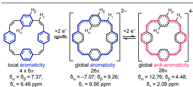
Fig. 1 Reduction of neutral 1 (PCT) to the di- and tetra-anion, showing the number of \pi electrons in the delocalization pathways and 1 H NMR chemical shifts in THF- d 6 , -80 °C (data from ref. 3a).
