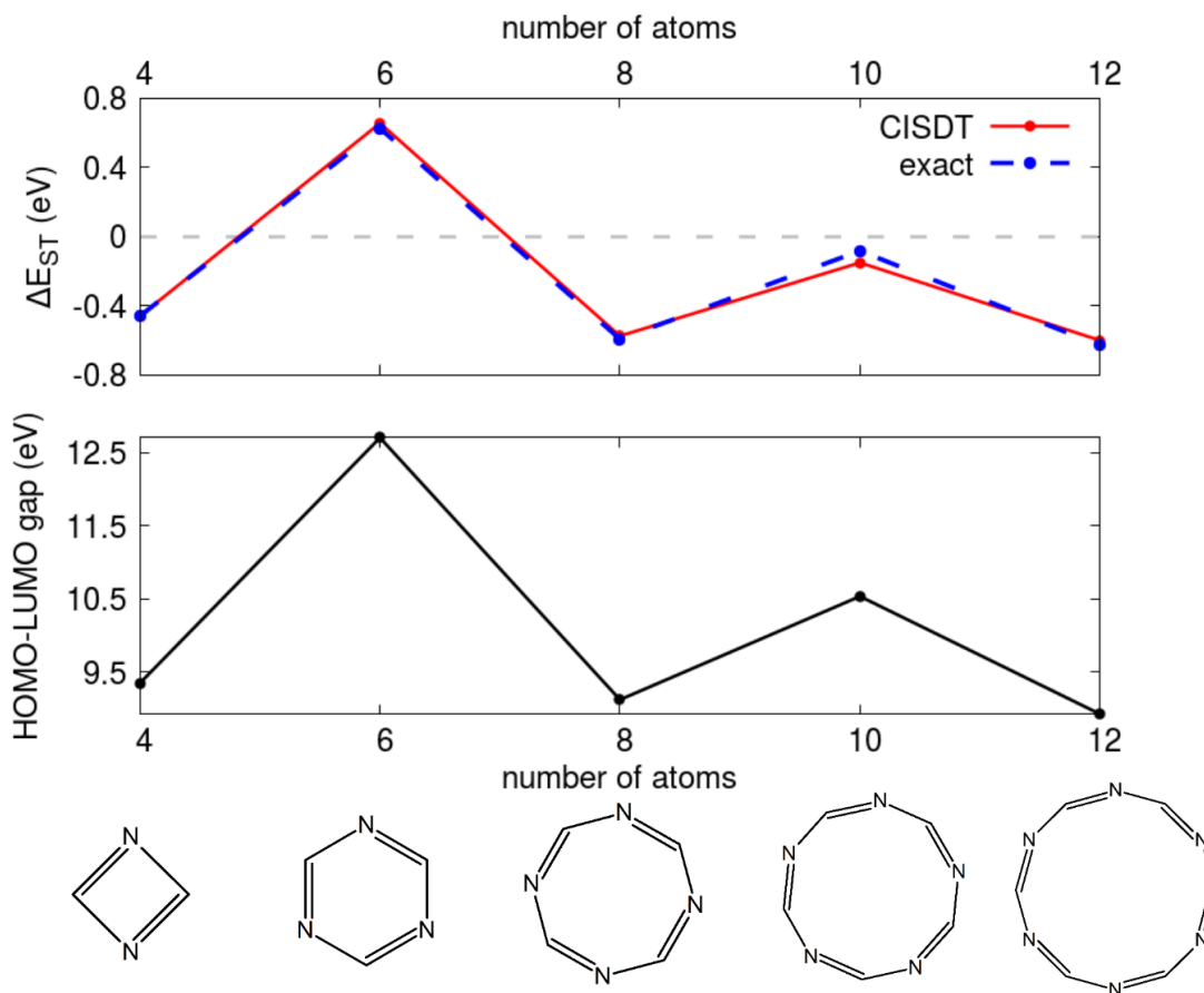
Figure 8: Results for rings with different numbers of aza nitrogen atoms. Upper panel: ST gap values. The red curve refers to PPP CISDT results. Dashed blue line refers to results from exact diagonalization in the RS basis (full-CI). Lower panel: HF HOMO-LUMO gap for the different aza-doped rings. Same parameters used in Fig. 4.
