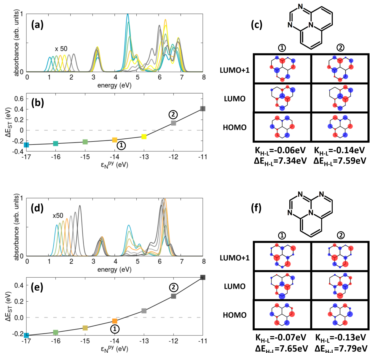
Figure 6: Decorating the 2T-N rim with an increasing number of aza nitrogen atoms while changing the pyrrole nitrogen site energy. Calculated absorption spectra (panels a and d), ST gap (panels b and e) and HF frontier orbitals (panels c and f) are shown for 2T-3N and 2T-4N'. In panels a and d, spectra are normalized with respect to the maximum absorbance of the most intense spectrum, while the band relevant to the first excited singlet state is magnified by 50. In panels c and f, we report the relevant HOMO-LUMO exchange energies, K_{H-L} , and gaps, \Delta E_{H-L} . Calculations done at PPP CISDT level for the same parameters used in Fig. 4.
