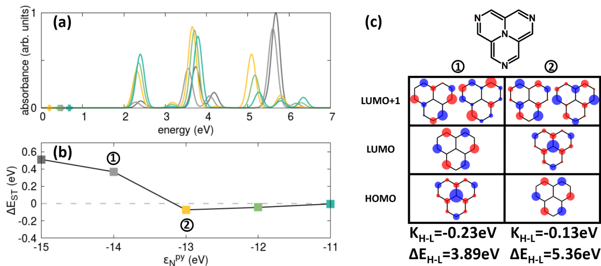
Figure 5: The effect of \epsilon_N^{py} on the energy levels of 2T-4N. Panel a: Absorption spectra calculated for different \epsilon_N^{py} values (same color code used in panel b). The crosses mark the position of the first excited (dark) state. Spectra are normalized with respect to the maximum absorbance of the most intense spectrum. Panel b: Calculated singlet-triplet energy gaps. Panel c: Frontier Hartree-Fock MOs for two different \epsilon_N^{py} values. Relevant HF HOMO-LUMO exchange energy K_{H-L} and energy gaps \Delta E_{H-L} are also reported. Other parameters are defined in the main text. Results obtained at the PPP CISDT level.
