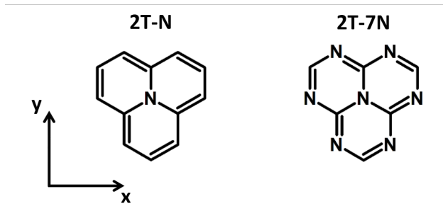
Figure 1: Sketches of the molecular structures of two prototypical triangulenes: 2T-N, also called cyclazine, and 2T-7N, also called heptazine.
