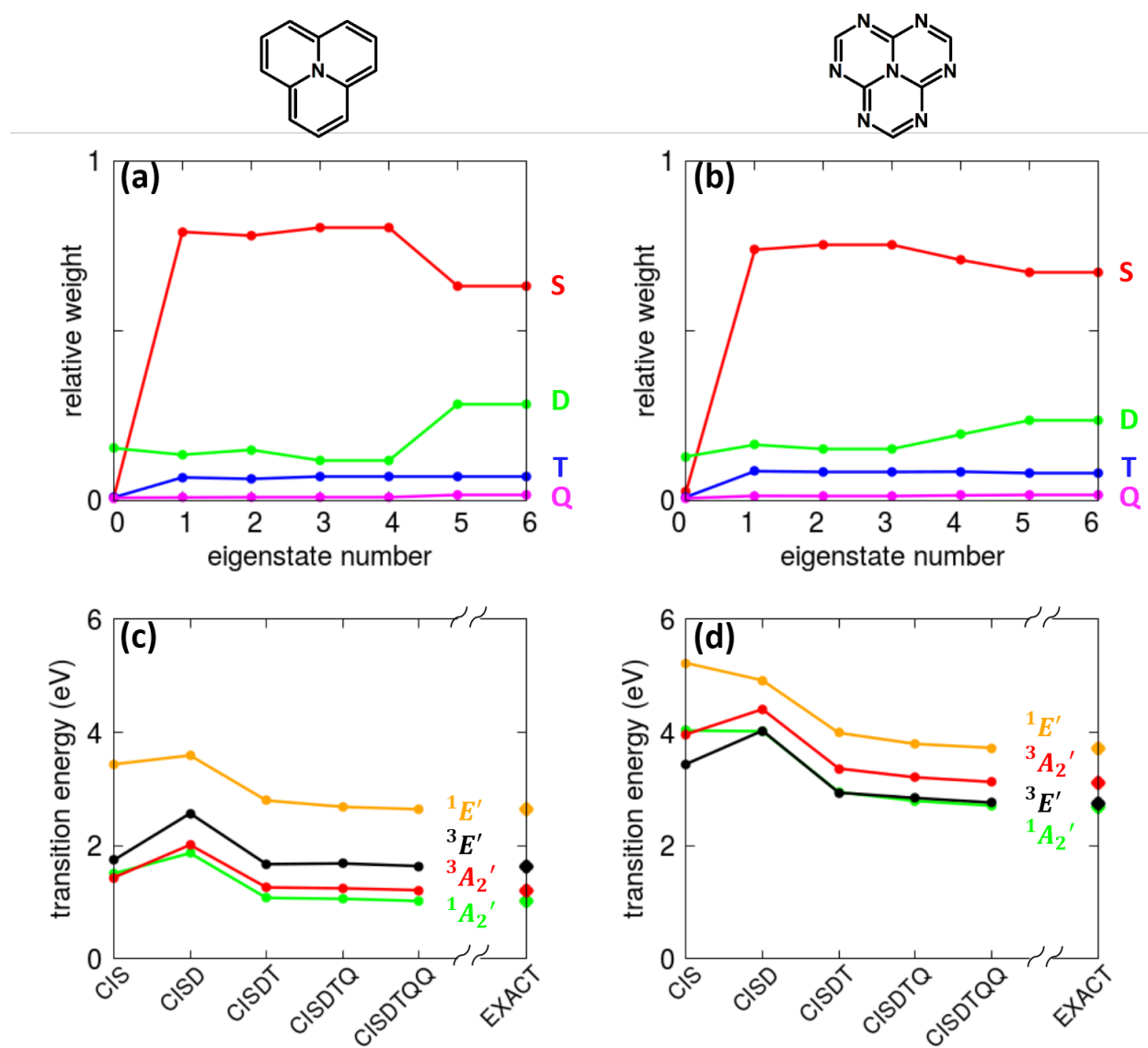
Figure 4: Relative weights of single (S), double (D), triple (T), quadruple (Q) excitations for the first seven singlet and triplet eigenstates of 2T-N (panel a) and 2T-7N (panel b) calculated at the CISDTQ level, together with the excitation energies of the first few electronic states of 2T-N (panel c) and 2T-7N (panel d) at different levels of theory. Relevant results from exact diagonalization in the real space basis (full-CI) are shown as colored dots in panels c and d. Model parameters defined in the main text.
