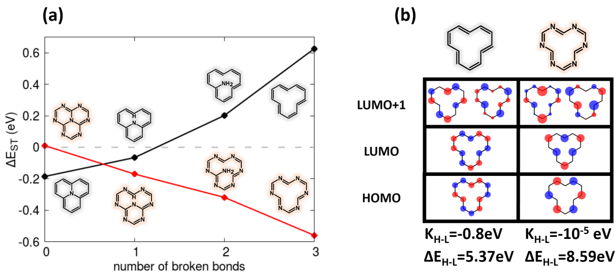
Figure 7: The role of central connectivity on the ST gap. Panel a: Calculated ST gap as a function of the number of broken central bonds for both 2T-N (black curve) and 2T-7N (red curve). Calculations done at the PPP CISDT level. Panel b: Frontier HF MOs are shown for the two annulenes obtained by breaking all three central bonds in 2T-N and 2T-7N. Relevant HOMO-LUMO exchange energies and gaps are also shown. Same model parameters as in Fig. 4.
