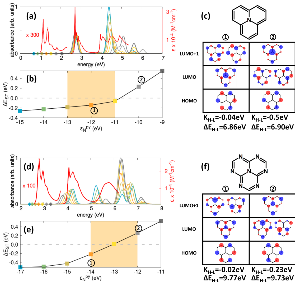
Figure 2: Simulating the photophysics of 2T-N (panels a-c) and 2T-7N (panels d-f). (a) Absorption spectra of 2T-N: red lines are experimental data from Ref., 57 colored lines show results for several \epsilon_N^{py} values (same color code as in panel b), the crosses in the low energy region mark the position of the dark state. Calculated spectra are normalized to the maximum absorbance of the most intense spectrum. (b) 2T-N singlet-triplet energy gaps calculated for different \epsilon_N^{py} values, the shaded area highlights \epsilon_N^{py} values giving acceptable agreement between calculated and experimental absorption spectra. (c) 2T-N frontier HF-MO for two values of \epsilon_N^{py} , the corresponding exchange integral K_{H-L} , and energy gaps, \Delta E_{H-L} . (d) Absorption spectra of 2T-7N: red lines are experimental data from Ref., 58 colored lines show results for several \epsilon_N^{py} values (same color code as in panel e), the crosses in the low energy region mark the position of the dark state. Calculated spectra are normalized to the maximum absorbance of the most intense spectrum. (e) The same as (b) for 2T-7N. (f) The same as (c) for 2T-7N.
