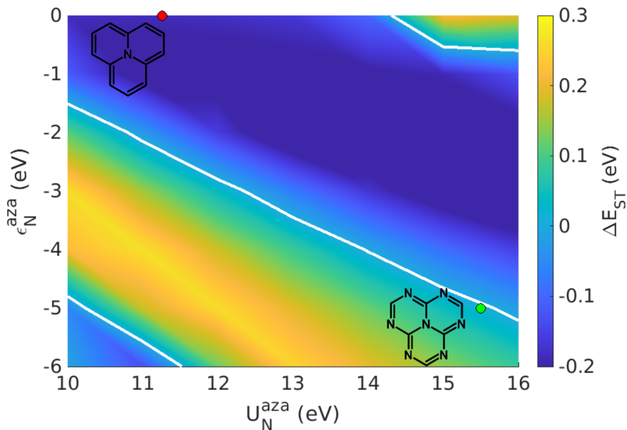
Figure 3: The color map shows the dependence of the ST gap (color code on the right) as a function of \epsilon_N^{aza} and U_N^{aza} , having set \epsilon_N^{py} = -13 eV. White lines at \Delta E_{ST} = 0 mark the boundary between the ST inverted region (dark blue) and the normal region (light blue and yellow). Red and green dots indicate the parameters relevant to 2T-N and 2T-7N, respectively. Calculation done at the PPP CISDT level with model parameters defined in the main text.
