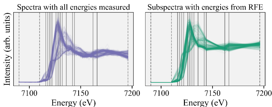
Figure 4 Fully measured experimental XANES spectra (left) compared to the reduced energy point subspectra (right), with energies recommended by the RFE algorithm (vertical gray lines). The dashed lines indicate energies we subsequently added for normalization purposes.
