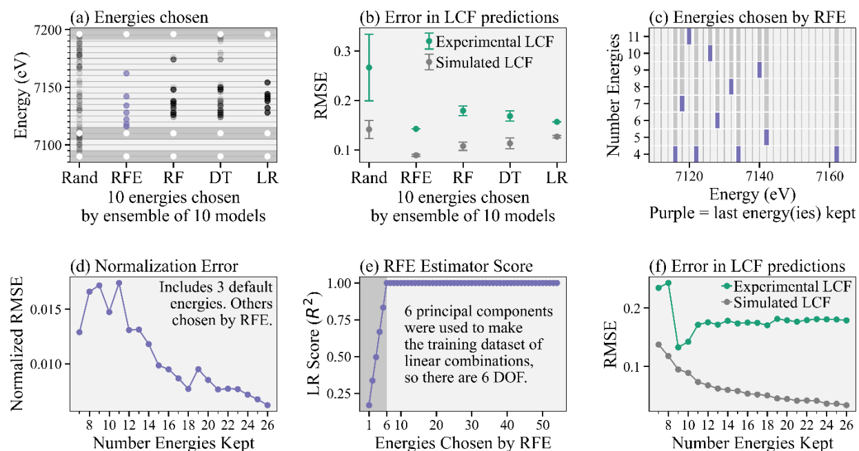
Figure 3 Characterization and validation of RFE algorithm. (a) Collection of energies chosen by different feature selection algorithms: random selection (Rand), recursive feature elimination (RFE), random forest (RF), decision tree (DT), and linear regression (LR). The dark bars include the three default energies (white) to ensure normalization. (b) Corresponding errors in LCF predictions on both a generated test dataset and the experimental spectra for all models. (c) Energies consecutively removed by the RFE as fewer energy points are kept, which shows consistency in training. The last energy, or set of energies, kept by the RFE are denoted in purple. (d) Error in reconstructing spectra using normalization parameters from reduced energy point subspectra of different sizes compared to normalized full energy spectra. (e) R^2 score of the linear regression (LR) base estimator in the RFE. (f) Error in LCF predictions versus subspectra size on both simulated test data and the experimental spectra.
