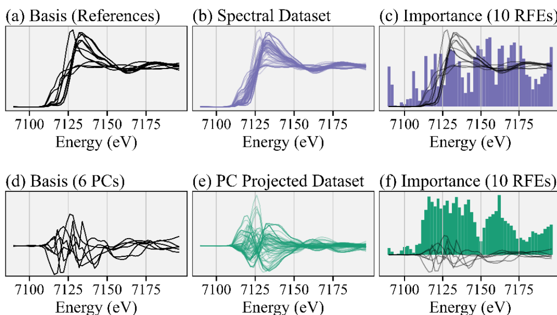
Figure 2 Comparing RFE results on the full reference library versus using forced linear independence in the basis set and thus the training dataset. (a) The spectral reference library. (b) Training dataset of linear combinations of references. (c) The RFE results, trained on the spectral linear combinations. The black basis vectors are the same as in Fig. 2a. (reference spectra). (d) Spectra are instead represented using a basis set comprised of the first six principal components (PCs) to force linear independence. Thus, the linear combination solutions are unique. (e) The
