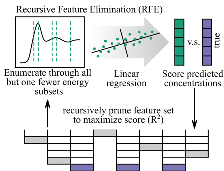
Figure 1 Recursive Feature Elimination (RFE) optimizes the feature subset to measure, in this case energies, by training a base machine learning model – such as linear regression – to predict target variables from spectra.
