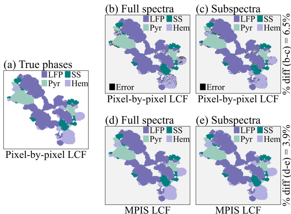
Figure 5 Linear Combination Fitting (LCF) results via standard pixel-by-pixel analysis and Manifold Projection Image Segmentation (MPIS). (a) The “true” results, using the full energy spectra via pixel-by-pixel NNLS-LCF onto the four known reference phases. (b) Pixel-by-pixel NNLS-LCF applied to the full energy spectra; black dots in this panel and later in the figure indicate erroneous inference by the analysis. (c) Pixel-by-pixel NNLS-LCF applied to the reduced energy point subspectra. (d) LASSO-LCF via MPIS applied to the full energy spectra. (e) LASSO-LCF via MPIS applied to the reduced energy point subspectra.
