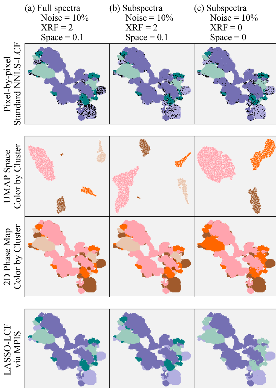
Figure 6 MPIS and LASSO-LCF results using (a) the full spectra and multimodal encoding, (b) the subspectra and multimodal encoding, and (c) the subspectra by themselves without augmented information. Here, the total XRF intensity of sulfur, phosphorus, and chromium and the spatial location of pixels are multimodal information.
