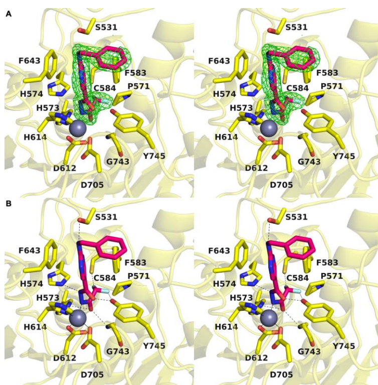
Figure 2. A: Stereoview of the Polder omit map of 13 contoured at 3\sigma (PDB 8GD4). B: Stereoview highlighting intermolecular interactions in the enzyme-inhibitor complex in the active site of HDAC6. The catalytic zinc ion is shown as a gray sphere; metal coordination
