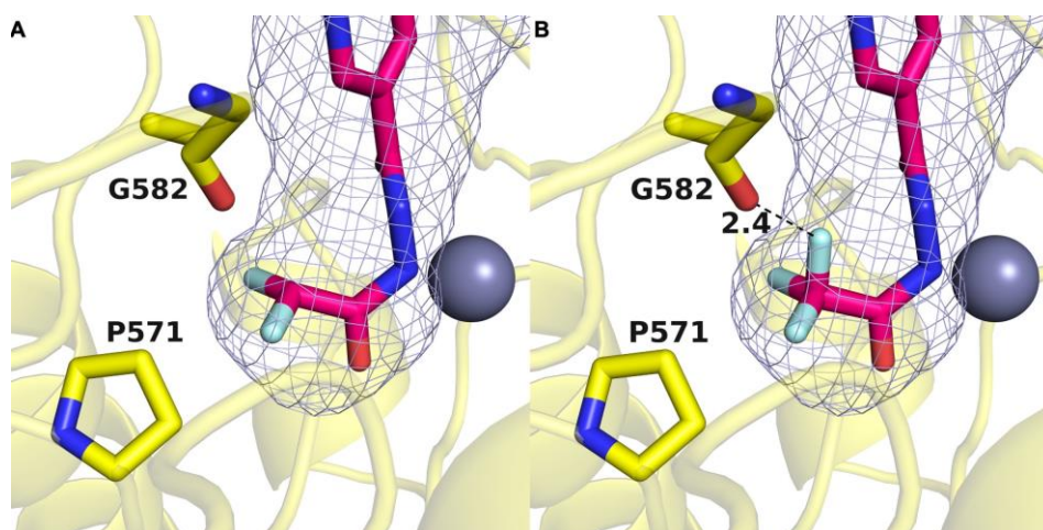
Figure 6. A: Binding pocket of HDAC6 in purple mesh generated by GetCleft showing the orientation of the difluoromethyl group determined in the crystal structure of the complex with 13 (PDB 8GD4). B: Substitution of the CHF 2 group with a CF 3 group yields a model of the complex with hydrolyzed 17 in the ring-opened form. The additional fluorine atom results in a clash with the backbone carbonyl of G582.
