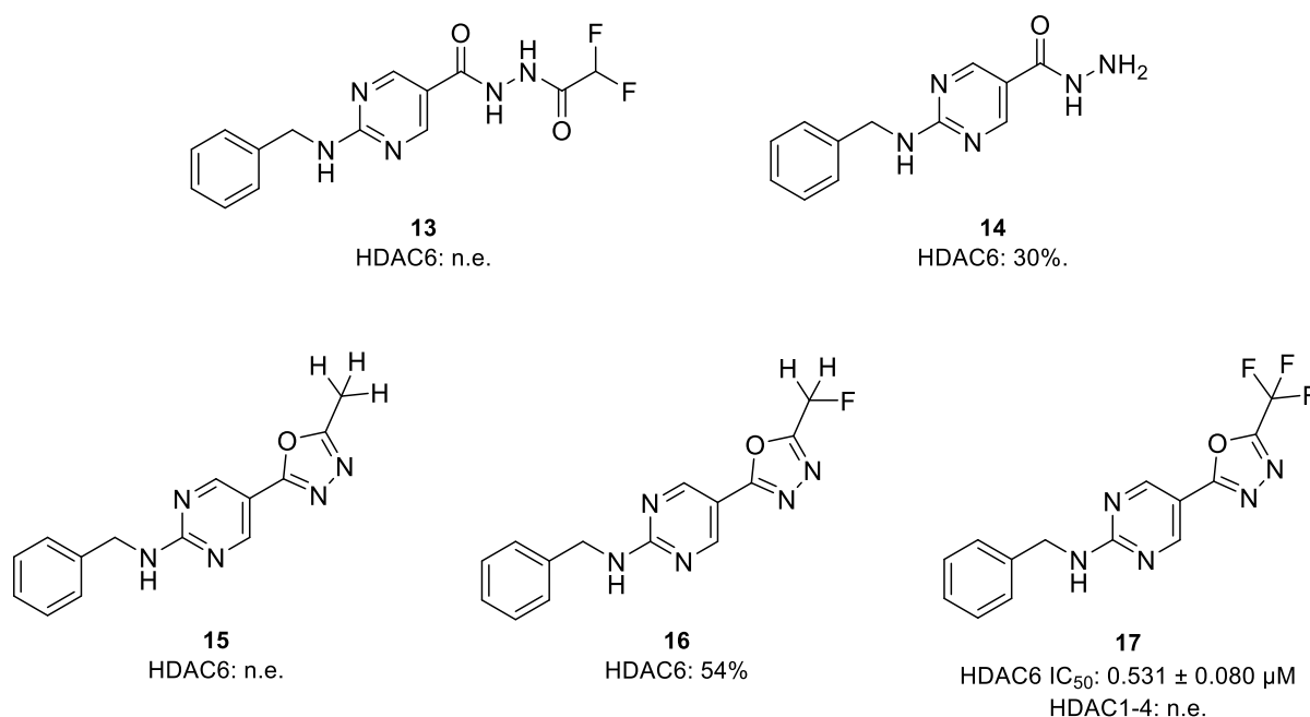
Figure 4. Structures of the acylhydrazide ( 13 ), hydrazide ( 14 ), methyl-1,3,4-oxadiazole ( 15 ), monofluoromethyl-1,3,4-oxadiazole ( 16 ) and trifluoromethyl-1,3,4-oxadiazole ( 17 ) analogs. Inhibitory activities of prepared compounds against HDAC1-4 and HDAC6; IC 50 [μM, mean ± SD] or percent inhibition at 10 μM; n.e.: no effect = < 15% inhibition at 10 μM.
