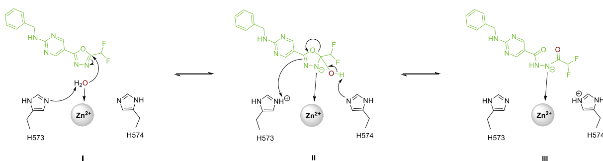
Figure 7. Proposed reaction mechanism of \text{Zn}^{2+} catalyzed ring opening reaction of DFMO compound 6 .
