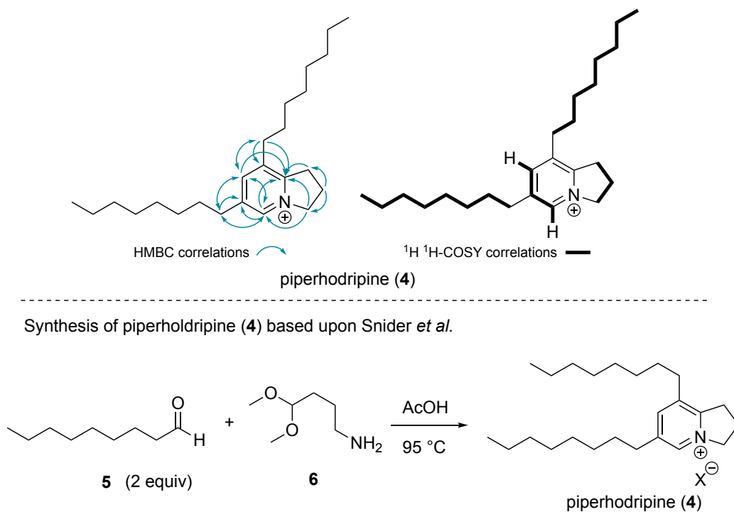
Figure 3. Key 2D NMR correlations and confirmatory synthesis leading to the structure determination of piperholdripine (4)
