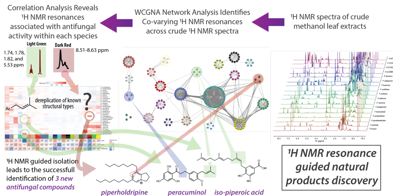
Figure 1. Summary of workflow for the 1 H NMR guided isolation of bioactive natural products
