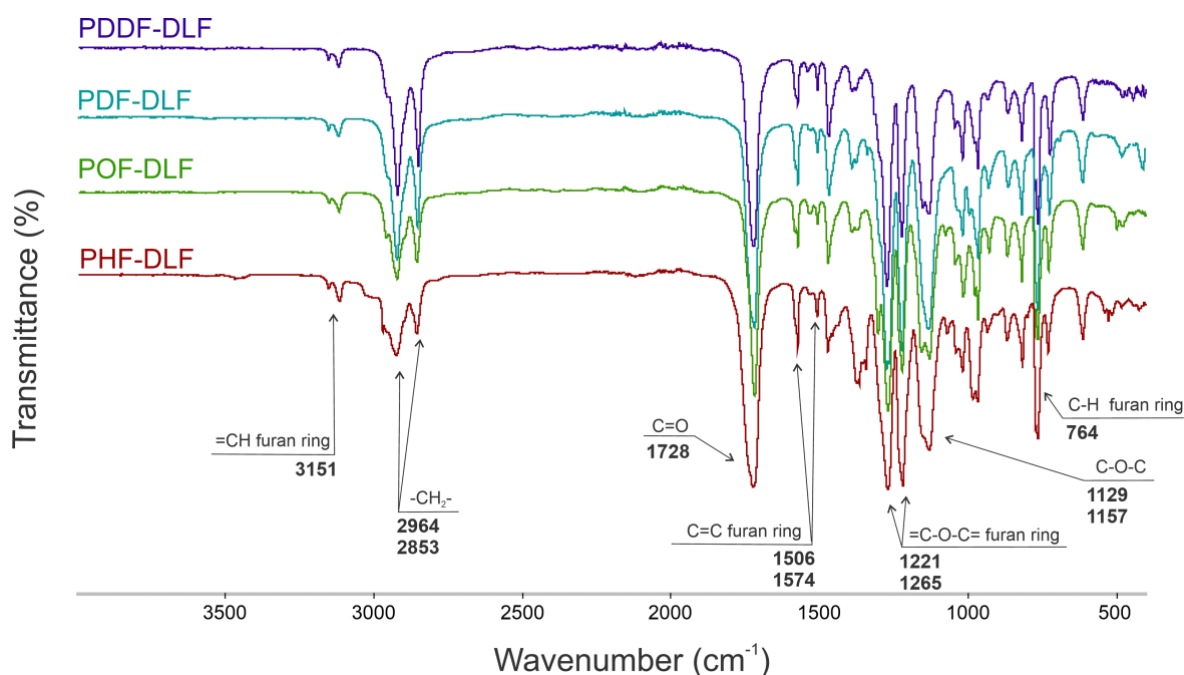
Figure 3. FTIR spectra of furan-based copolyesters.
