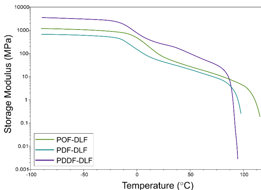
Figure 9. The dependence of storage modulus on temperature for furan-based copolymers.
