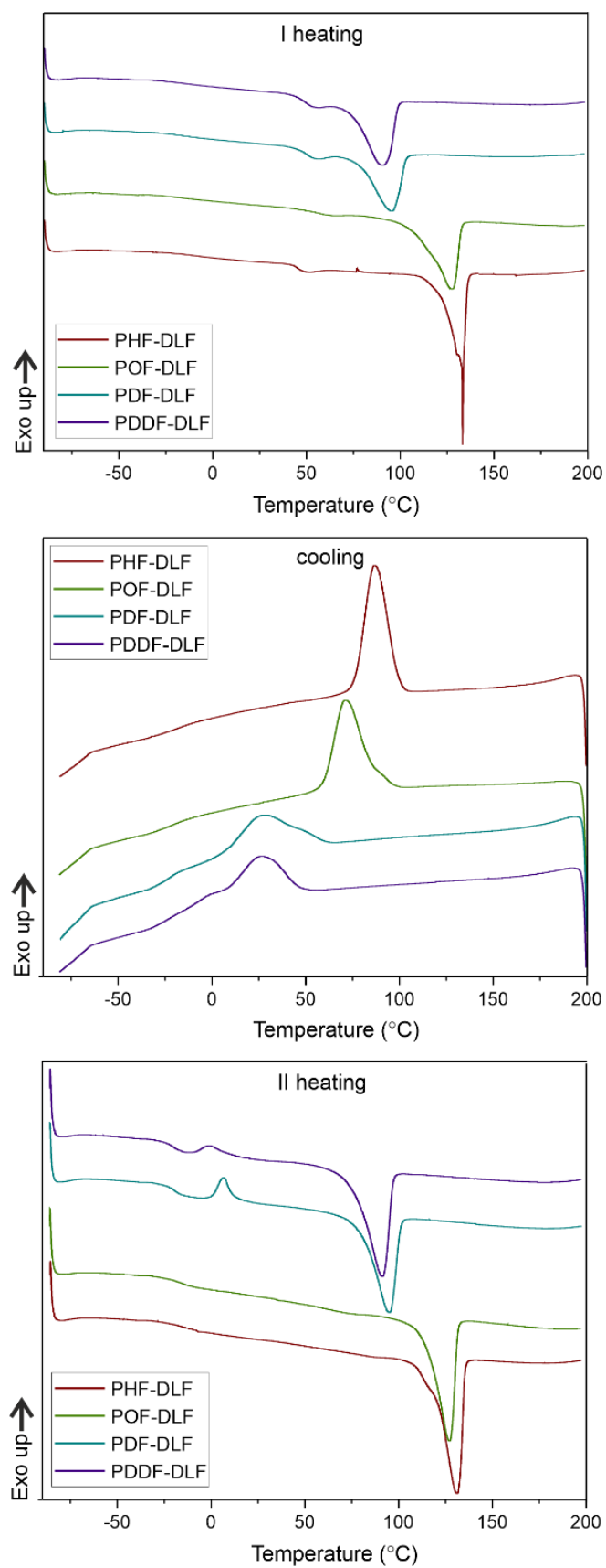
Figure 7. DSC first heating, cooling, and second heating thermograms of furan-based copolymer series.
