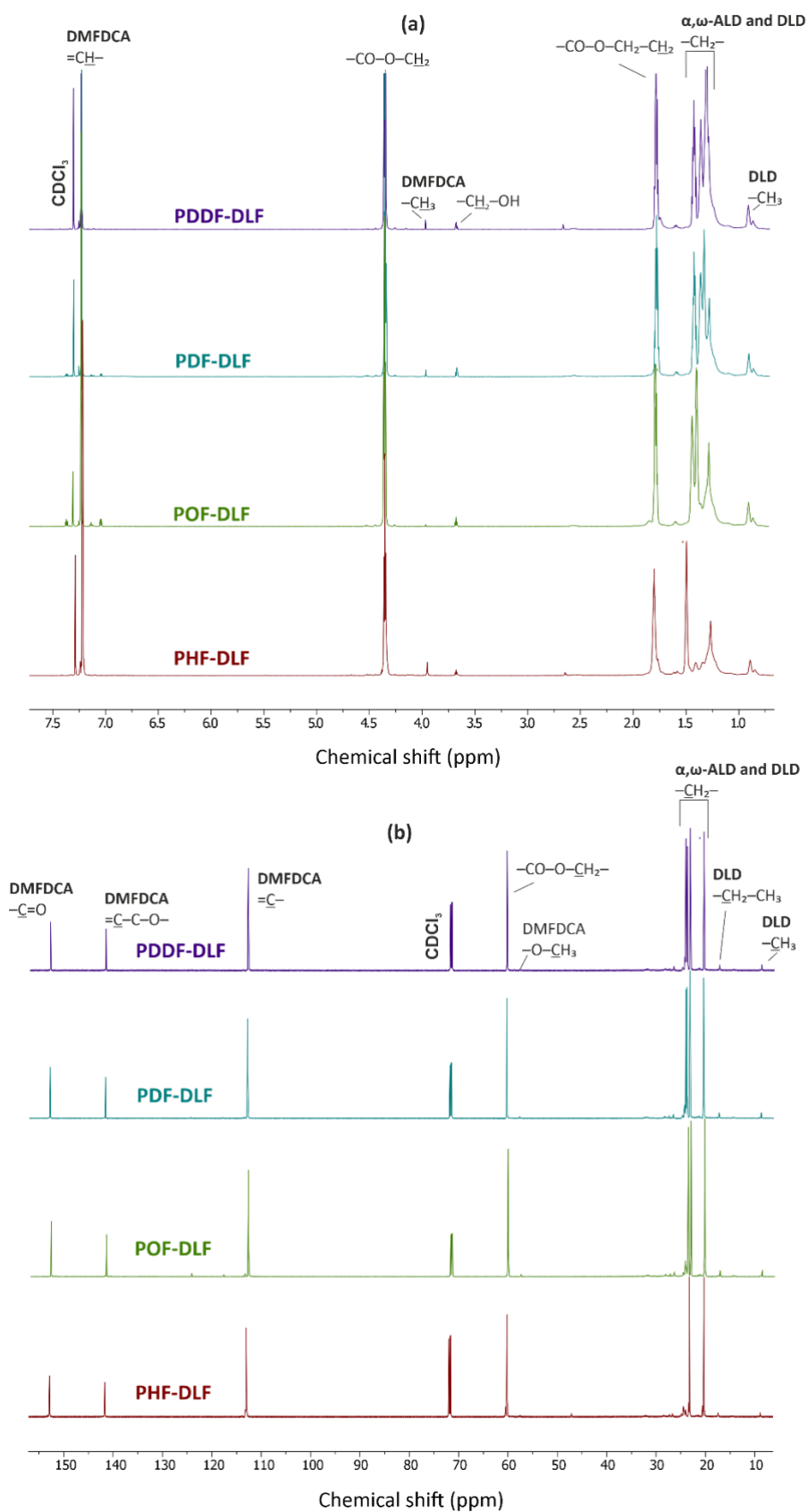
Figure 2. (a) 1 H NMR and (b) 13 C NMR spectra of the furan-based copolyesters.
