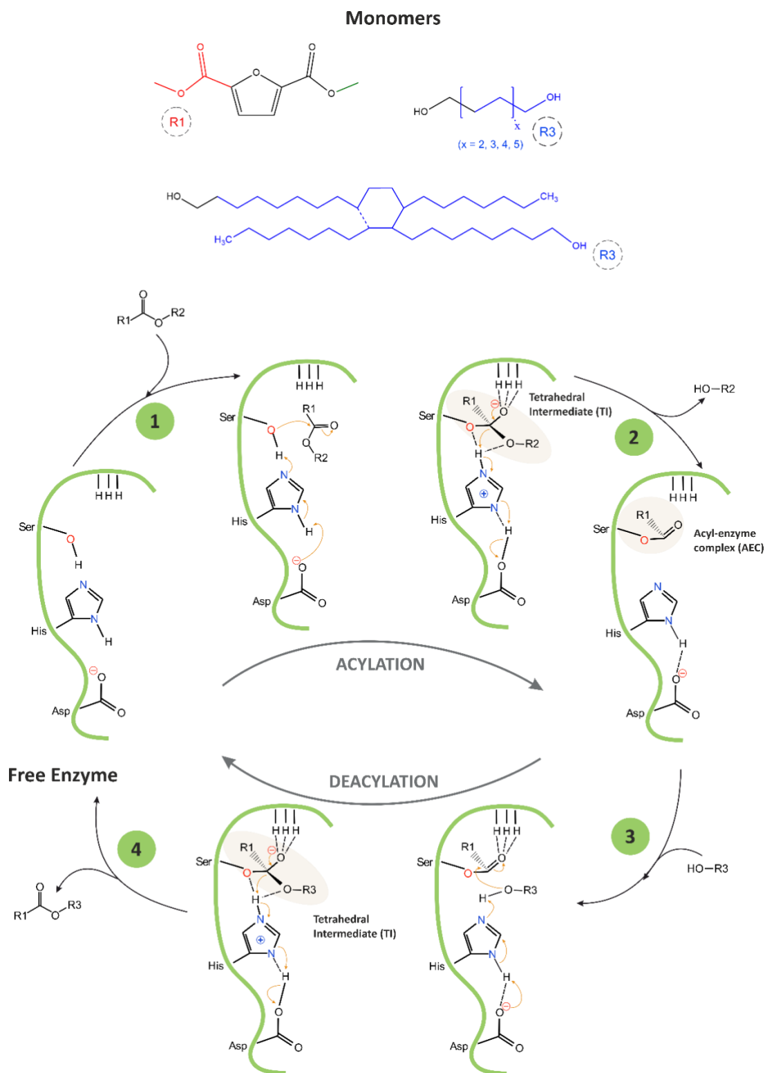
Scheme 2. Proposed mechanism of CAL-B-catalyzed transesterification of DMFDCA with \alpha,\omega -ALD, and DLD.
