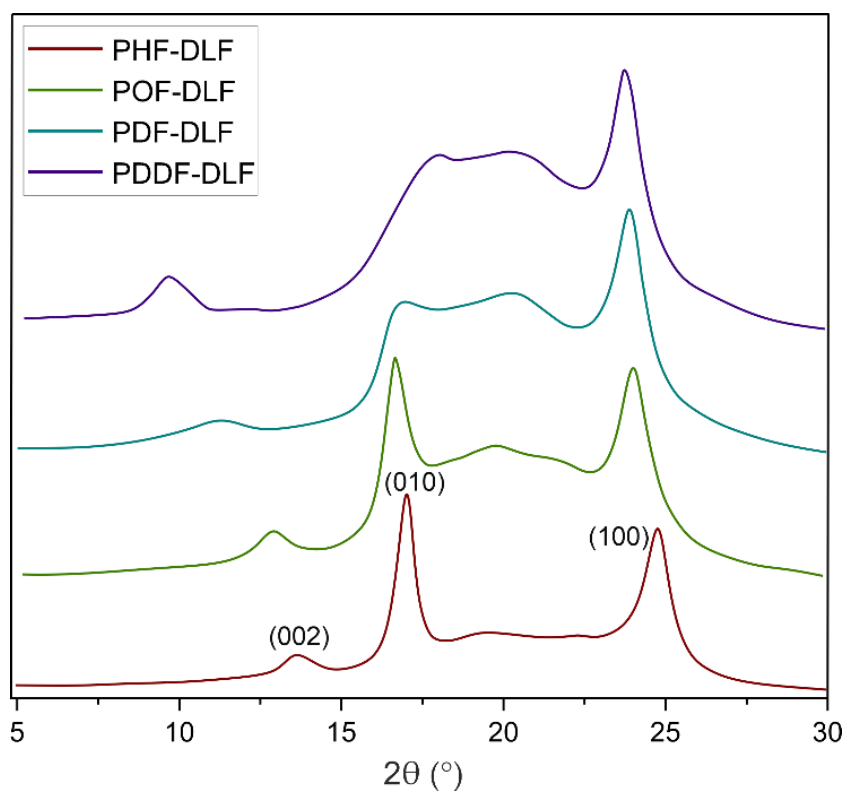
Figure 4. XRD spectra of furan-based copolyesters
