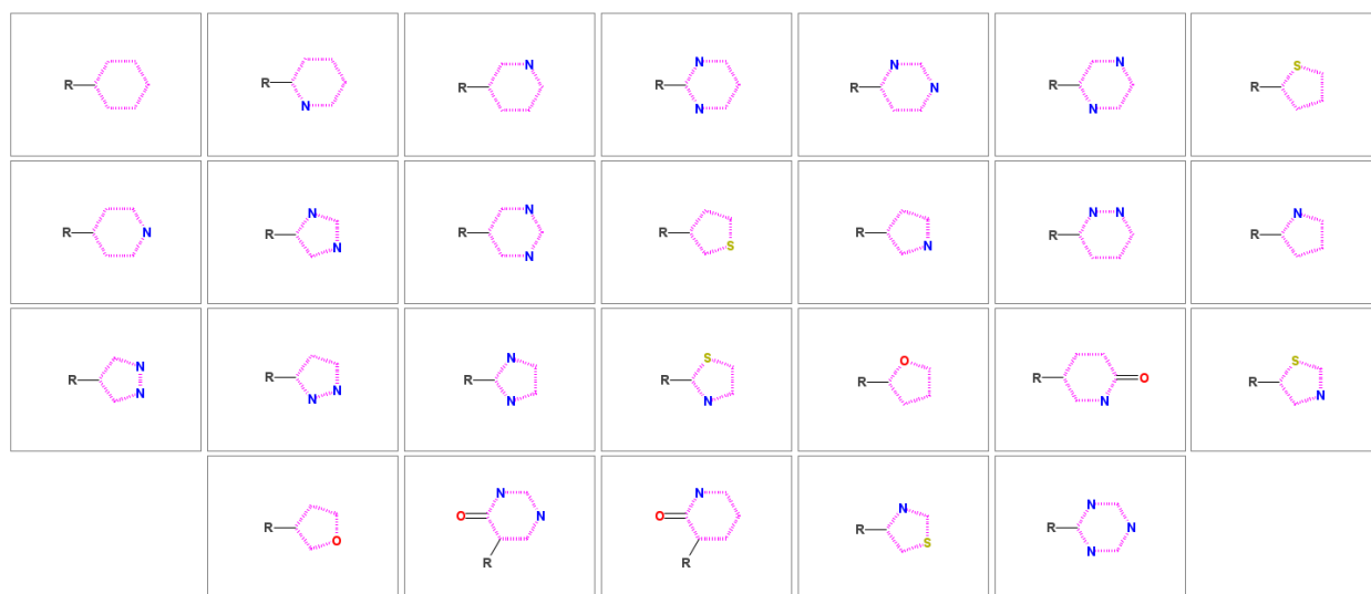
Figure 1. The rings that are used most frequently as substrates reacting with boronic acids in Suzuki-Miyaura coupling. The R represents chlorine or bromine atom, the dashed bonds indicate an aromatic system.
