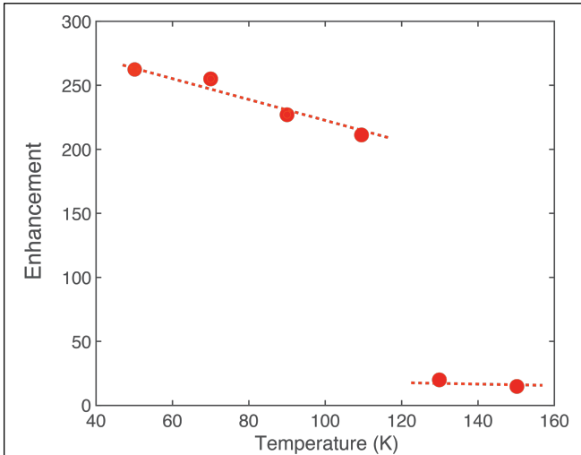
FIG. 5: Temperature dependence of the DNP enhancement of the optimized ASE for sample (2) 20 mM trityl-OX063 in glycerol- d_8 :D 2 O:H 2 O = 6:3:1.
