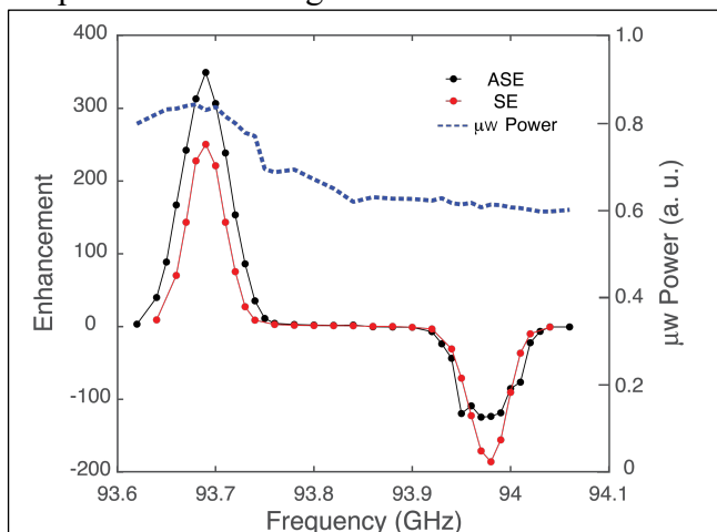
FIG. 1: Field profile of the DNP enhancement comparing ASE and SE for sample (1) 10 mM trityl-OX063 in the d_8 -glycerol: D_2O : H_2O = 6:3:1. The DNP enhanced NMR signals were measured after 150 s of DNP using 12 \mu\text{s} microwave pulses with a repetition delay of 1.2 ms. For the ASE experiment, a 40 MHz frequency chirp was applied, while for the SE no chirping was employed. The dashed line shows the frequency dependence of the microwave power profile (arbitrary units) produced by the EIK and at 93.7 GHz is \sim 250 W.
