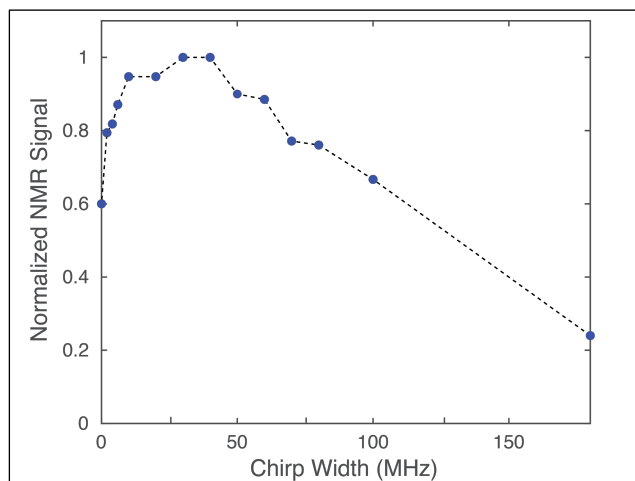
FIG. 2: Normalized NMR signal intensity of sample (1) 10 mM trityl-OX063 in the d_8 -glycerol: D_2O : H_2O = 6:3:1 enhanced by ASE with different chirp widths. All the sequences were with the same 12 \mu\text{s} pulse length. With no chirping, the left most point is the SE, while the right most point becomes the SSE.
